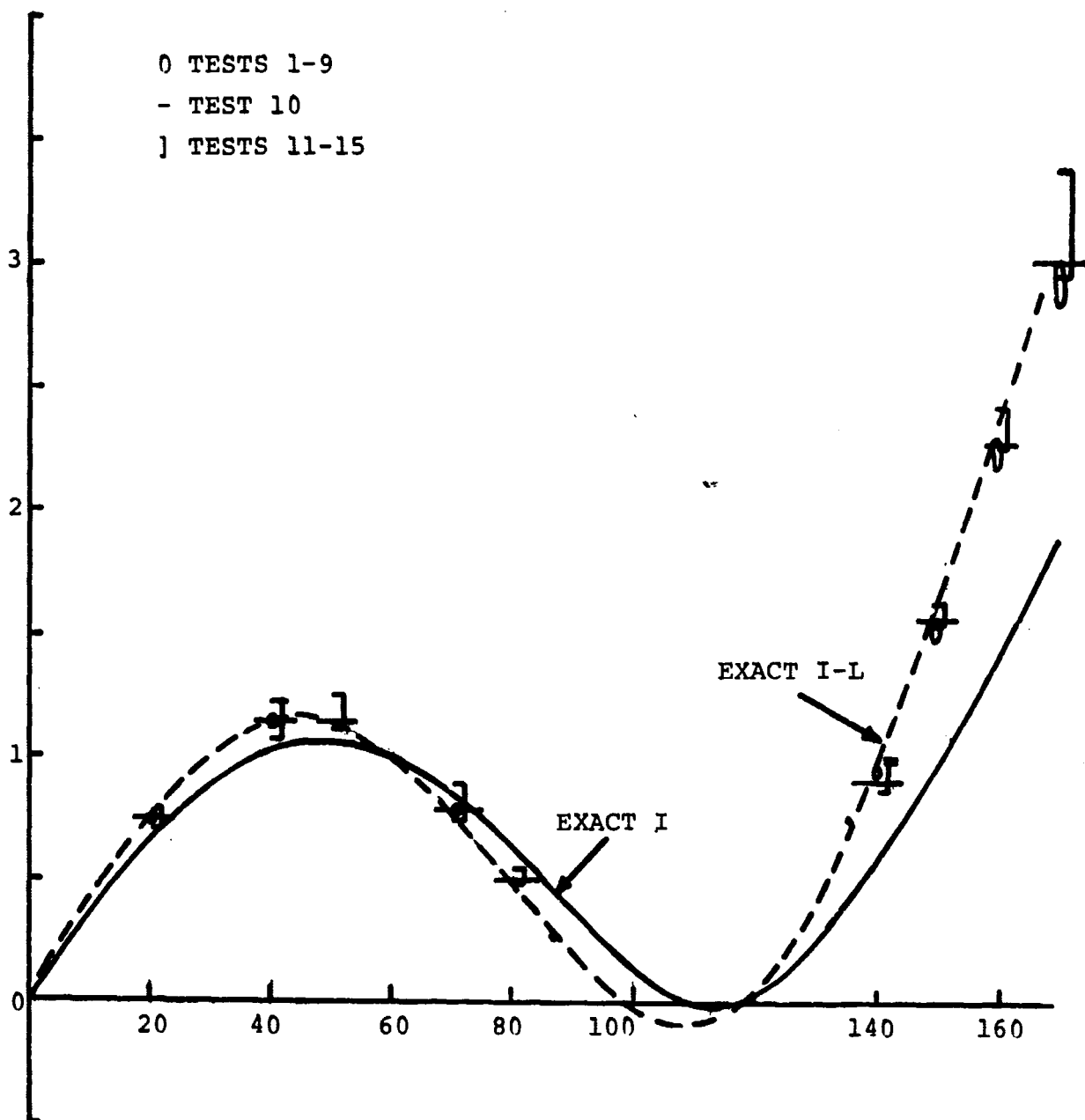
Figure 5b. Computed Mode Changes Due to Stiffness Change Second Mode, Specimen I, Change L.
