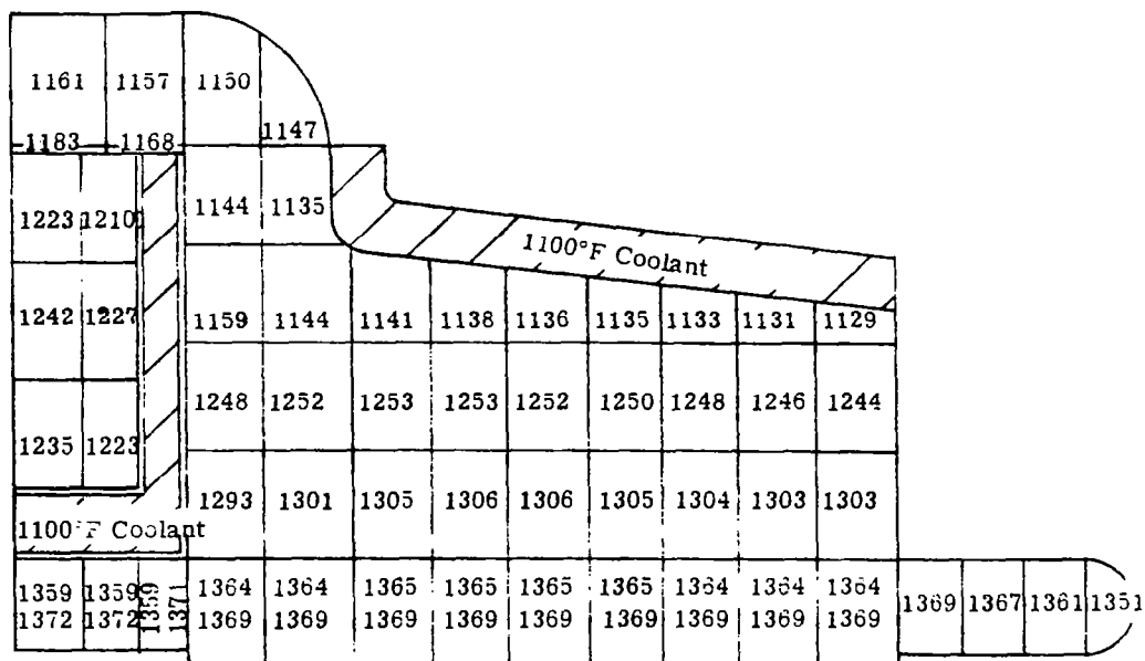
STATOR COOLING SCREENING STUDY, TEMPERATURE DISTRIBUTION (°F) MANIFOLD AND FIELD COIL COOLING WITH AC WINDING COOLING FINS, 1100°F COOLANT, END TURN RADIATION
