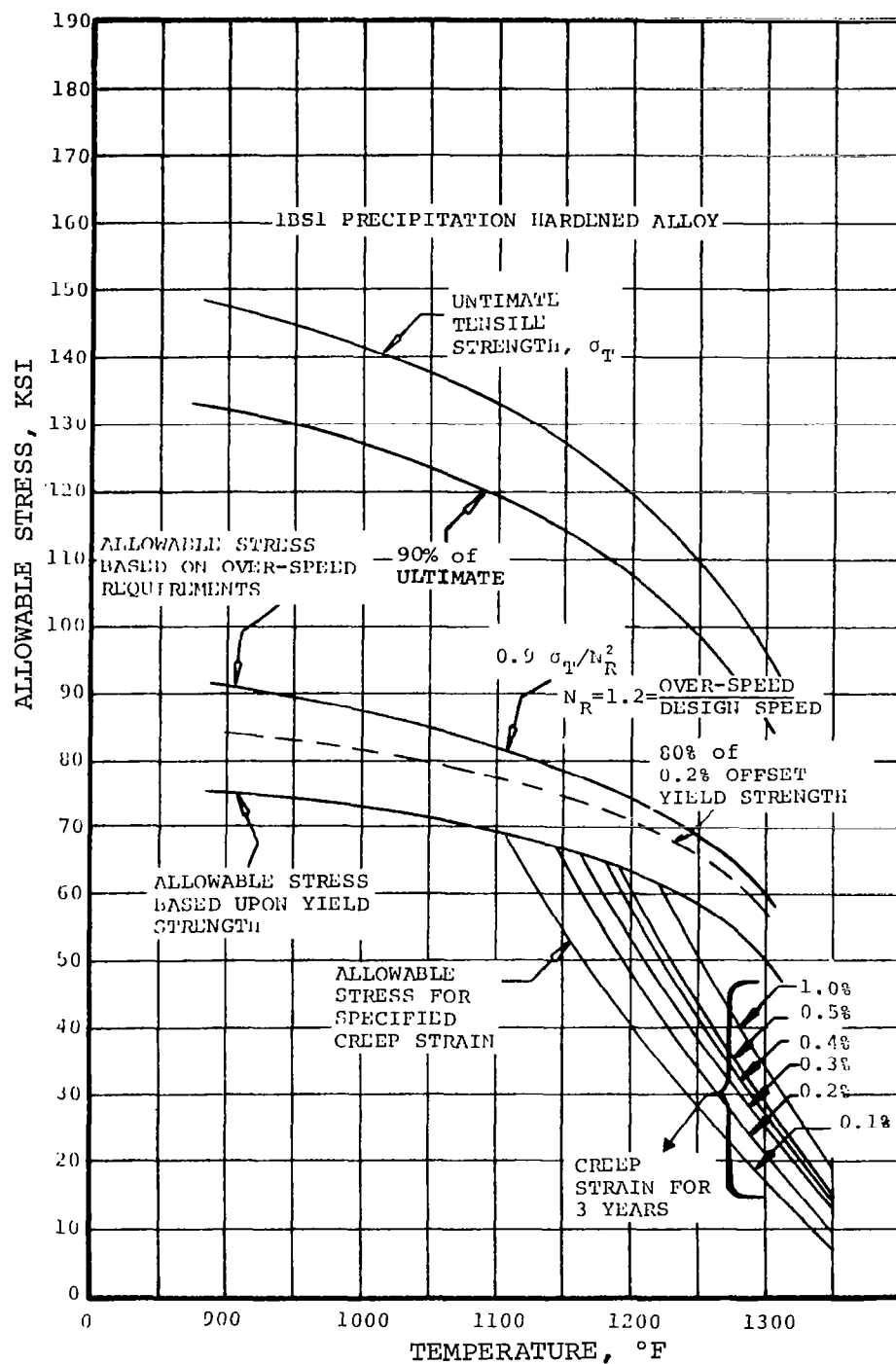
INTERPRETATION OF 1BS1 PRECIPITATION-HARDENED ALLOY PROPERTY DATA
