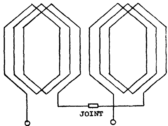
60 DEGREE PHASE BELTS
