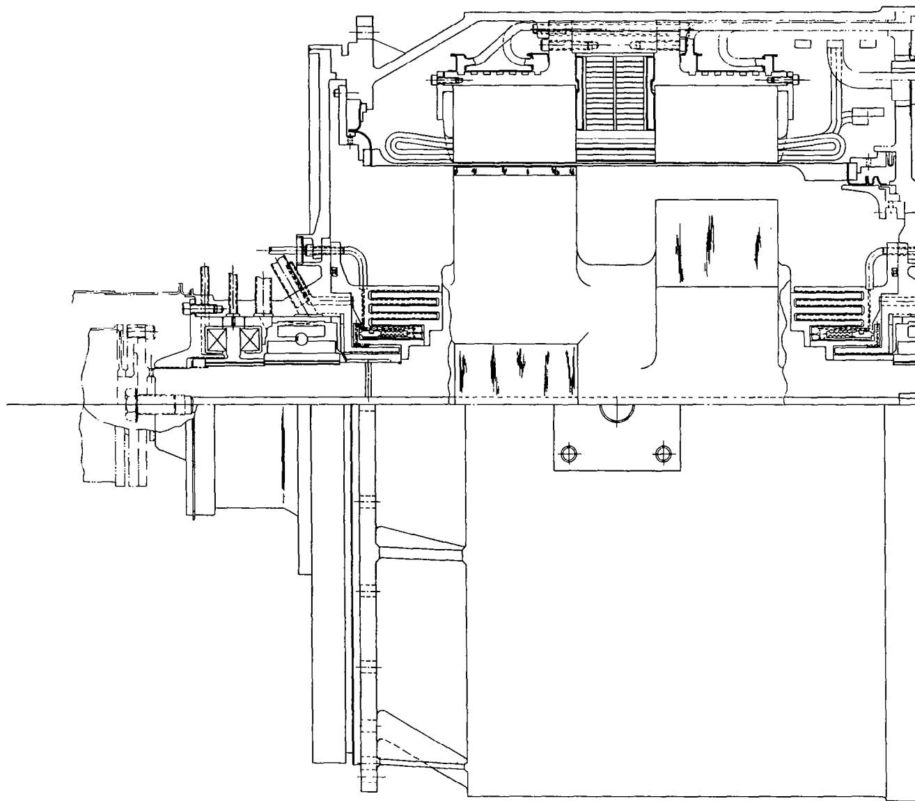
CONCEPTUAL DESIGN LAYOUT, 24,000 RPM, 800°F COOLANT
