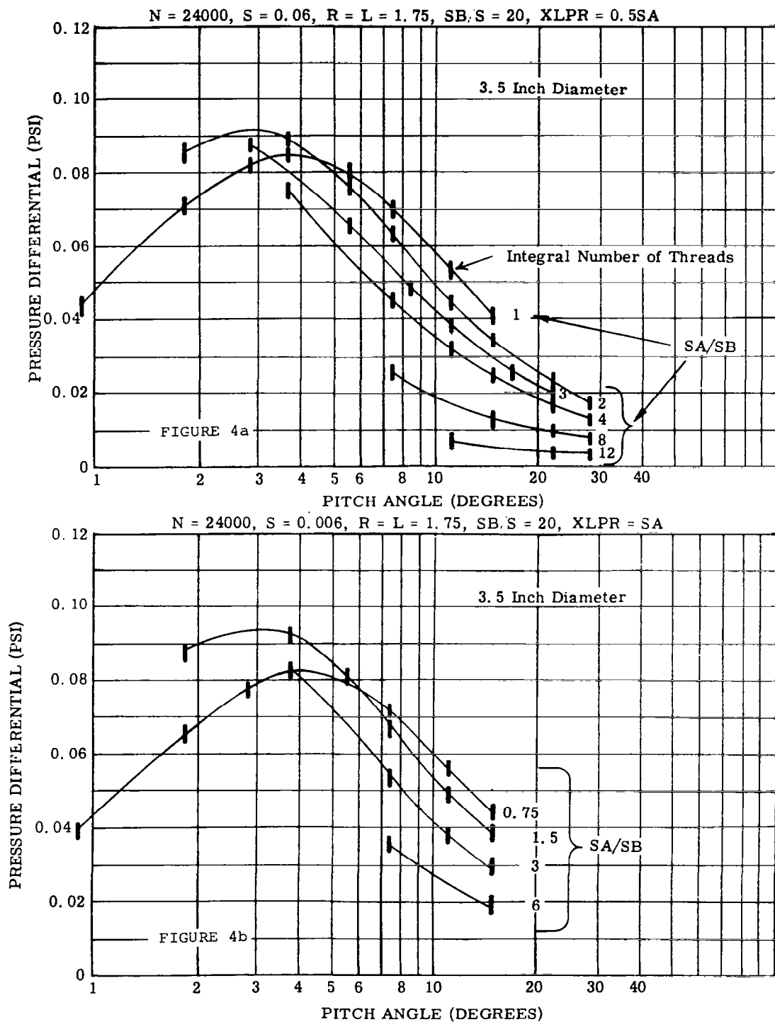
HOLWECK PUMP PARAMETRIC DATA, EFFECT OF PITCH ANGLE, 3.5 IN. DIA
