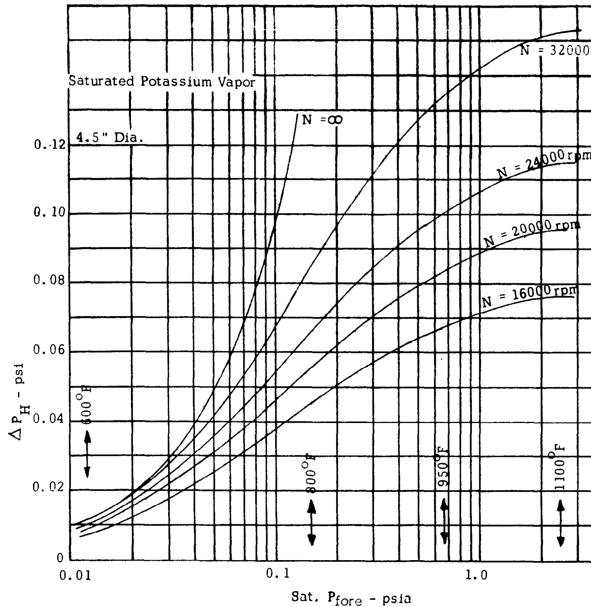
HOLWECK PUMP VAPOR SEAL TYPICAL PERFORMANCE
