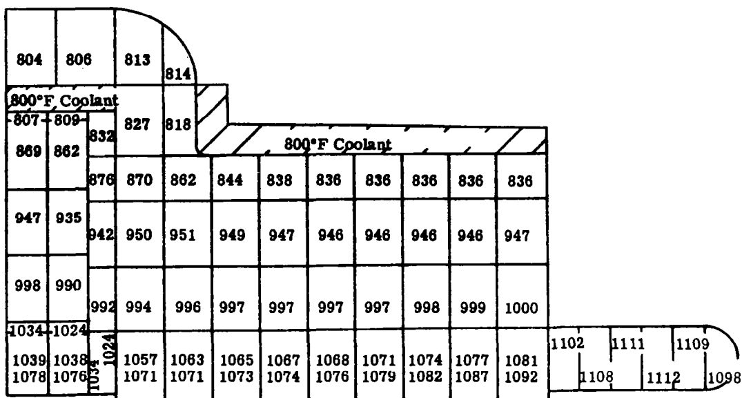
NUMBER 1 DESIGN STATOR TEMPERATURE DISTRIBUTION (°F) 550-KW E RATING, 0.1 W/IN. 2 °C SLOT CONDUCTANCE
