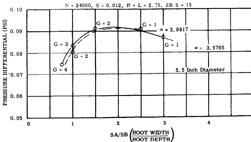
HOLWECK PUMP PERFORMANCE DATA, EFFECT OF SA/SB, 5.5 IN. DIA
