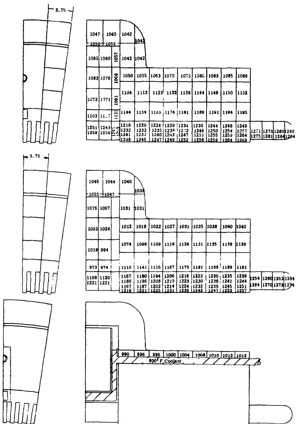
STATOR COOLING SCREENING STUDY, TEMPERATURE DISTRIBUTION (°F) COOLING TUBES EVERY 15 DEG, 800°F COOLANT, END TURN RADIATION
