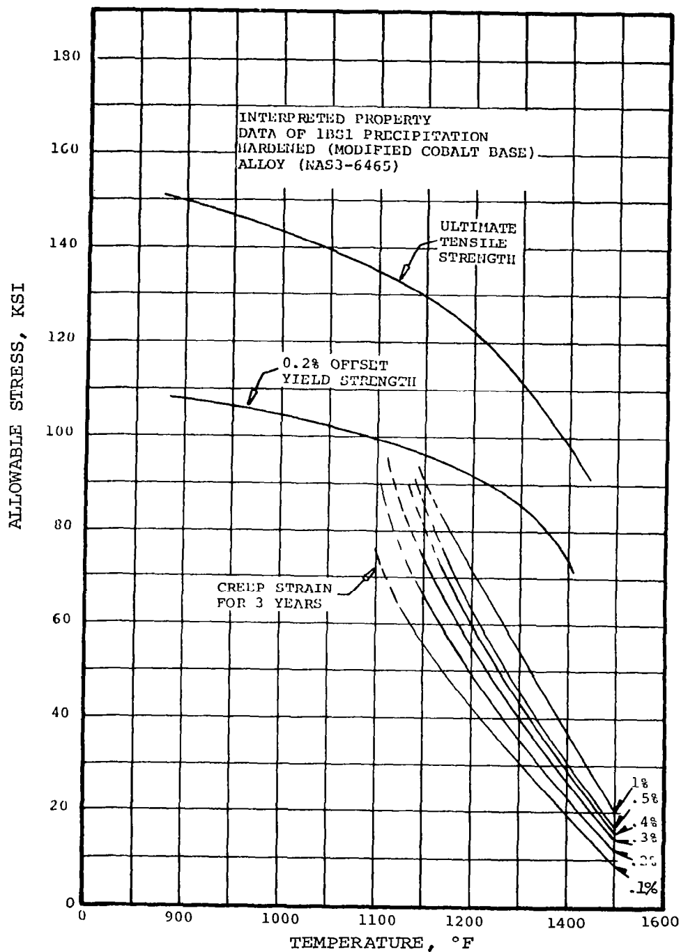
INTERPRETATION OF 1BS1 PRECIPITATION-HARDENED ALLOY PROPERTY DATA
