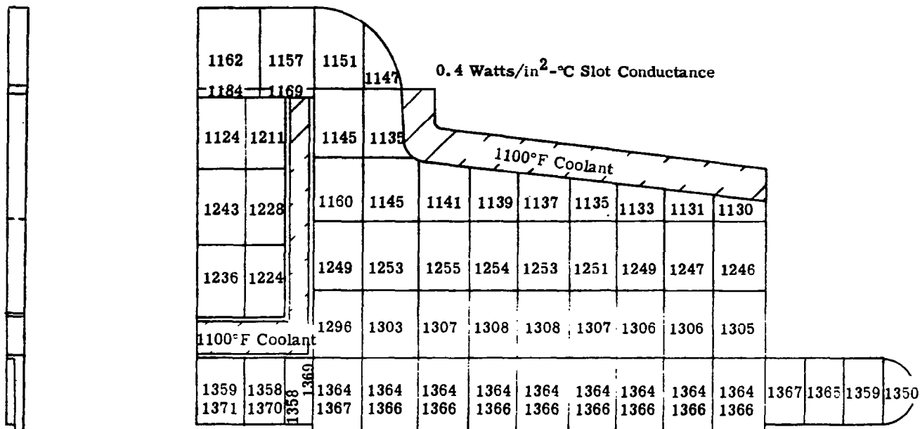
STATOR COOLING SCREENING STUDY, TEMPERATURE DISTRIBUTION (°F) MANIFOLD AND FIELD COIL COOLING WITH AC WINDING COOLING FINS, 1100°F COOLANT, END TURN RADIATION -0.4 W/IN. 2 °C SLOT CONDUCTANCE
