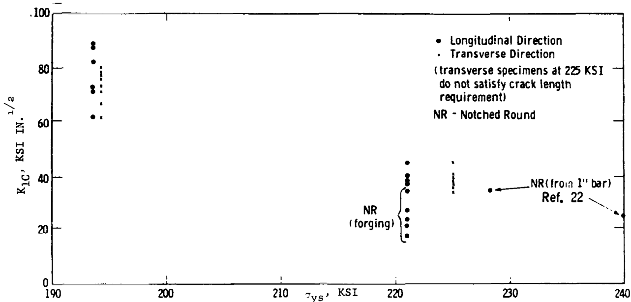
H-11 FRACTURE TOUGHNESS VERSUS YIELD STRENGTH
