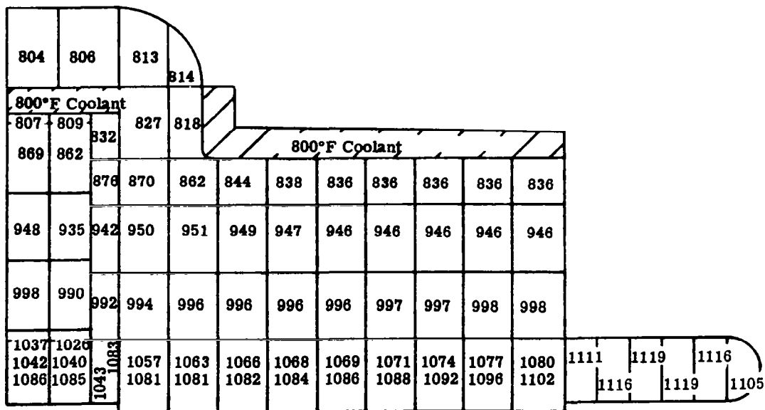
NUMBER 1 DESIGN STATOR TEMPERATURE DISTRIBUTION (°F) 550-KW E RATING, 0.05 W/IN. 2 °C SLOT CONDUCTANCE
