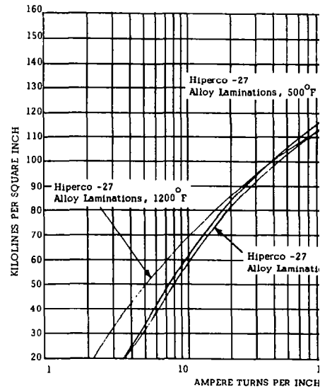
TYPICAL MAGNETIZATION CURVES
