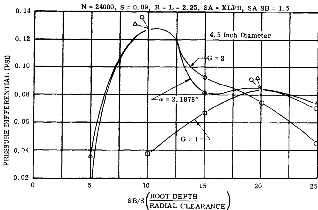
HOLWECK PUMP PARAMETRIC DATA, EFFECT OF SB/S, 4.5 IN. DIA
