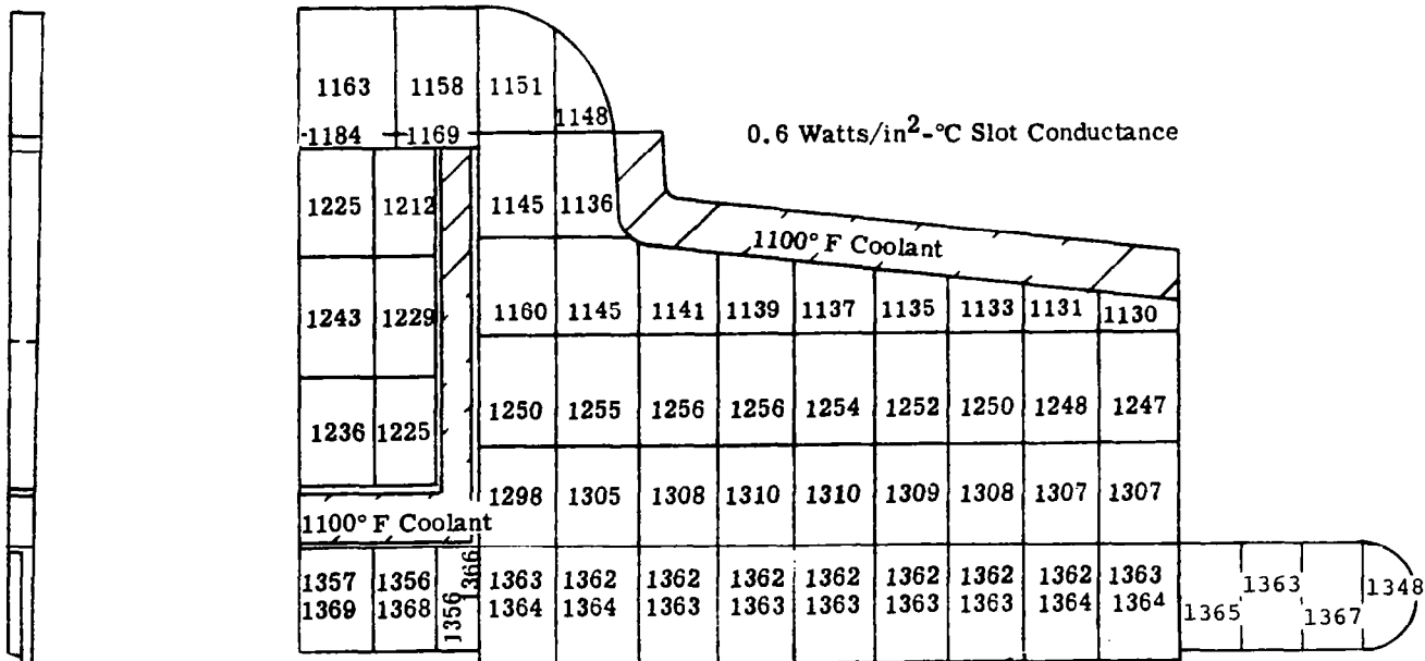
STATOR COOLING SCREENING STUDY, TEMPERATURE DISTRIBUTION (°F) MANIFOLD AND FIELD COIL COOLING WITH AC WINDING COOLING FINS, 1100°F COOLANT, END TURN RADIATION -0.6 W/IN. 2 °C SLOT CONDUCTANCE
