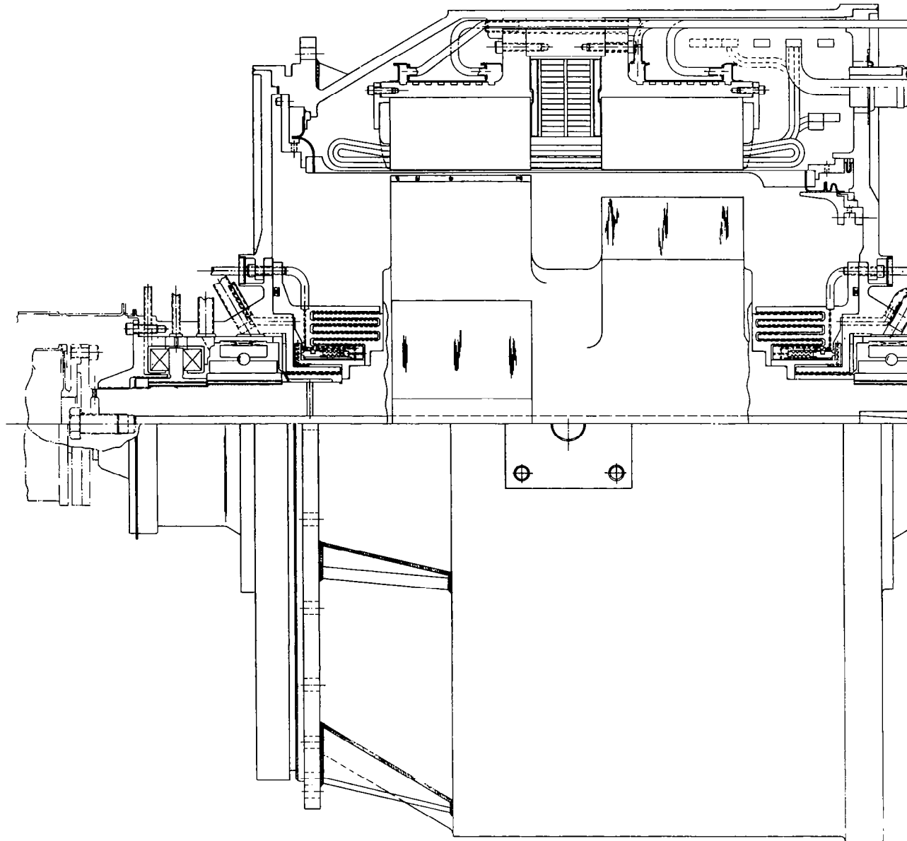
CONCEPTUAL DESIGN LAYOUT, 19,200 RPM, 800°F COOLANT
