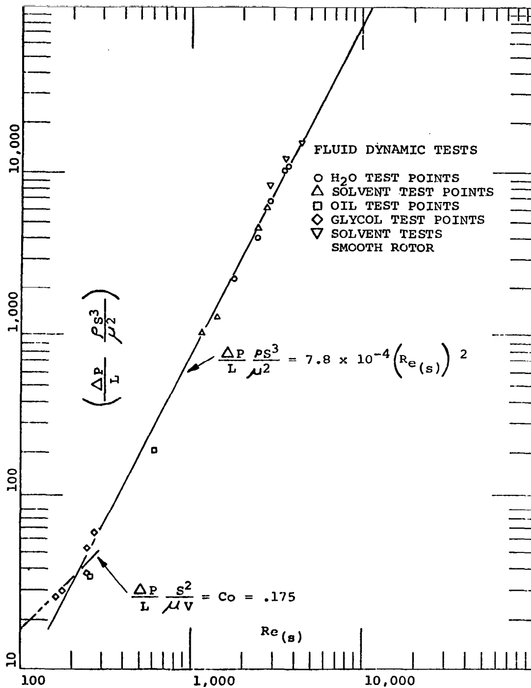
DIMENSIONLESS PLOT OF EXPERIMENTAL DATA FROM VISCOSALS IN TEST FIXTURE DESCRIBED IN REFERENCE 16
