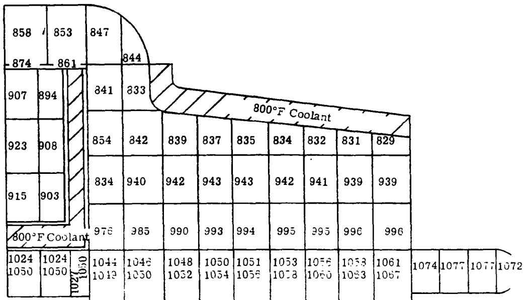
STATOR COOLING SCREENING STUDY, TEMPERATURE DISTRIBUTION (°F) MANIFOLD AND FIELD COIL COOLING WITH AC WINDING COOLING FINS, 800°F COOLANT, END TURN RADIATION
