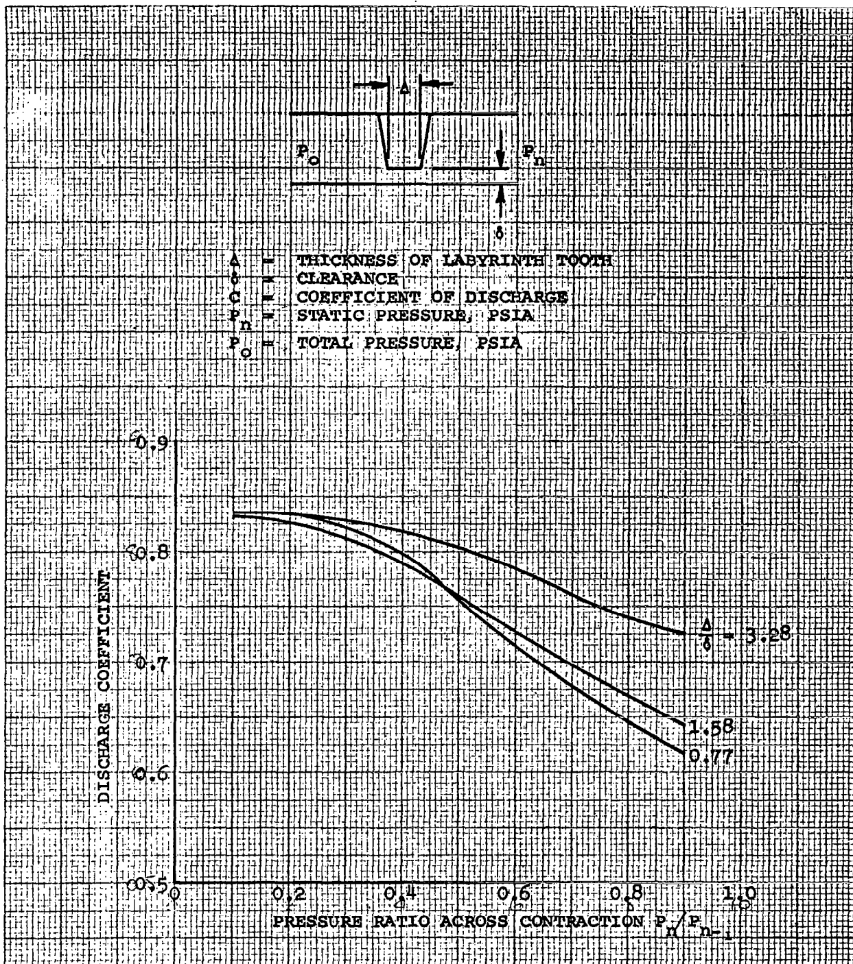
COEFFICIENT OF DISCHARGE FOR CONTRACTIONS FROM KEARTON AND KER
