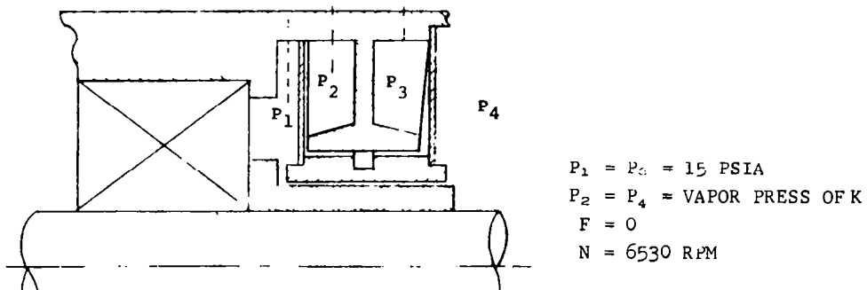
c. SEAL STATE AT LIFT-OFF
