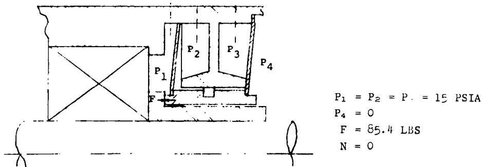
b. SEAL STATE PRIOR TO INITIAL ACCELERATION
