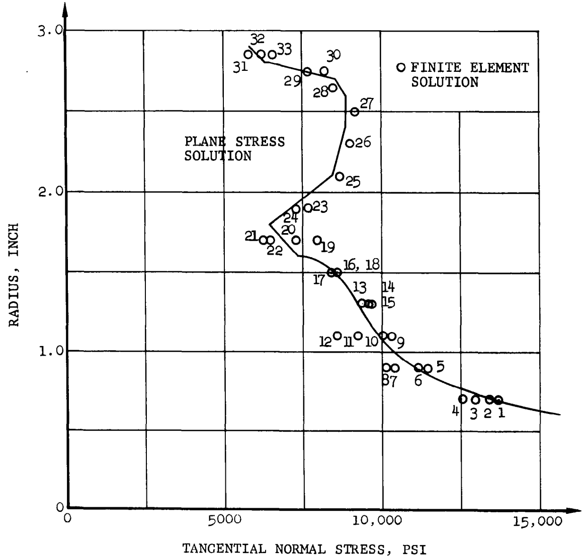
COMPARISON OF TANGENTIAL STRESSES OBTAINED BY PLANE STRESS SOLUTION AND FINITE ELEMENT METHODS
