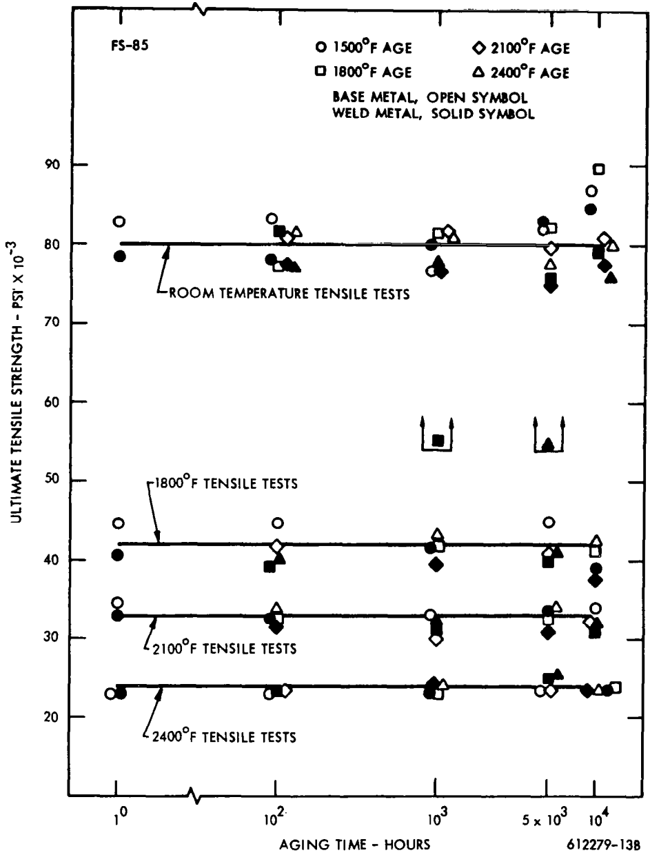
FIGURE 4 - Effect of Aging on the Ultimate Tensile Strength of FS-85 (Ref. 7) All Specimens Annealed 1 Hour at 2400°F Before Aging
