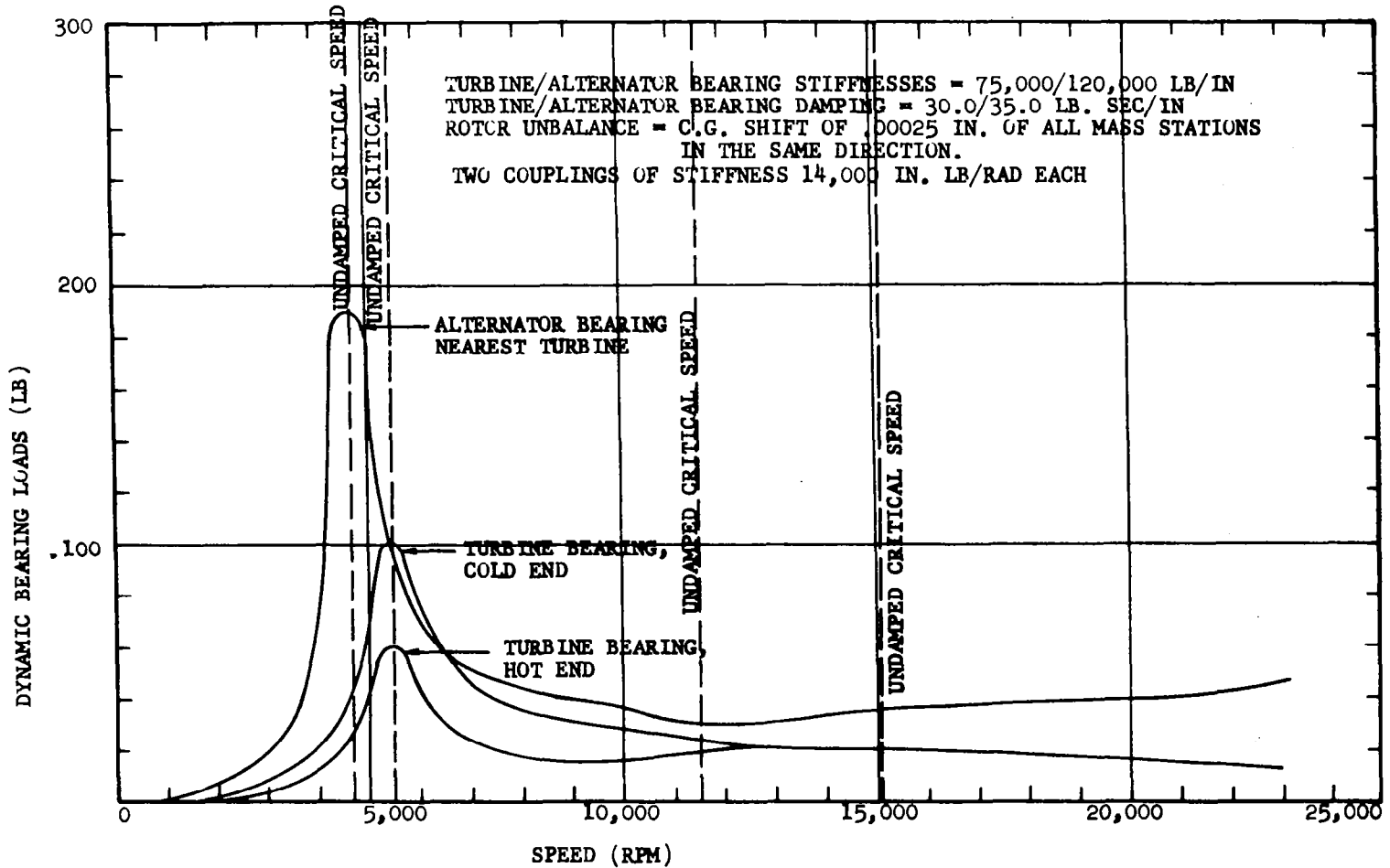
KTA TURBINE-ALTERNATOR COUPLED CRITICAL SPEED ANALYSIS
