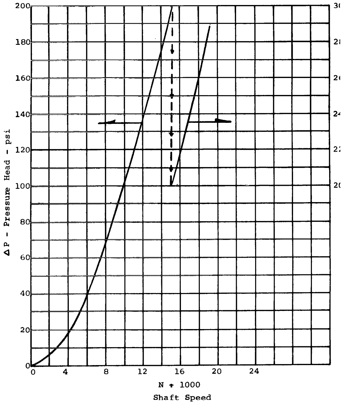
SLINGER CENTRIFUGAL HEAD
