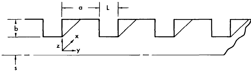
HOLWECK MOLECULAR PUMP SCHEMATIC
