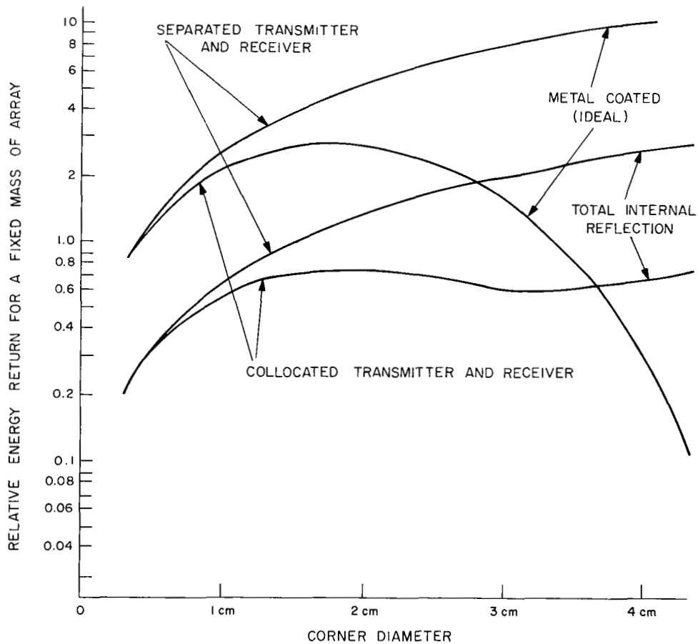
Figure 2-1. The energy of the laser signal reflected from an array of diffraction-limited corners as a function of corner size, for a fixed weight of array on a geosynchronous satellite.
