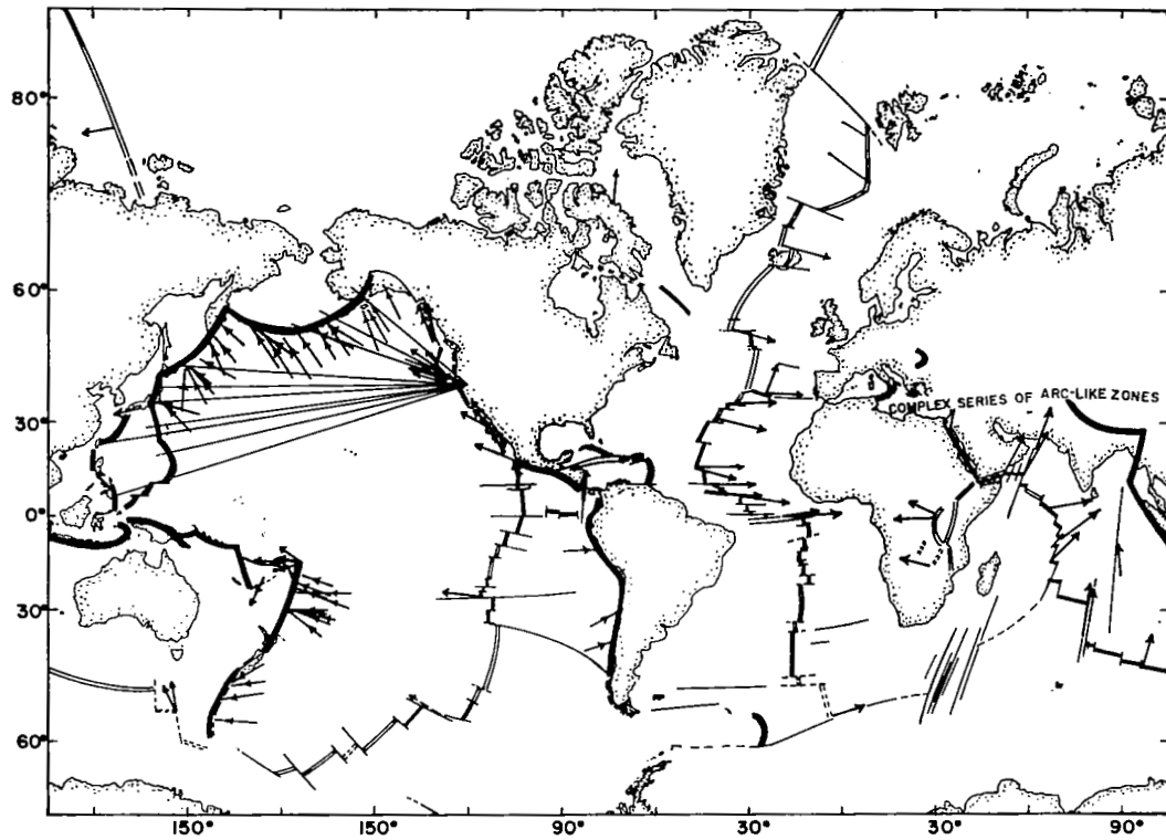
Figure 5-2. Slip vectors derived from earthquake-mechanism studies. Short arrows indicate horizontal components of direction of relative motion of block on which arrow is drawn to adjoining block. Compare with the directions in Figure 5-3 inferred from magnetic anomaly patterns. Long arrows indicate suggested radio-interferometer baselines using the Goldstone facility. 1
