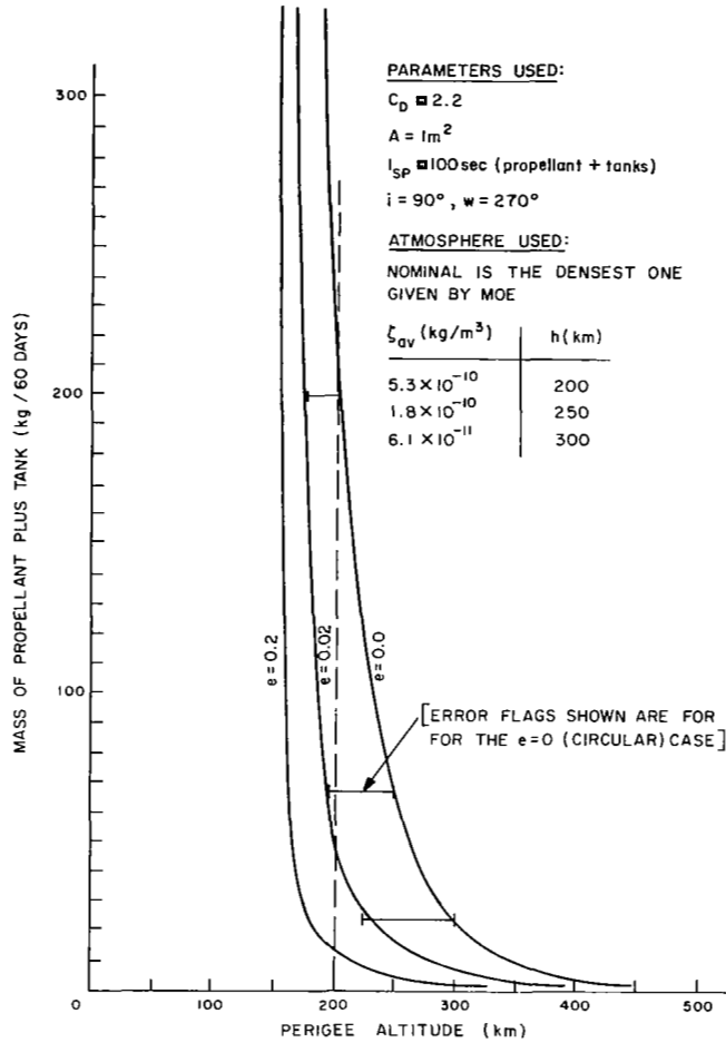
Figure 2-2. Drag-free satellite propulsion system mass as a function of perigee altitude and eccentricity for a cold-gas thruster.
