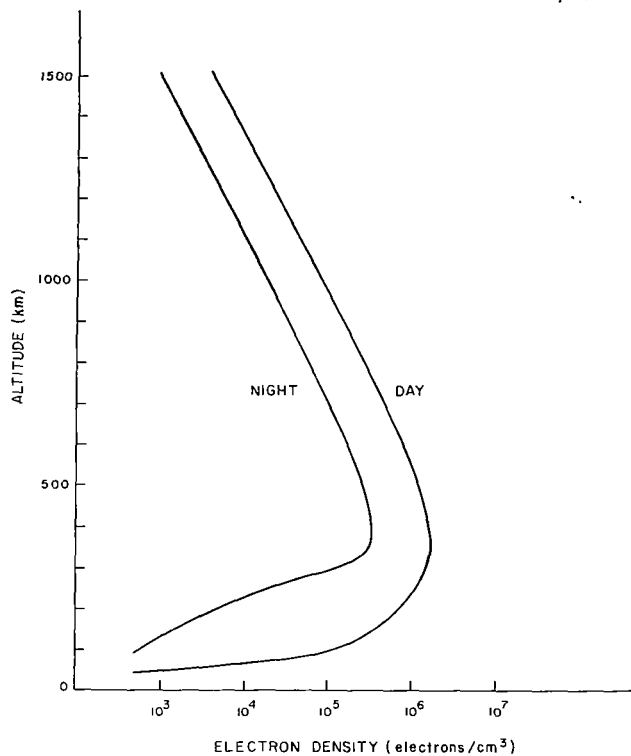
Figure 2-3. Representative ionospheric electron density as a function of altitude.
