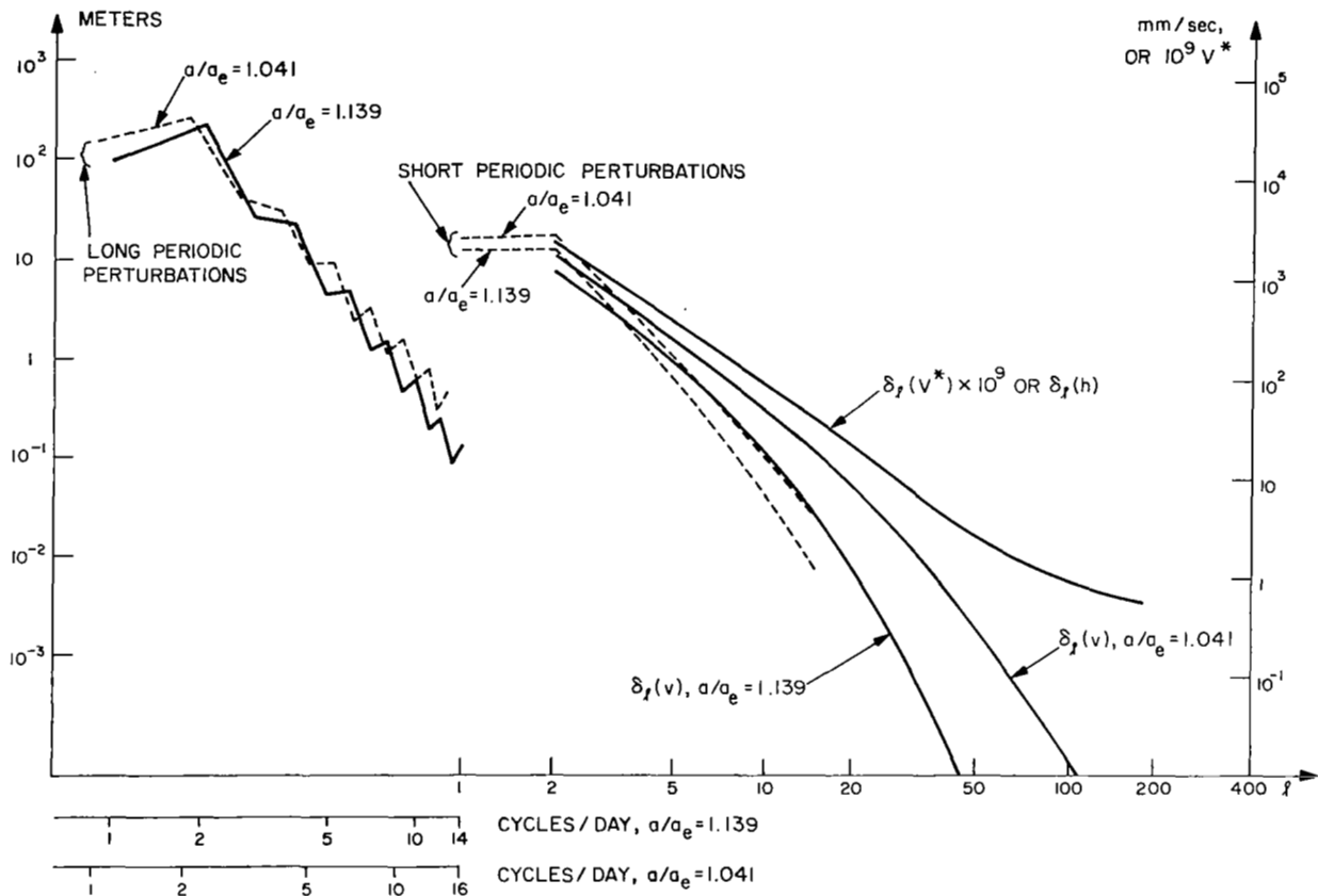
Figure 5-7. Spectra related to the earth's gravity field in terms of the root-mean-square amplitude of a single normalized spherical harmonic coefficient of degree l , \delta_l , for 1), the dimensionless potential V^* (right ordinate), and geoid height h (left ordinate); 2) velocity v (right ordinate) for orbits of altitude 260 km ( a/a_e = 1.041 ) and 890 km ( a/a_e = 1.139 ); and 3) long and short periodic perturbations (left ordinate) for orbits of these same altitudes. 17
