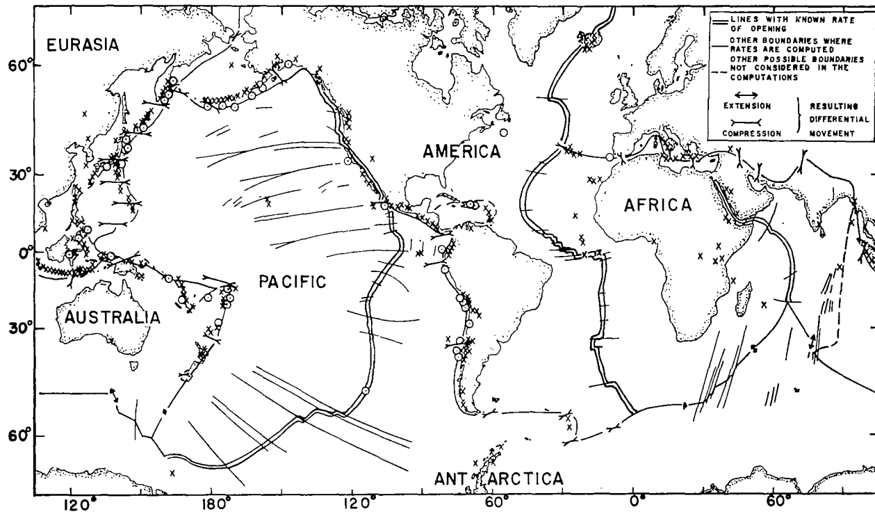
Figure 5-3. Computed rates of compression and extension along boundaries of six lithospheric blocks (after Le Pichon 5 ). Computed movements were derived from rates of spreading determined from magnetic data and from orientations of fracture zones along features indicated by double lines. The extensional and compressional symbols in the legend represent rates of 10 cm/yr; other similar symbols are scaled proportionally. Symbols appearing as diamonds represent small computed rates of extension for which the arrowheads coalesced. Historically active volcanoes (see Gutenberg and Richter 5 ) are denoted by crosses. Open circles represent earthquakes that generated tsunamis (seismic sea waves) detected at distances of 1000 km or more from the source. 1
