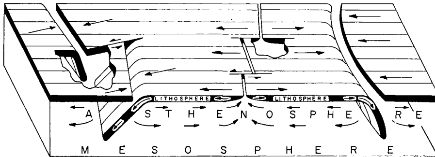
Figure 5-1. Block diagram illustrating schematically the configurations and roles of the lithosphere, asthenosphere, and mesosphere in a version of the new global tectonics in which the lithosphere, a layer of strength, plays a key role. Arrows on lithosphere indicate relative movements of adjoining blocks. Arrows in asthenosphere represent possible compensating flow in response to downward movement of segments of lithosphere. One arc-to-arc transform fault appears at left between oppositely facing zones of convergence (island arcs), two ridge-to-ridge transform faults along ocean ridge at center, simple arc structure at right. 1
