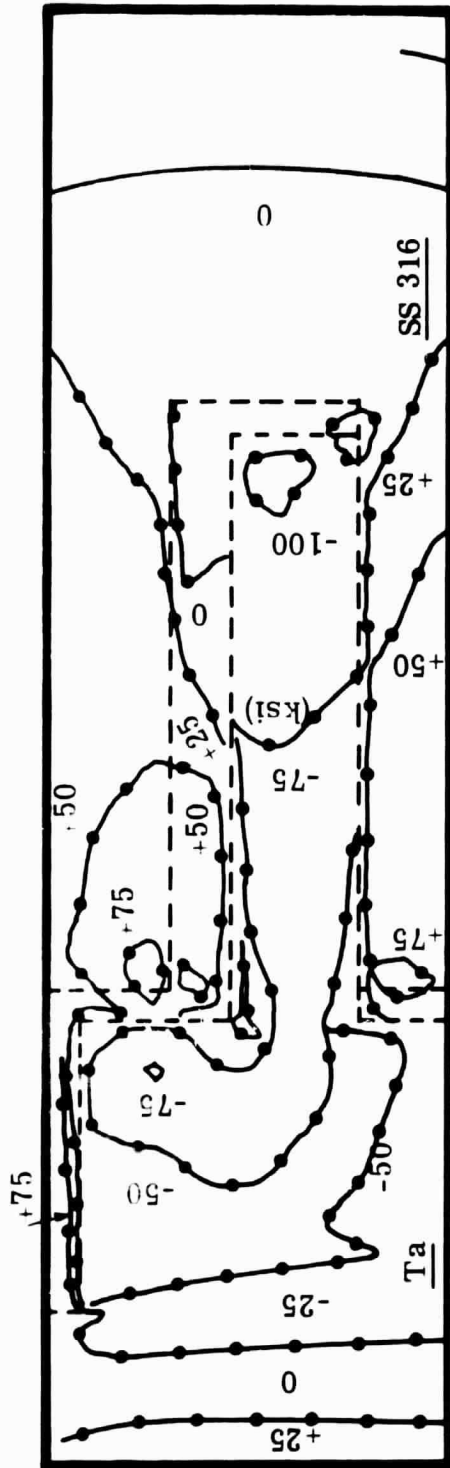
Figure 8. Residual Hoop Stresses Due Cool-down Bi-linear Iterations (1)
