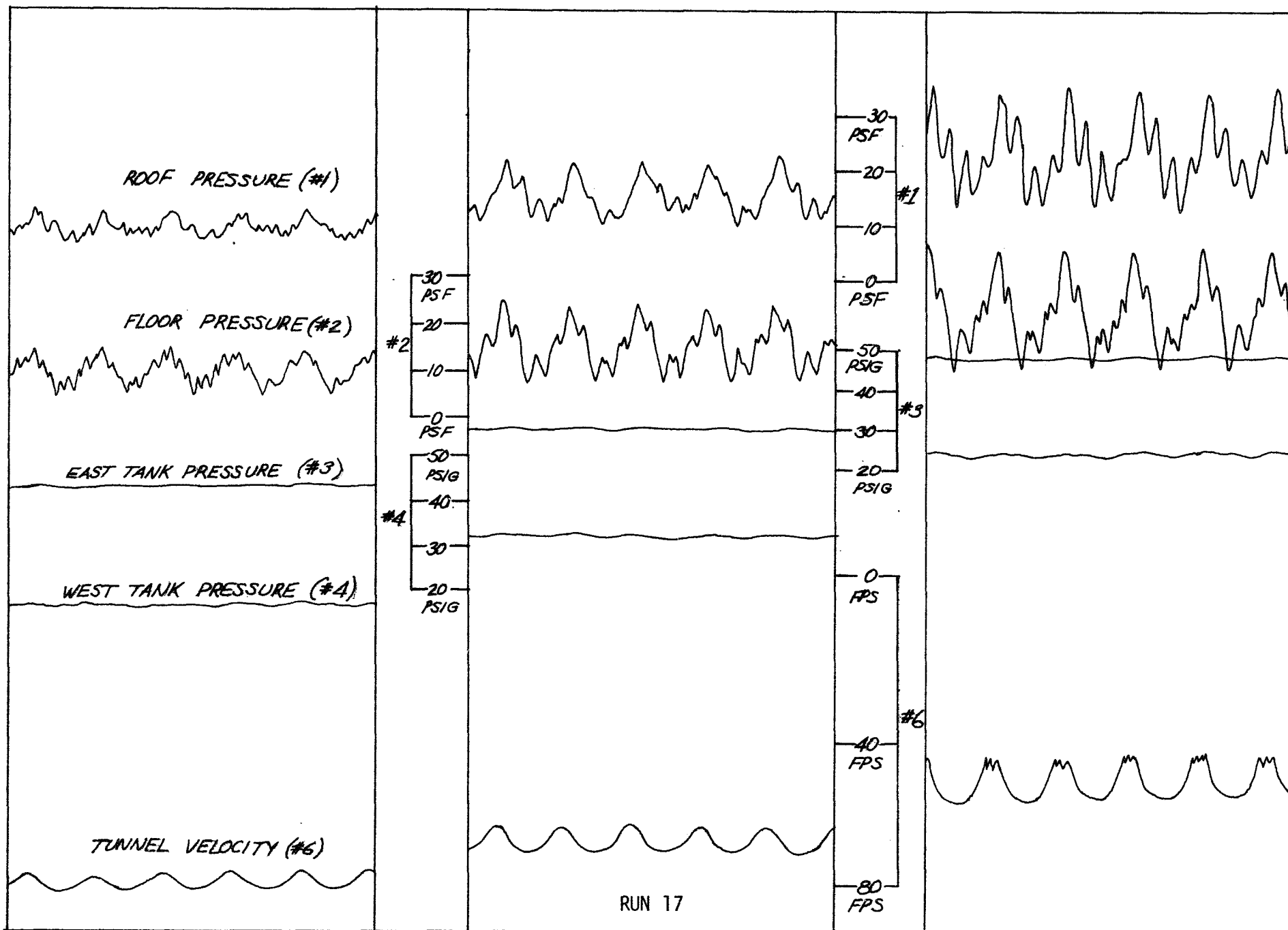
FIG. 9. GUSTS AT 38 HZ VALVES 30^\circ OUT OF PHASE
