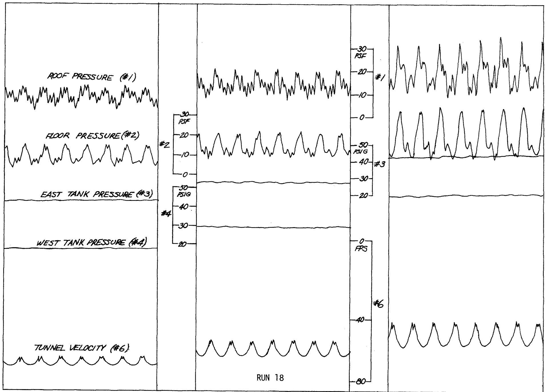
FIG. 10. GUSTS AT 54 HZ VALVES 30^{\circ} OUT OF PHASE
