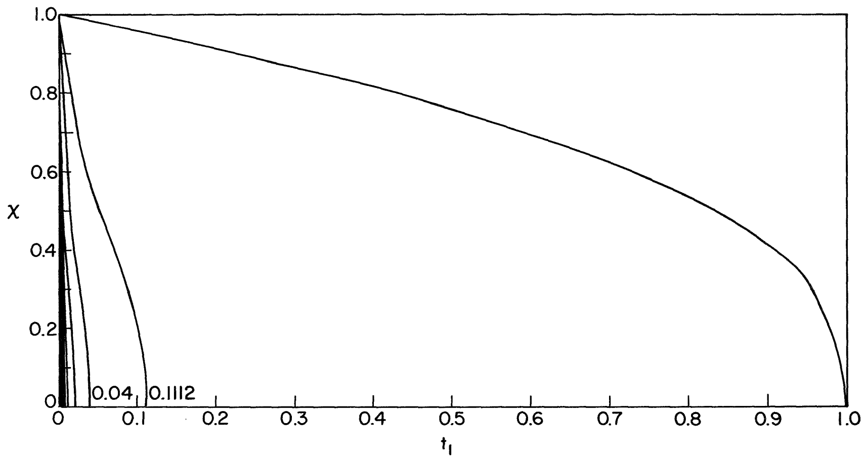
Fig. 1.3 Variation of \chi with respect to the minimal thickness constraint t_1 . \chi is the root of \chi = \frac{\sqrt{t_1}}{\omega} \cot \frac{\omega}{\sqrt{t_1}} (1 - \chi) lying between 0 and 1 ( \omega \approx \frac{\pi}{2} ).
