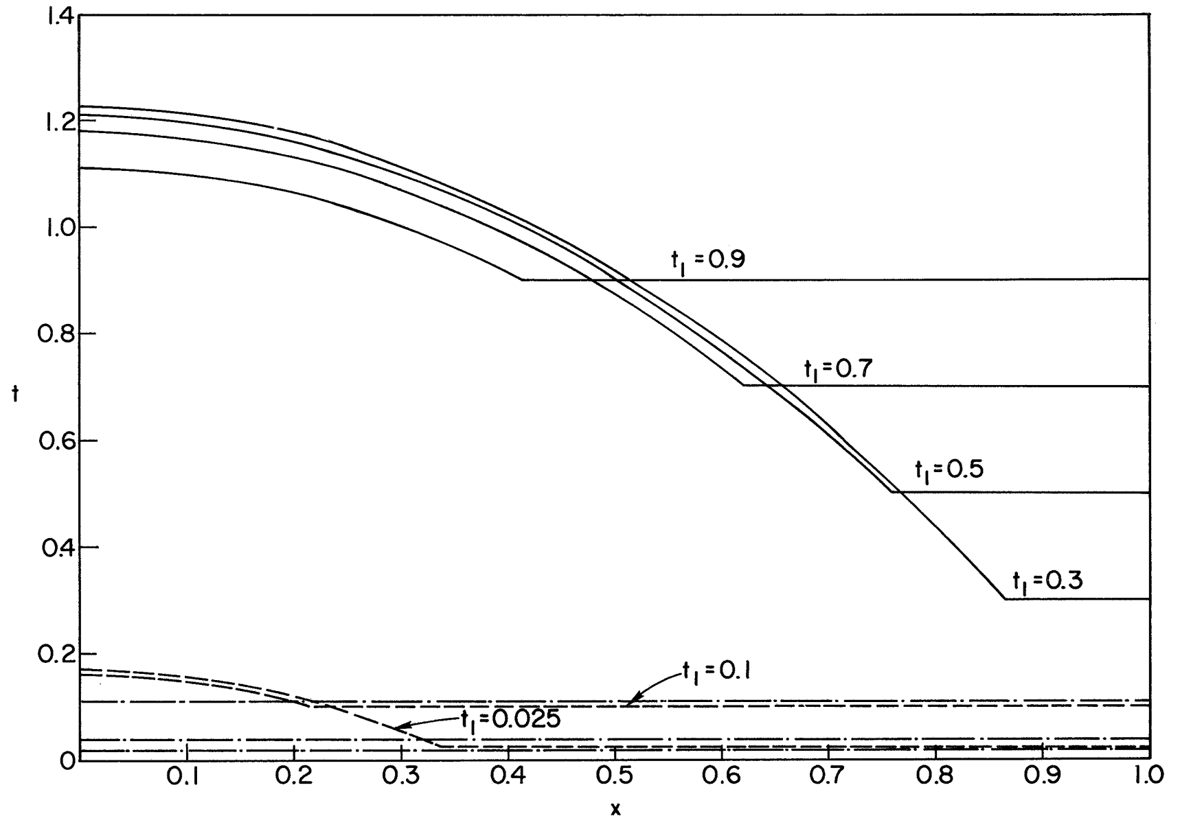
Fig. 1.4 Optimal thickness distributions. Torsional-divergence case with minimum-thickness constraint for different values of t_1 (the dotted lines are the distributions found for t_1 < \frac{1}{3^2} and t_1 < \frac{1}{5^2} respectively as described in Section 1.2.1).
