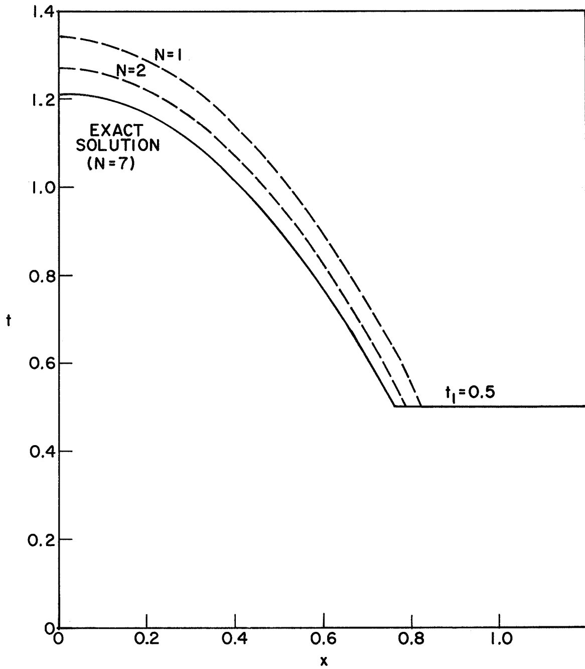
Fig. 1.6 A transition-matrix procedure for the case of torsional divergence with minimum thickness.
