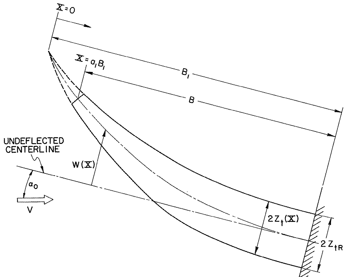
Fig. 3.1 Cross-section of forward half of a plate undergoing chordwise bending in a two-dimensional supersonic airstream.
