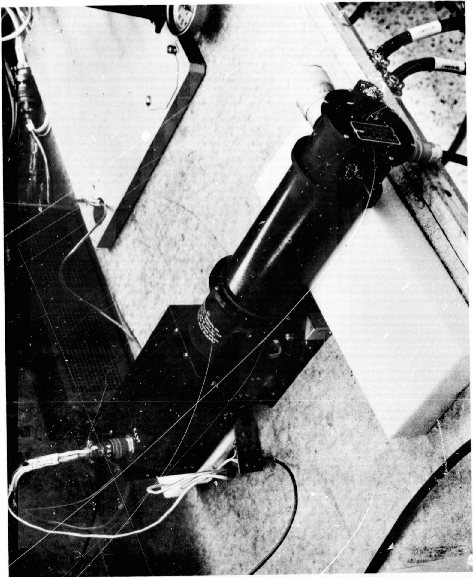
Figure 8-20: CANOPUS STAR TRACKER WITH TEST SET ATTACHED
