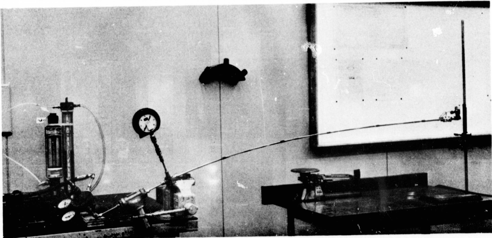
Figure 4-6: REACTION CONTROL THRUSTER FORCE AND IMPULSE TEST SETUP
