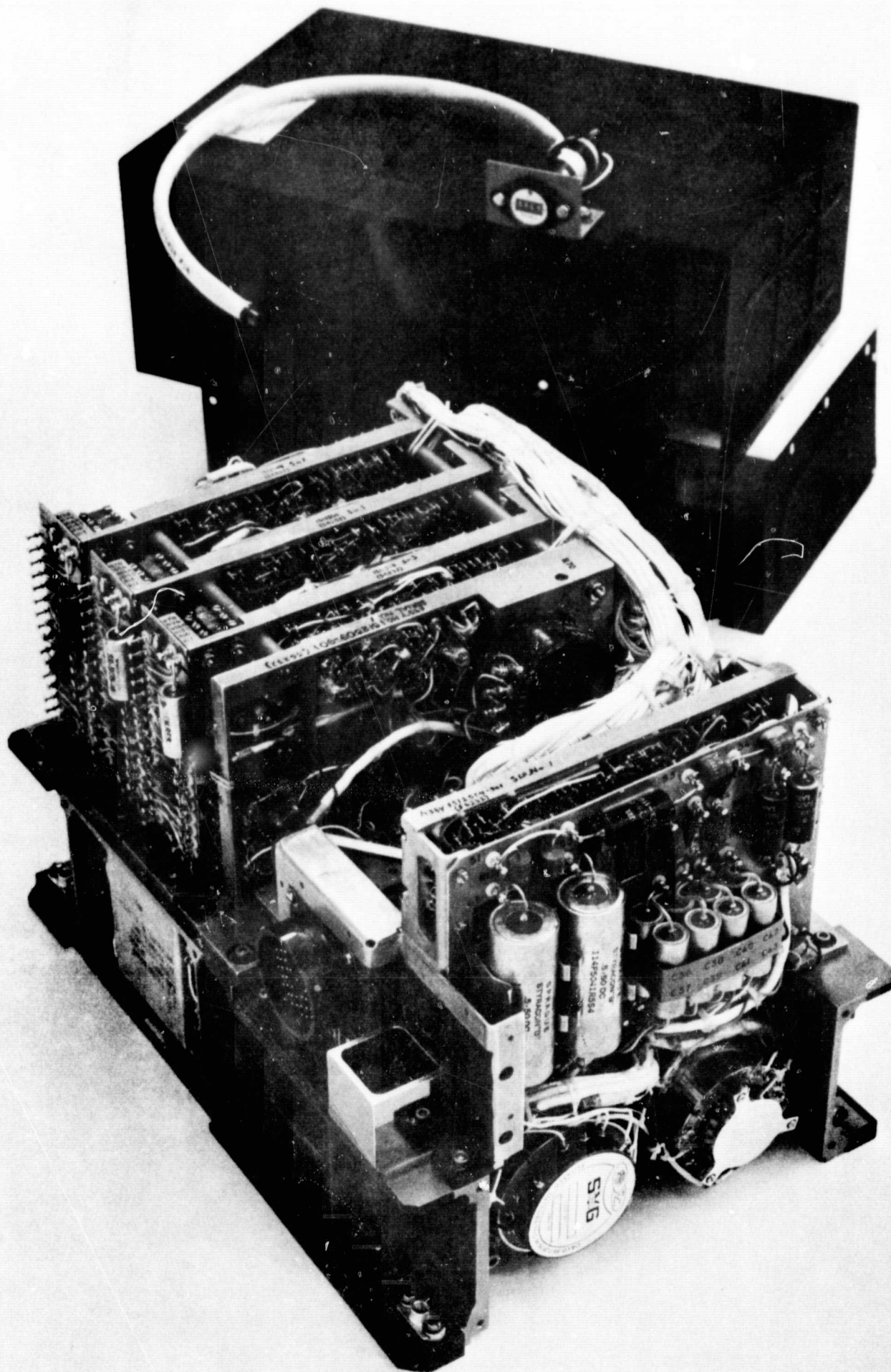
Figure 8-1: INERTIAL REFERENCE UNIT
