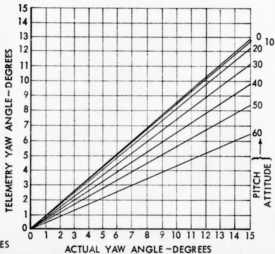
FIGURE 8-18 INFLIGHT COARSE SUN SENSOR CALIBRATION
