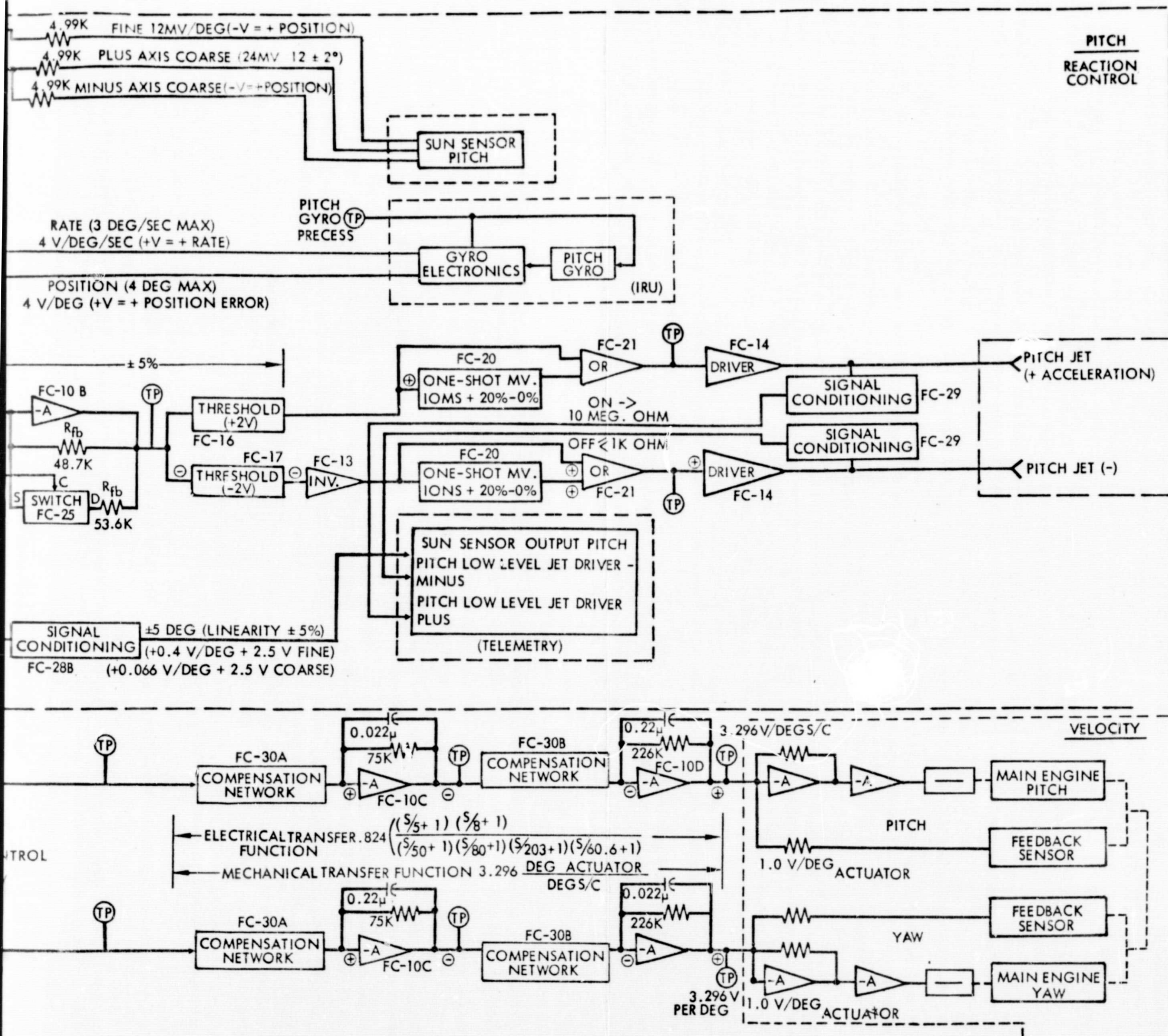
FIGURE 8-35 CLOSED LOOP ELECTRONICS
