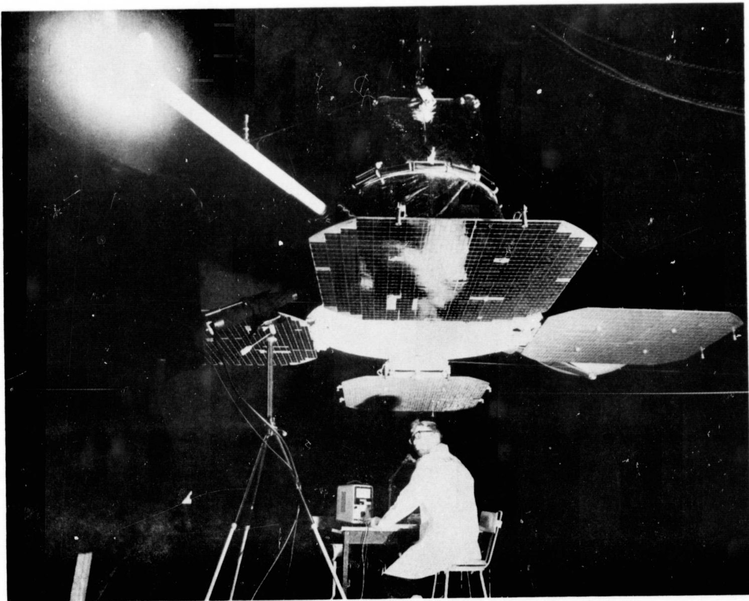
Figure 8-23: GROUND GLINT TEST IN PROGRESS
