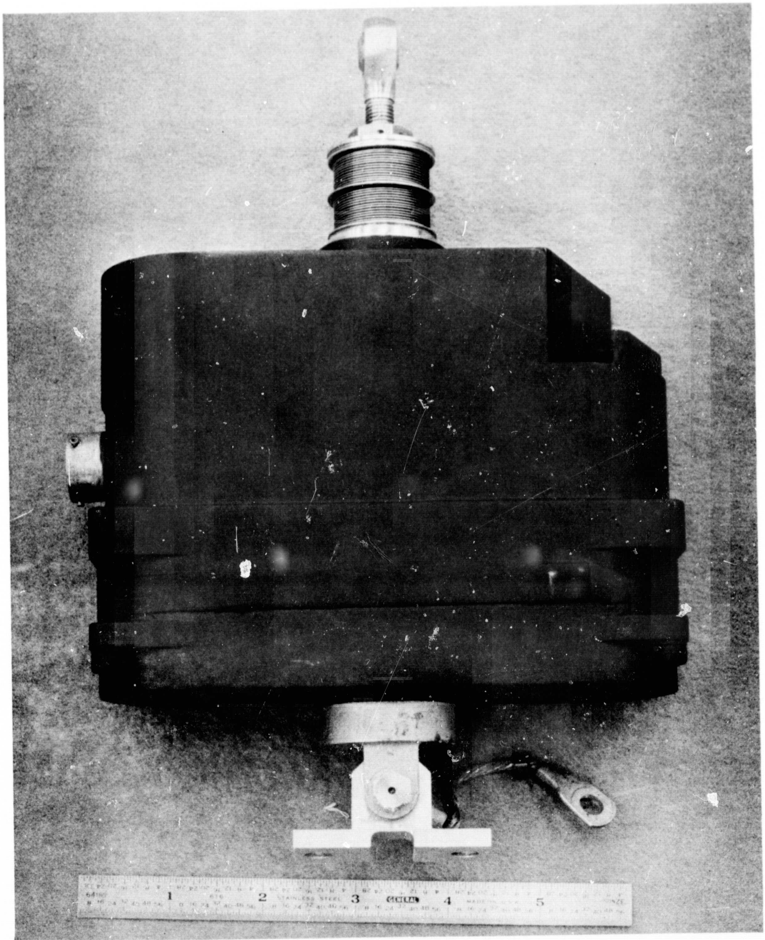
Figure 8-37: THRUST VECTOR CONTROL ACTUATOR
