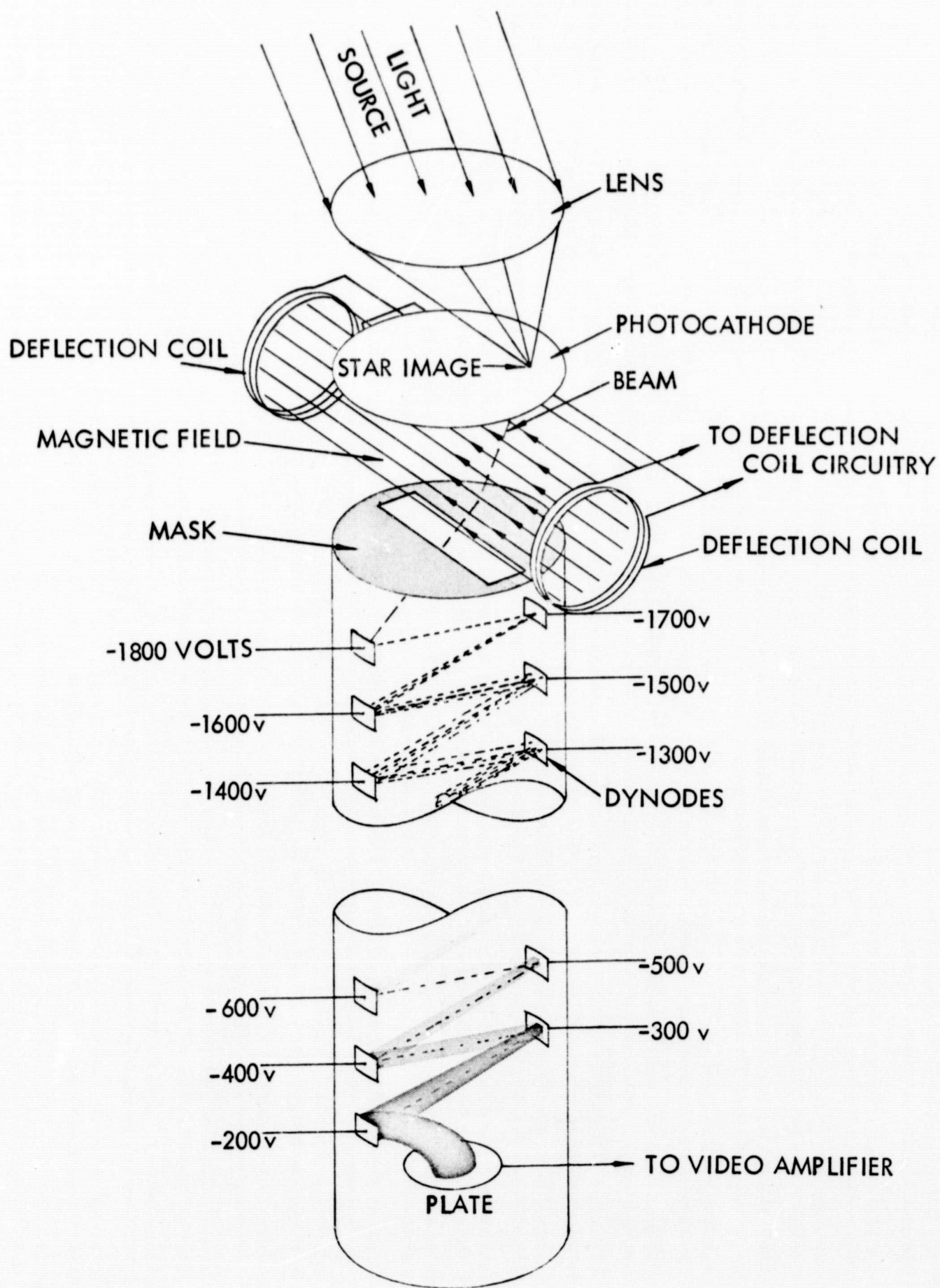
FIGURE 8-19 SCHEMATIC DIAGRAM OF IMAGE DISSECTOR TUBE AND LENS
