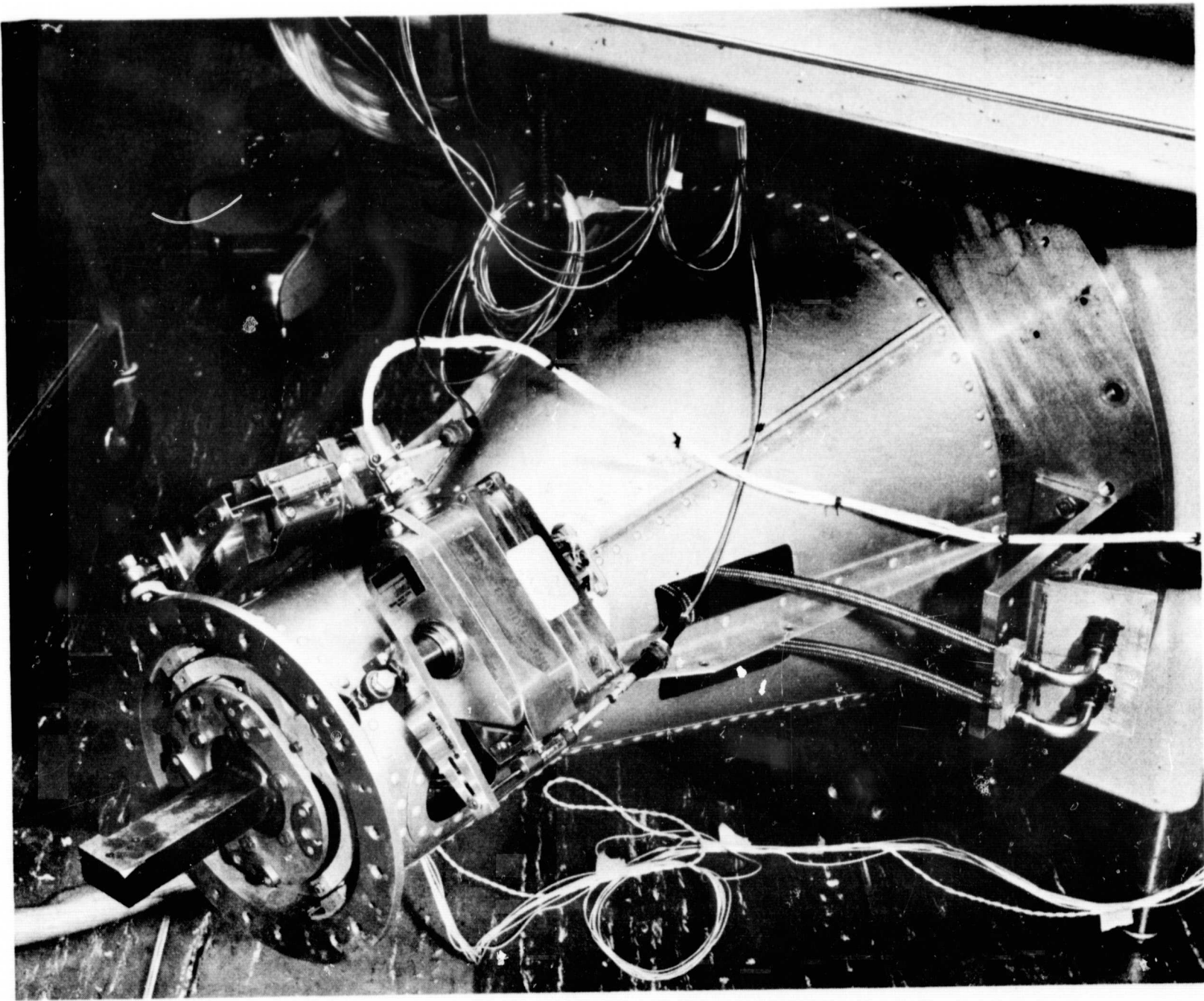
Figure 5-6: CLOSED-LOOP TEST OF THRUST VECTOR CONTROL SYSTEM
