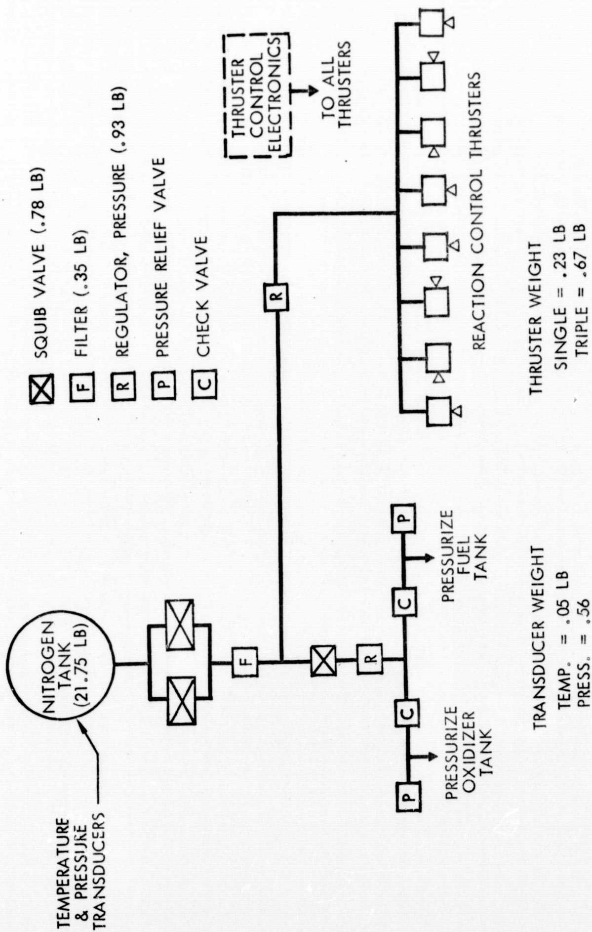
FIGURE 4-2 REACTION CONTROL SUBSYSTEM
