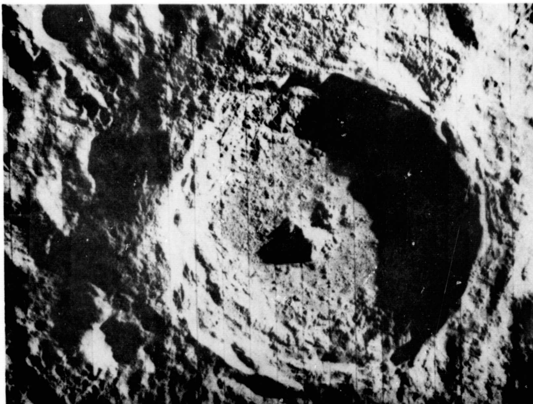
Figure 2.-7: ORIENTALE BASIN
