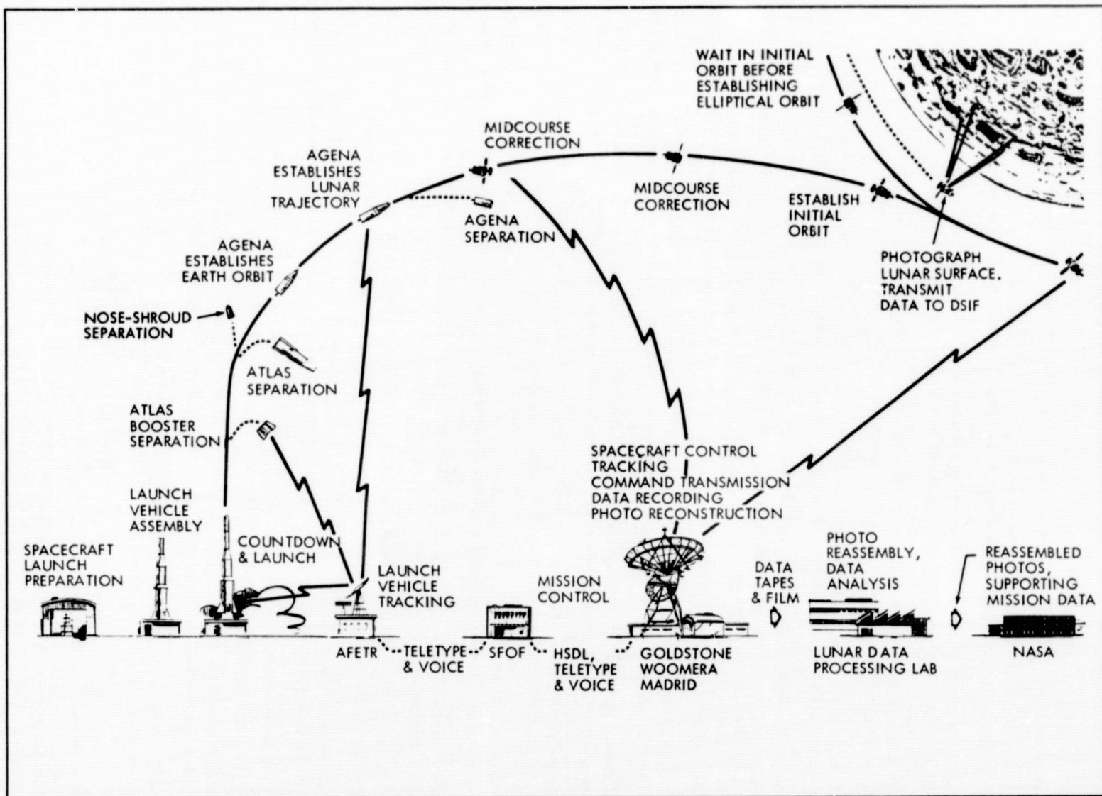
Figure 2-1: THE MISSION
