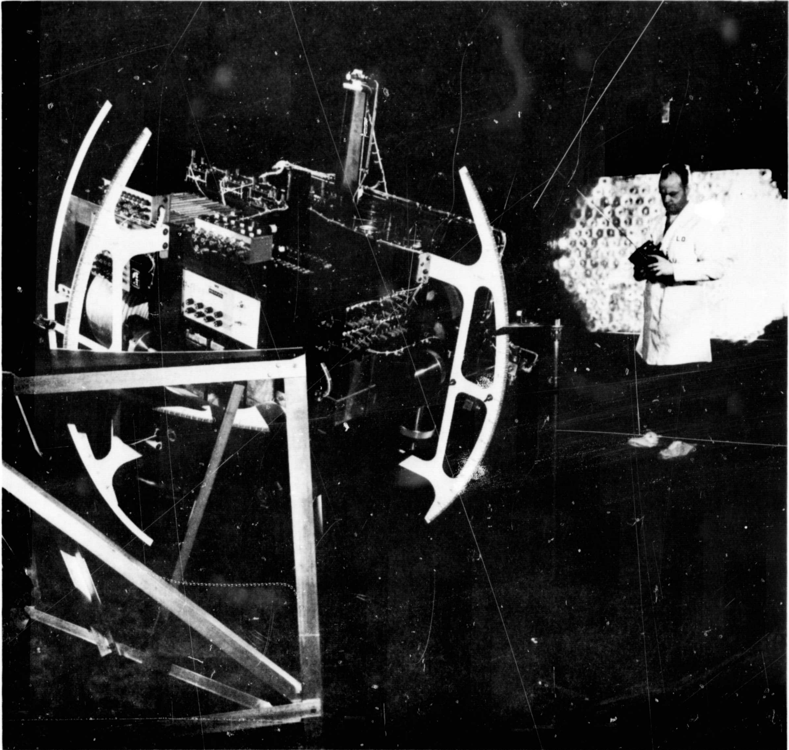
Figure 8-6: ATTITUDE CONTROL SUBSYSTEM Airbearing Simulator
