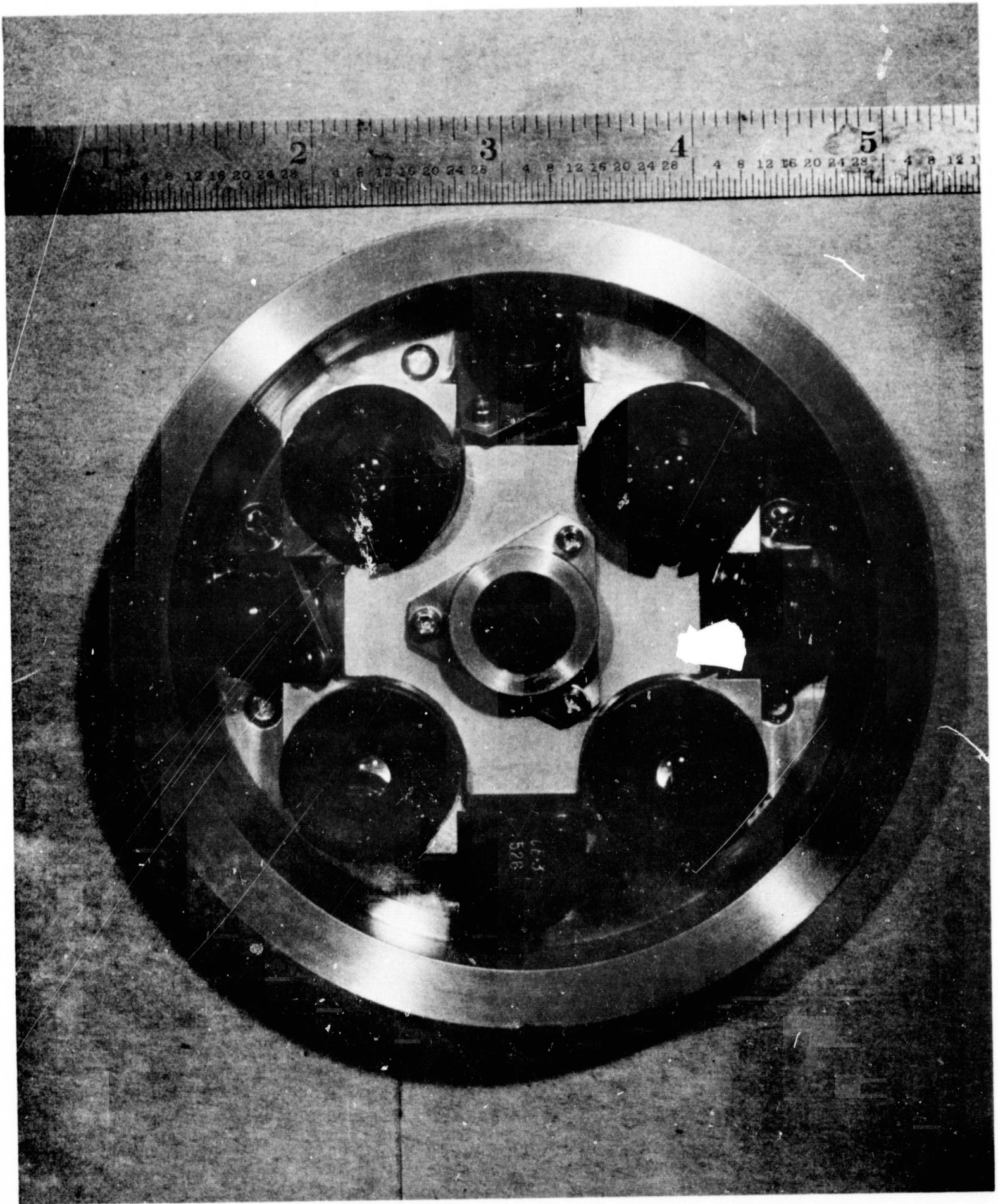
Figure 8-13: MAIN SUN SENSOR
