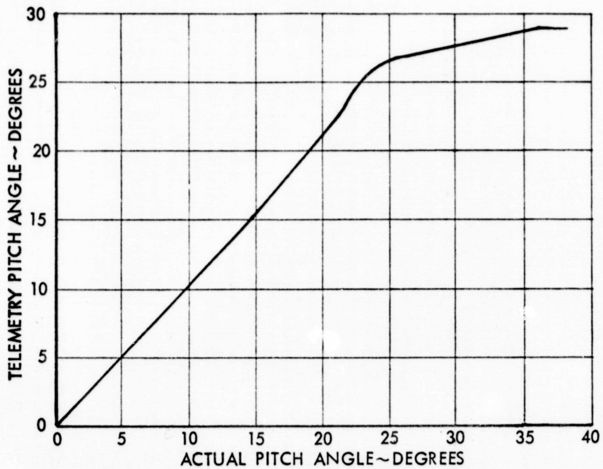
FIGURE 8-17 INFLIGHT COARSE SUN SENSOR CALIBRATION
