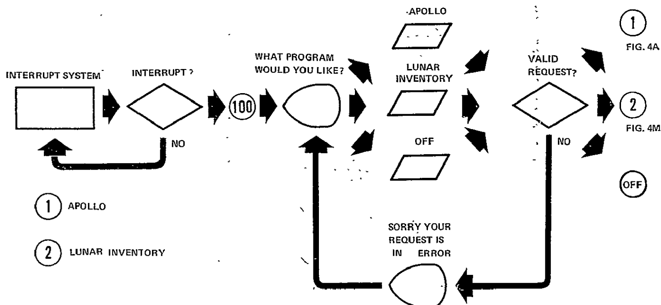
Figure 4. Background Program Console Language
