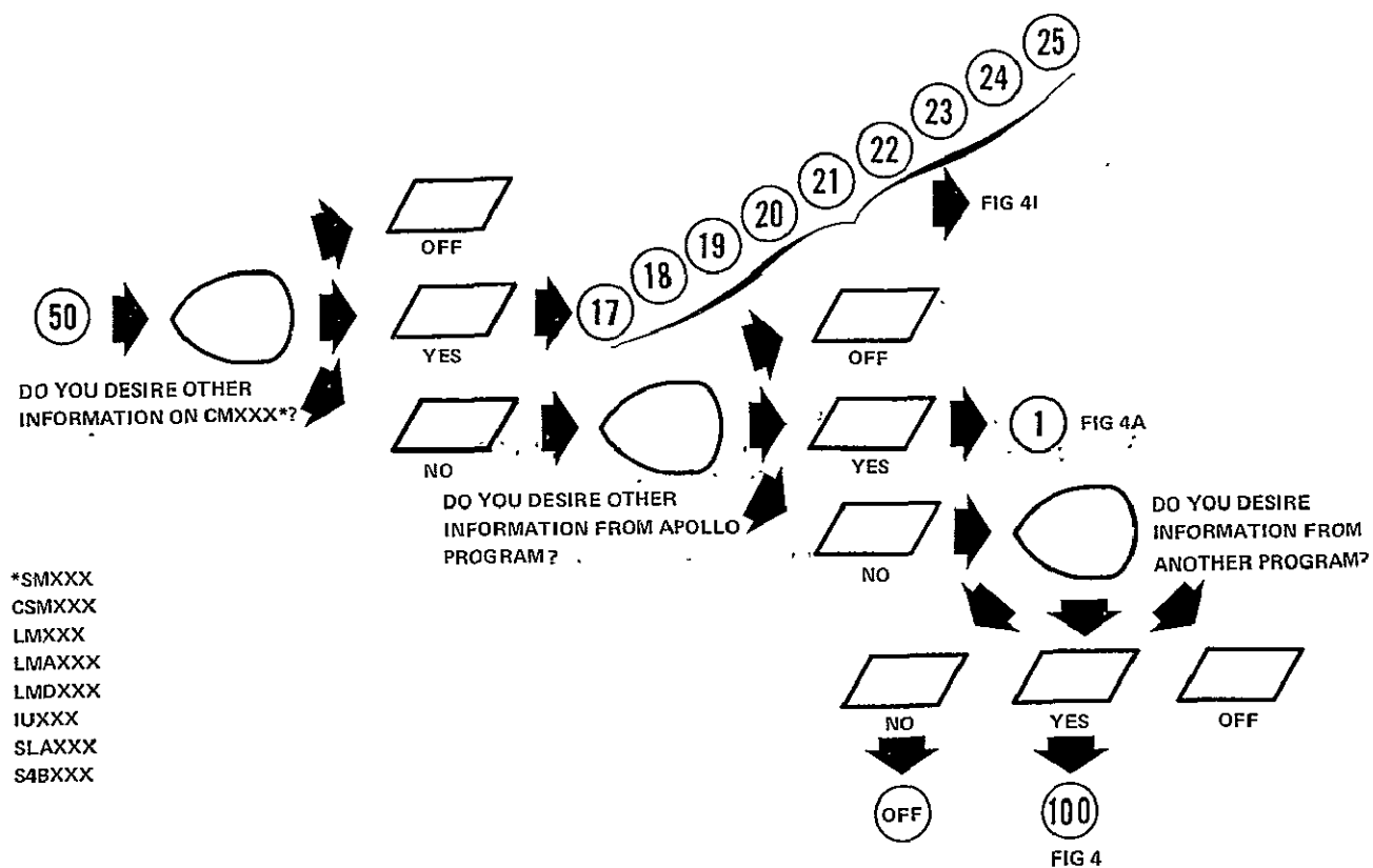
Figure 4L. Background Program Console Language, Apollo (Continued)
