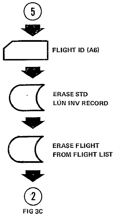
Figure 3E. Lunar Inventory Routine (Continued)
