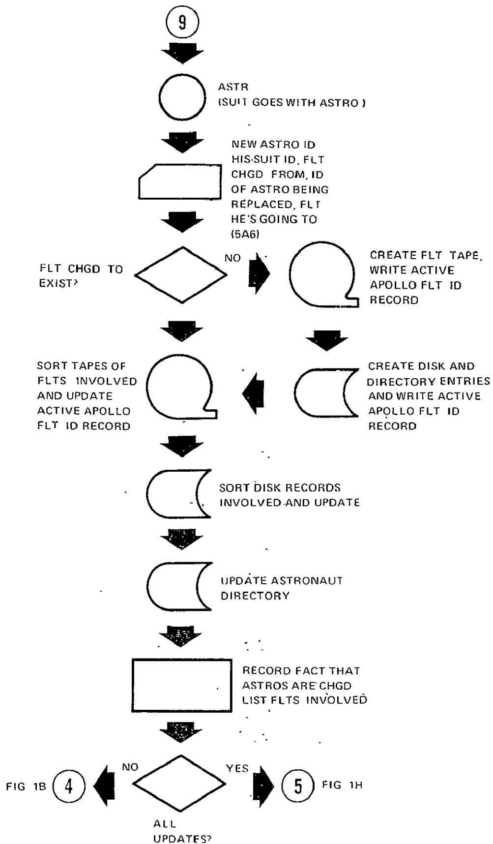
Figure 1F. File Preparation Routine (Continued)
