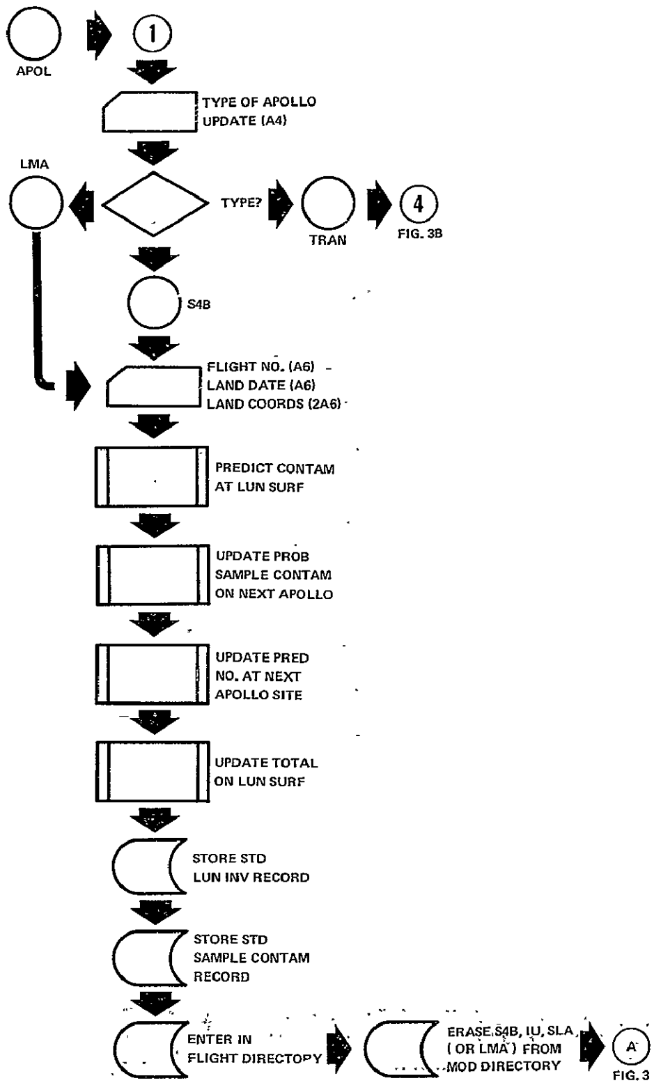
Figure 3A. Lunar Inventory Routine (Continued)
