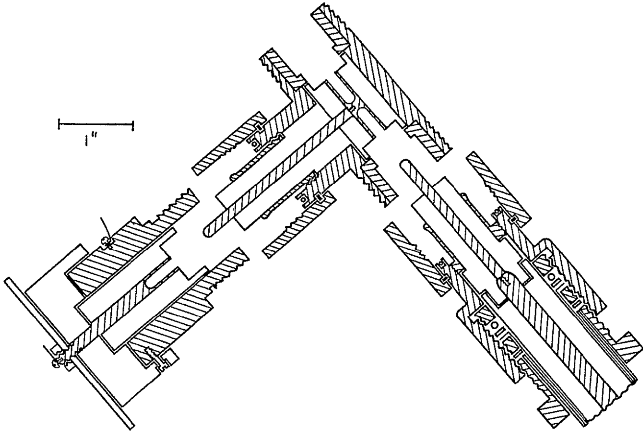
Figure 14. "T" and Coax Connectors
