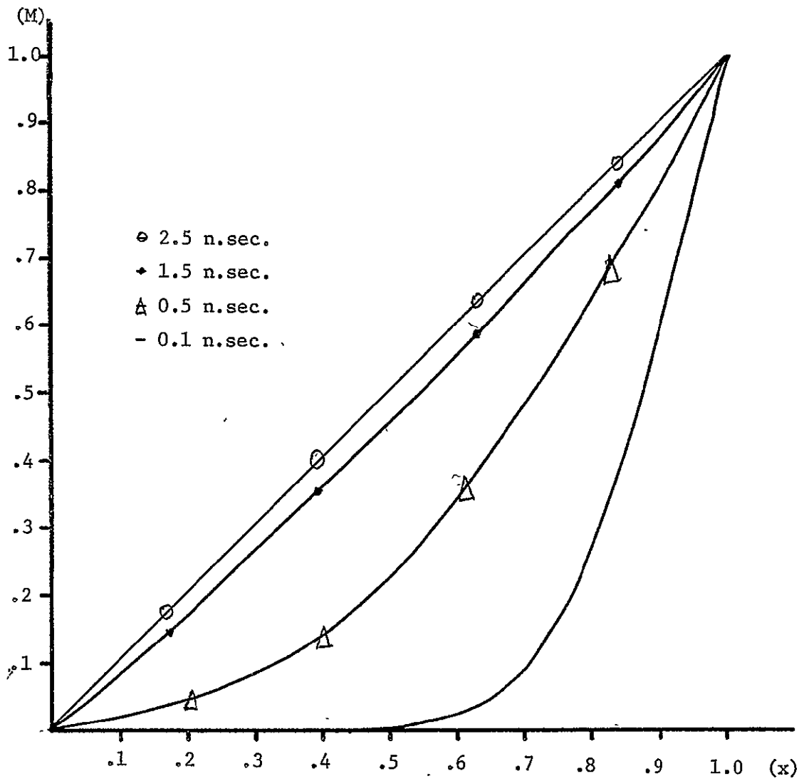
Figure 3. Computer Solution for the Magnetic Induction
