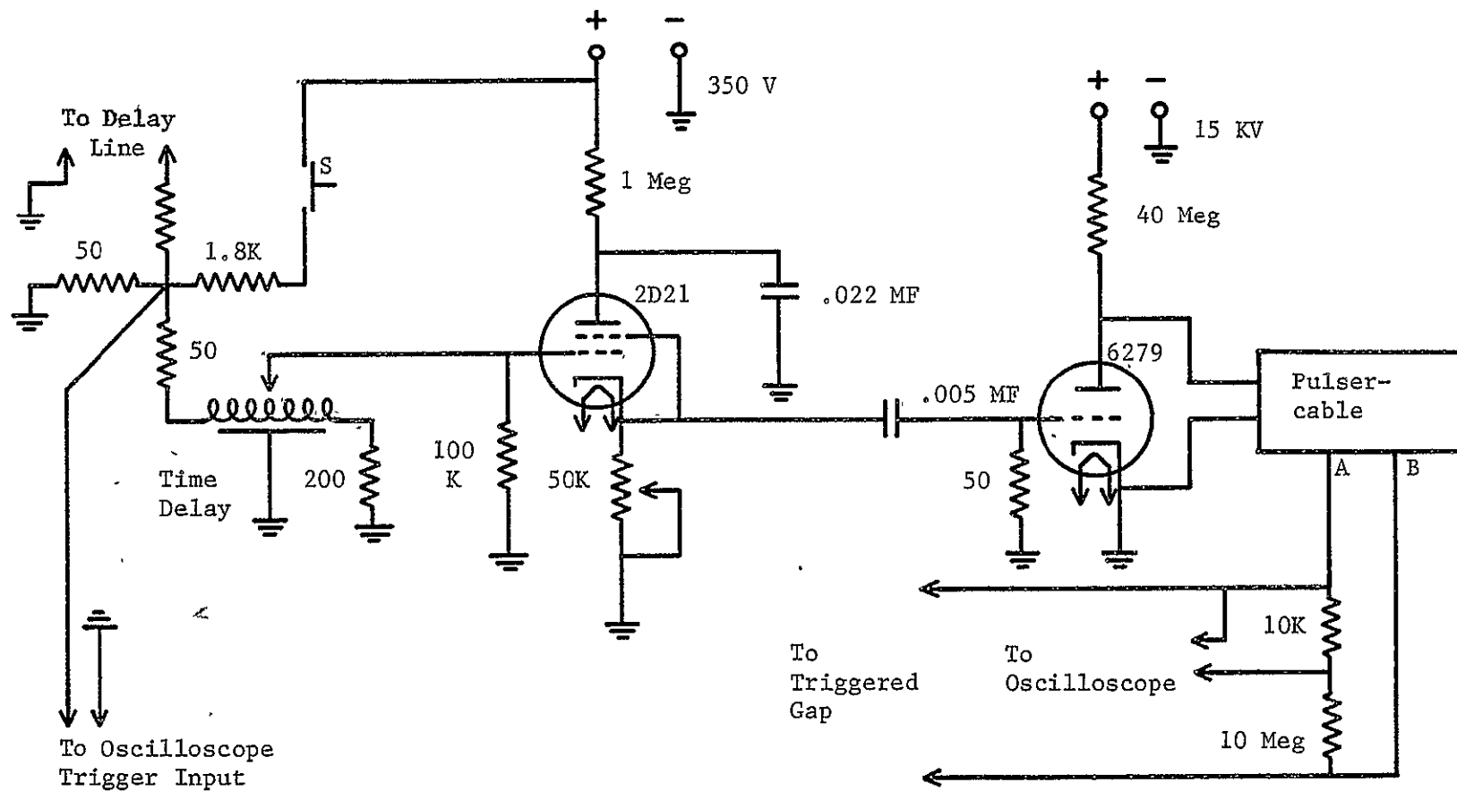
Figure 19. Time Delay and Thyatron Pulser
