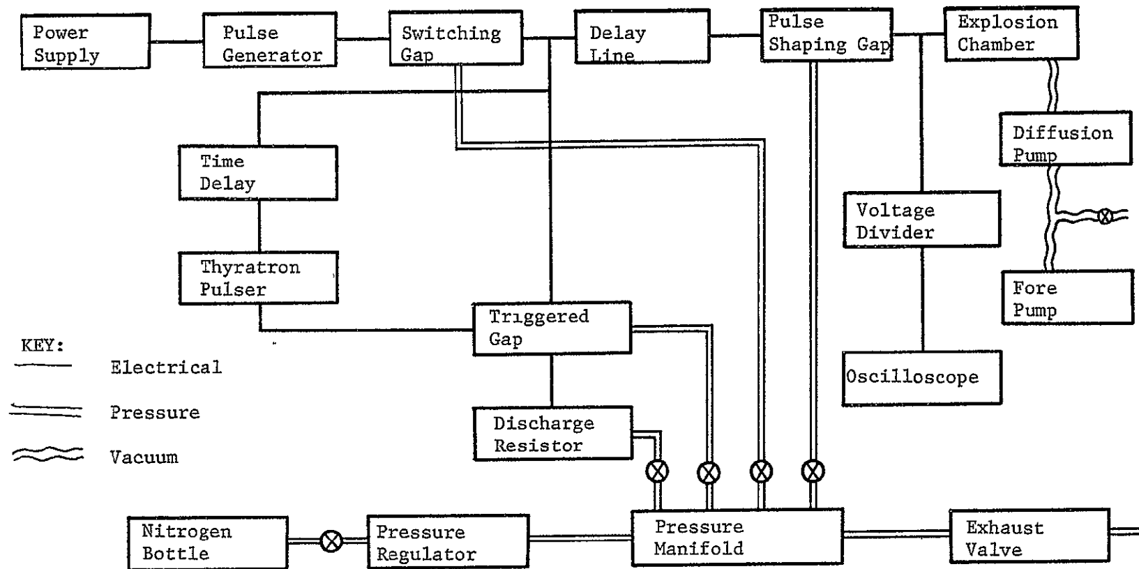
Figure 11. Block Diagram of "Exploding Wire" System
