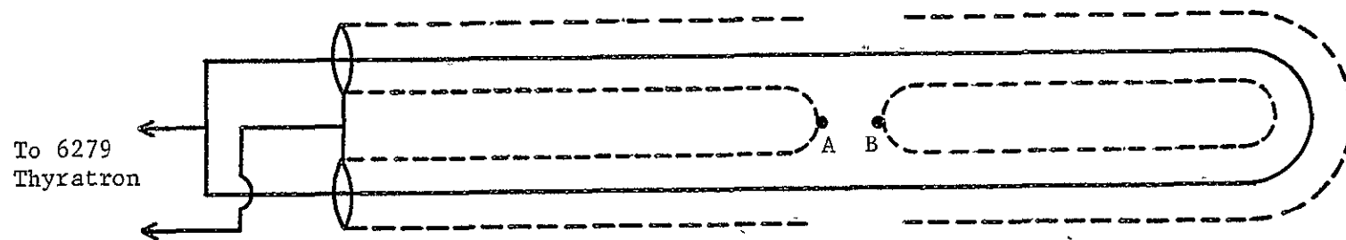
Figure 20. Pulser-cable
