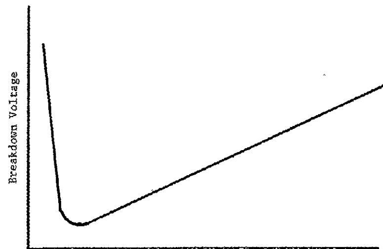
Figure 9. Paschen's Curve
