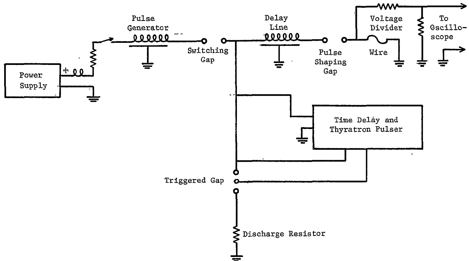
Figure 1. Electrical "Exploding Wire" Circuit
