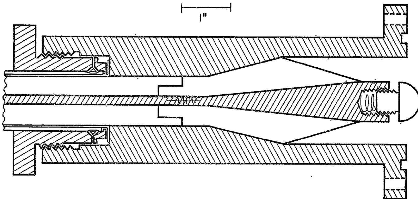
Figure 15. Spark Gap Electrode and Housing
