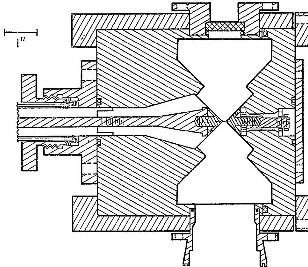
Figure 24. Explosion Chamber
