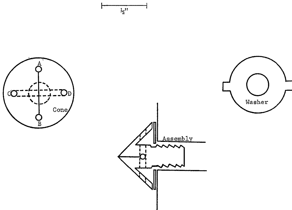
Figure 26. Wire Holder Assimbly
