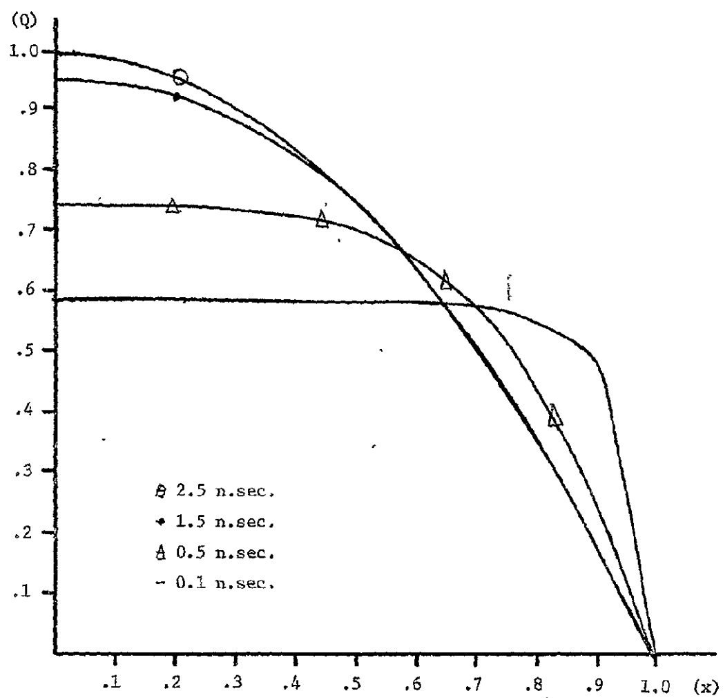
Figure 4. Computer Solution for the "Pinch" Pressure
