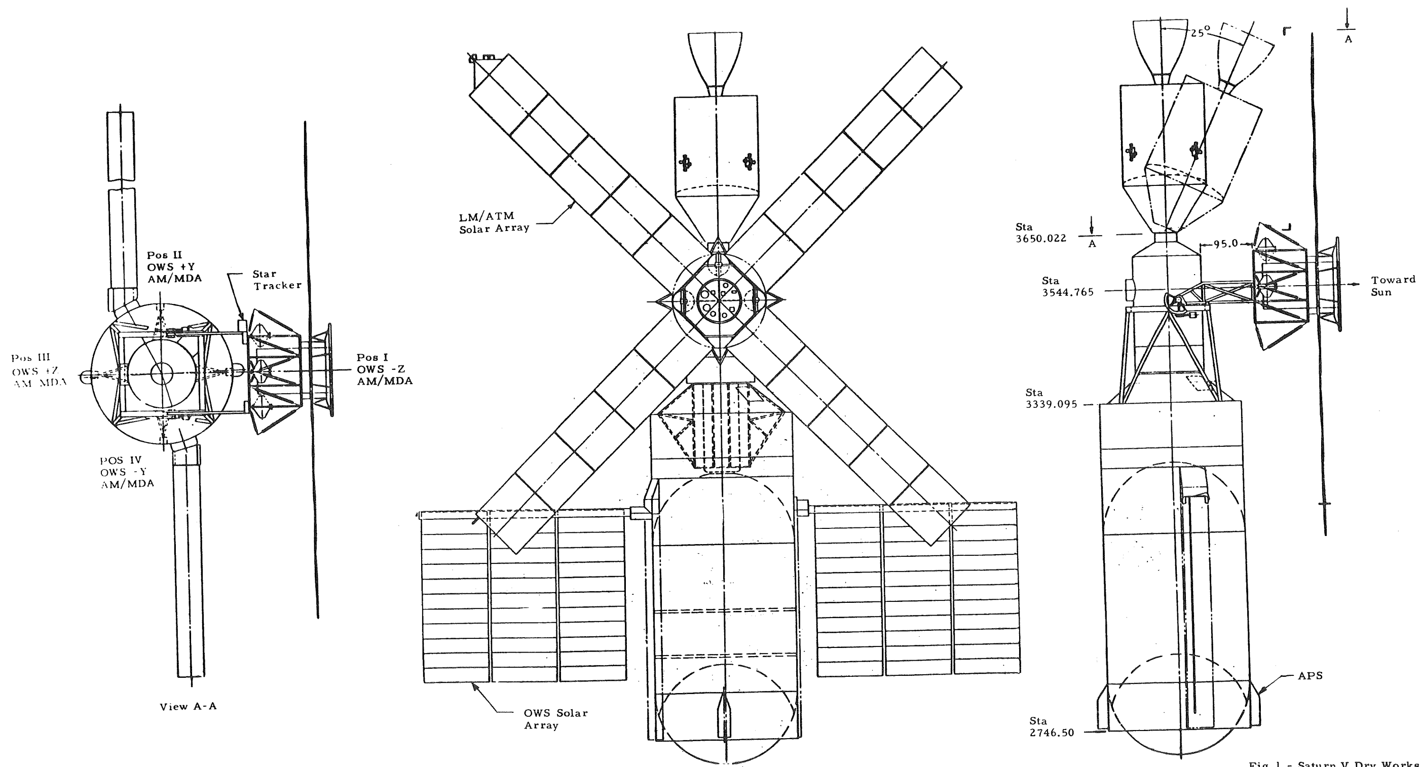
Fig. 1 - Saturn V Dry Workshop Cluster Arrangement
