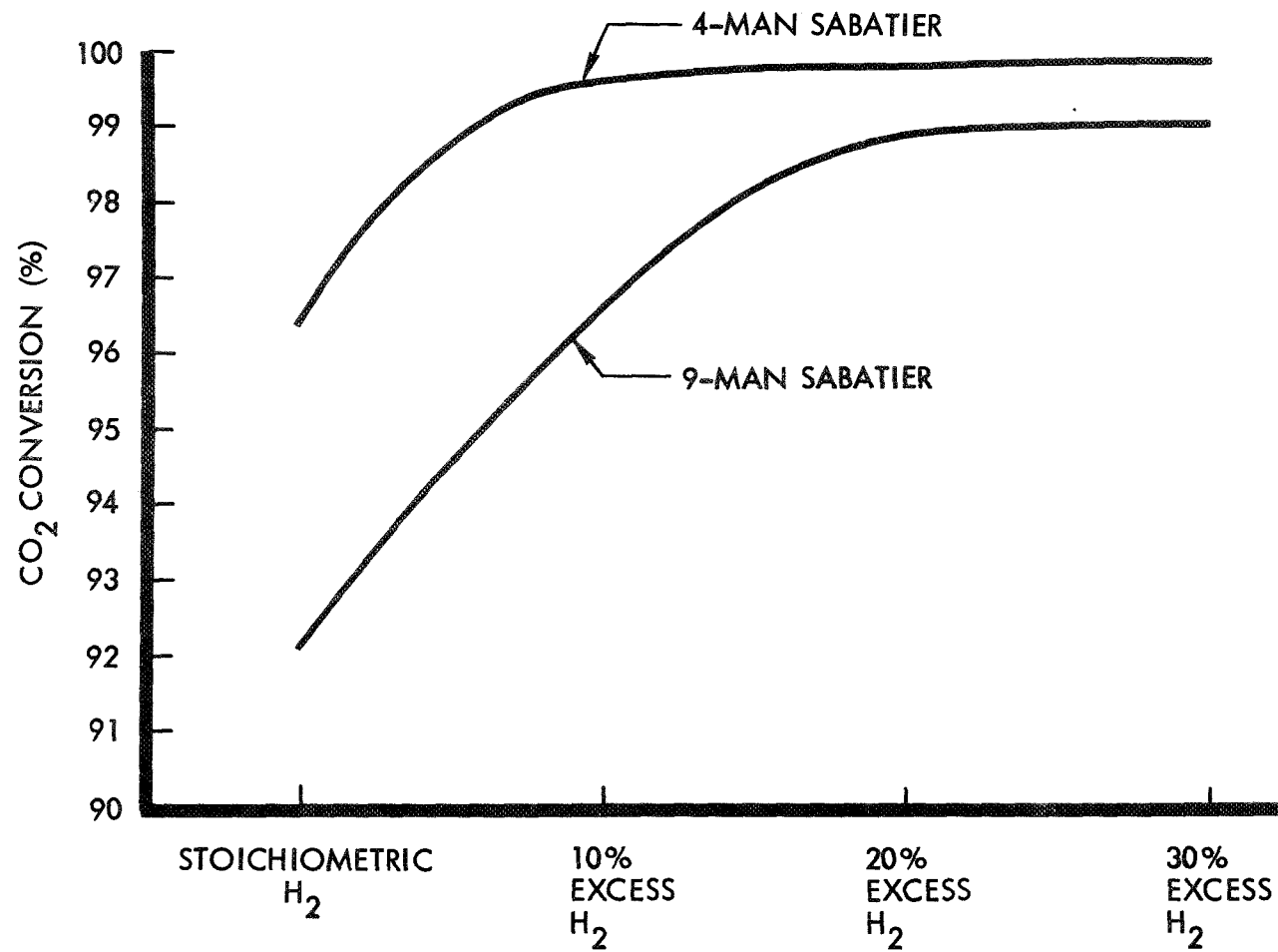
Figure 7.3: SABATIER REACTOR PERFORMANCE
