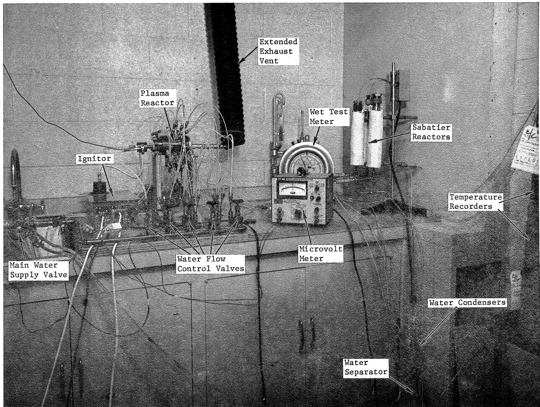
Figure 6.1: TEST SETUP
