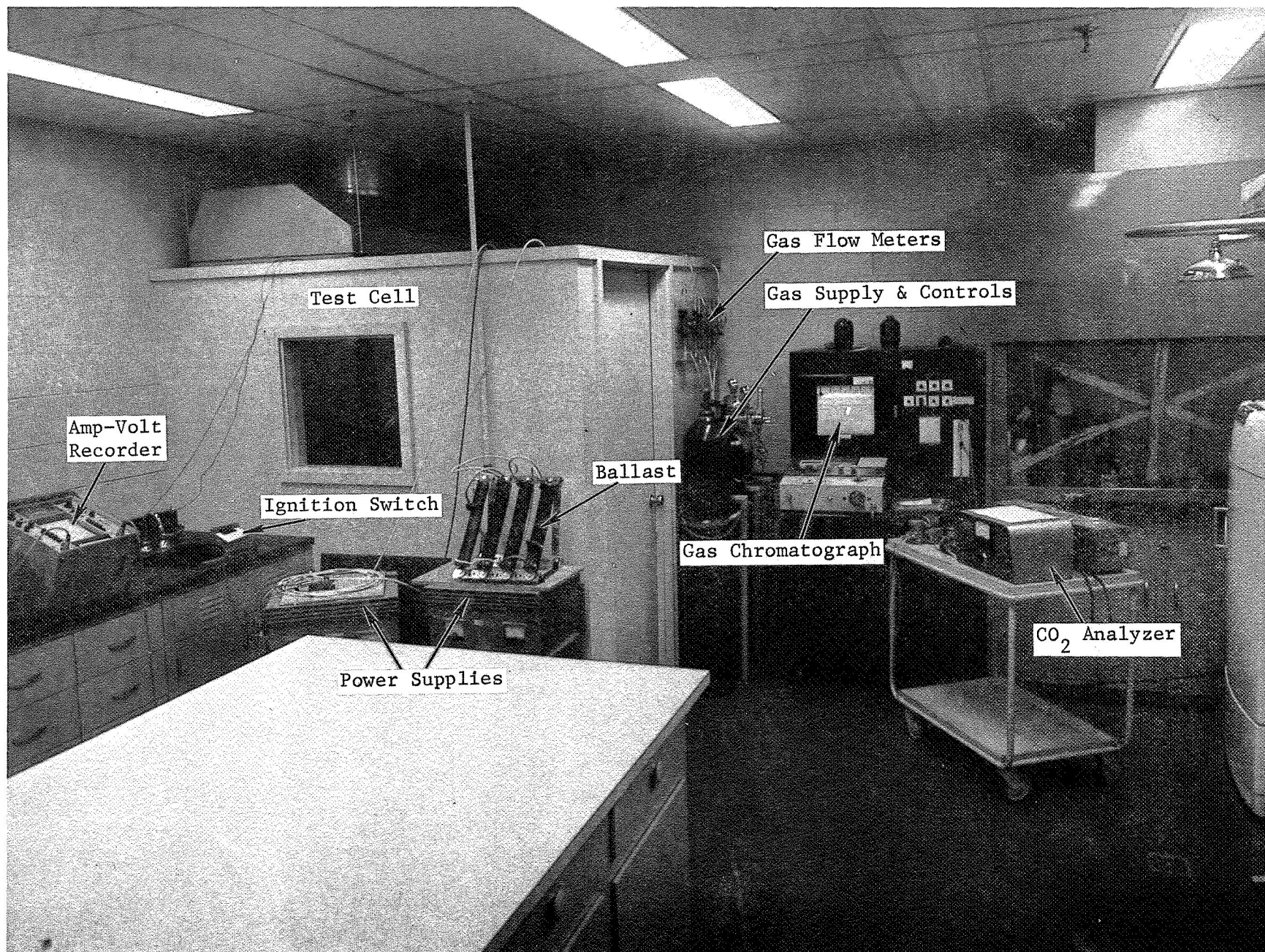
Figure 6.2: TEST SETUP
