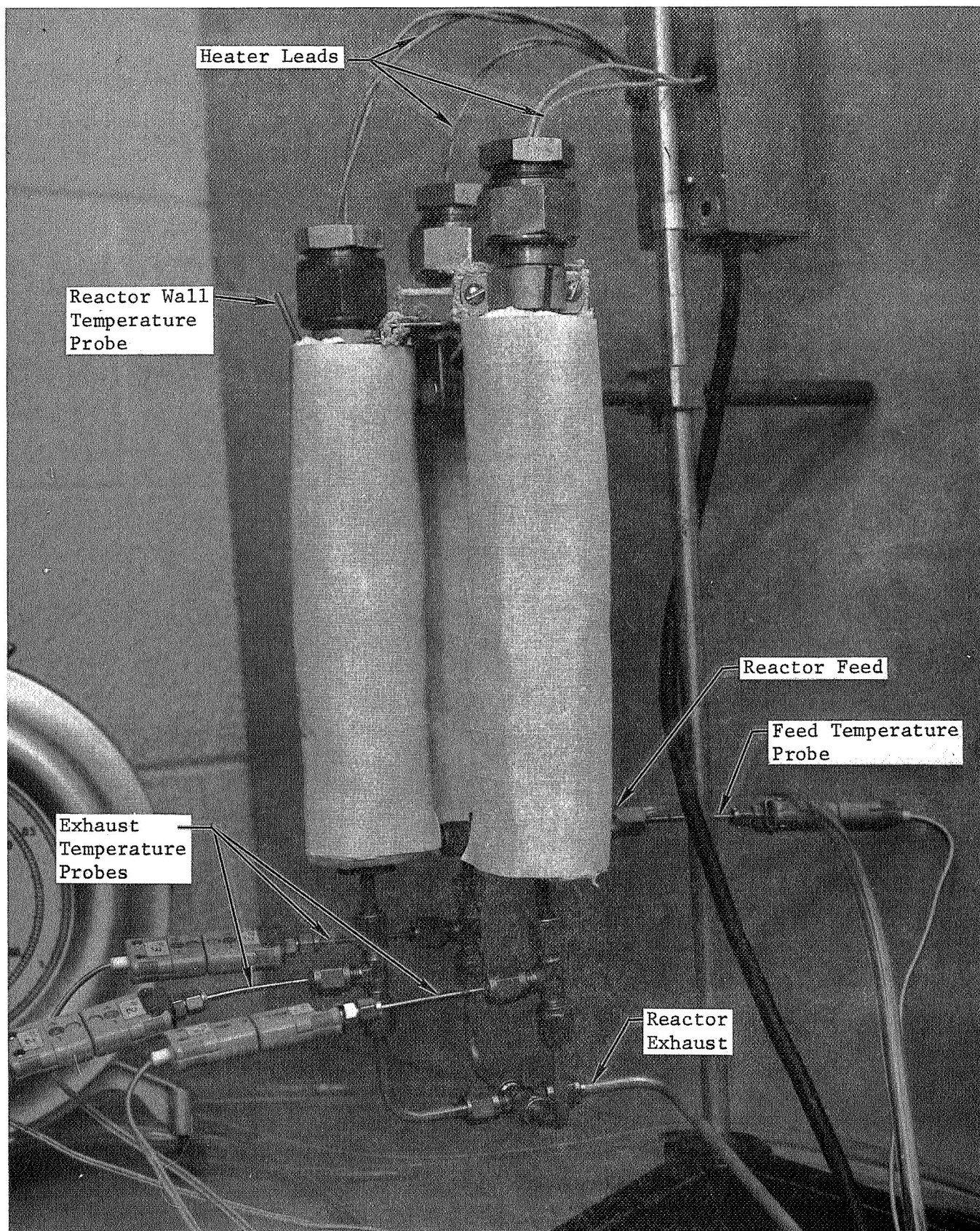
Figure 5.2: SABATIER REACTOR
