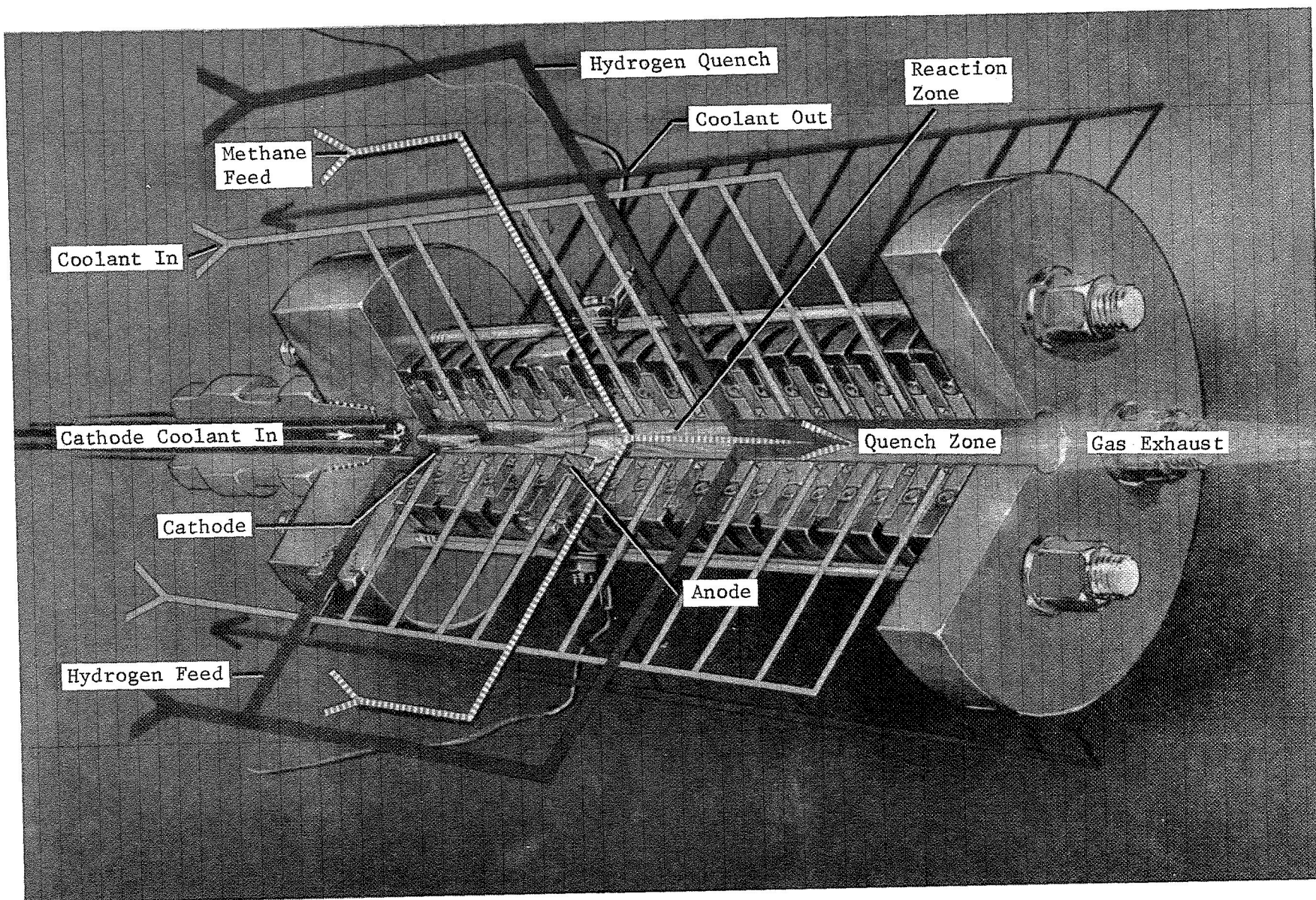
Figure 4.2: PLASMA REACTOR
