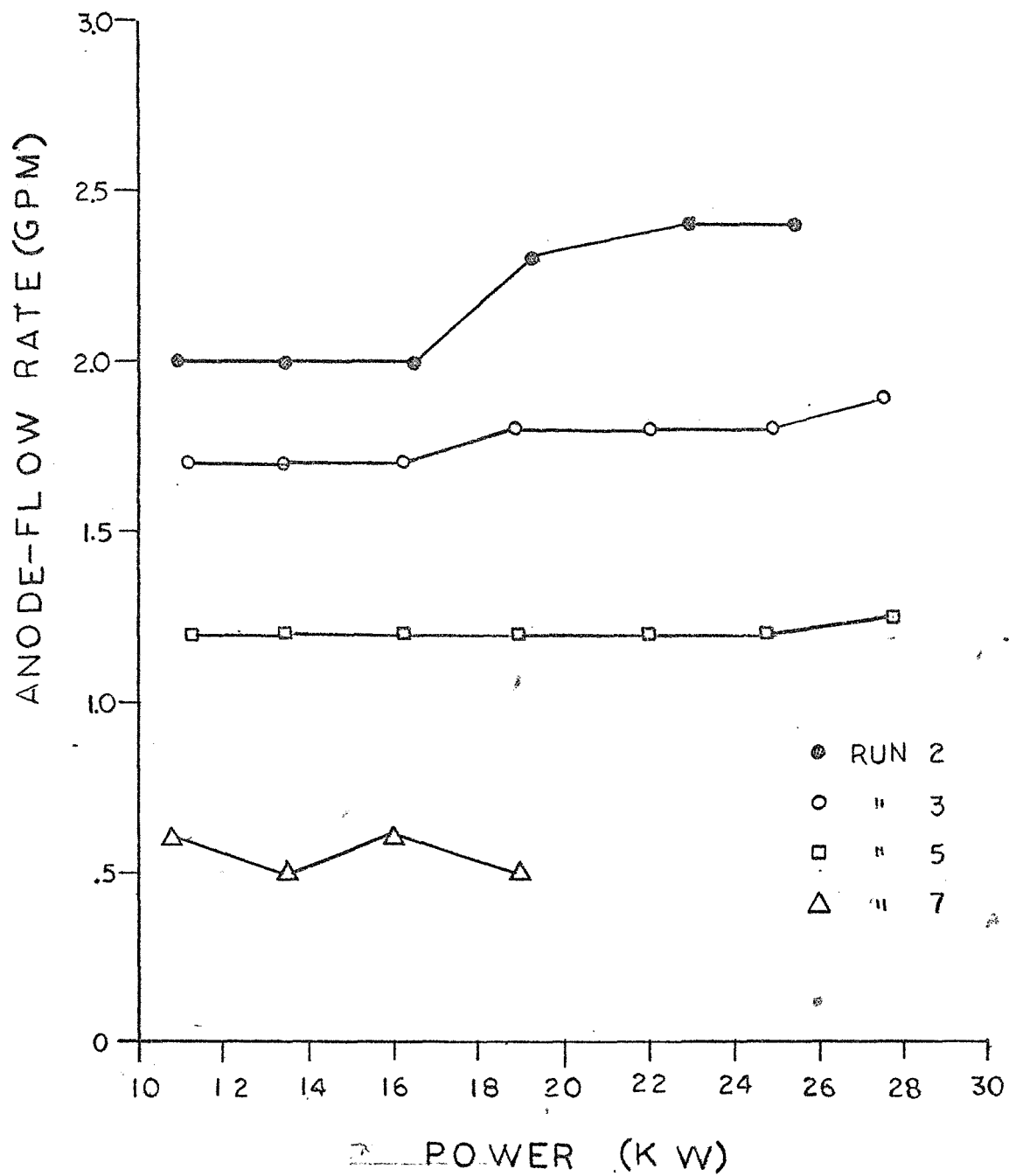
Figure B-5 Anode Flow Rate vs. Power Lamp #1 (1969)
