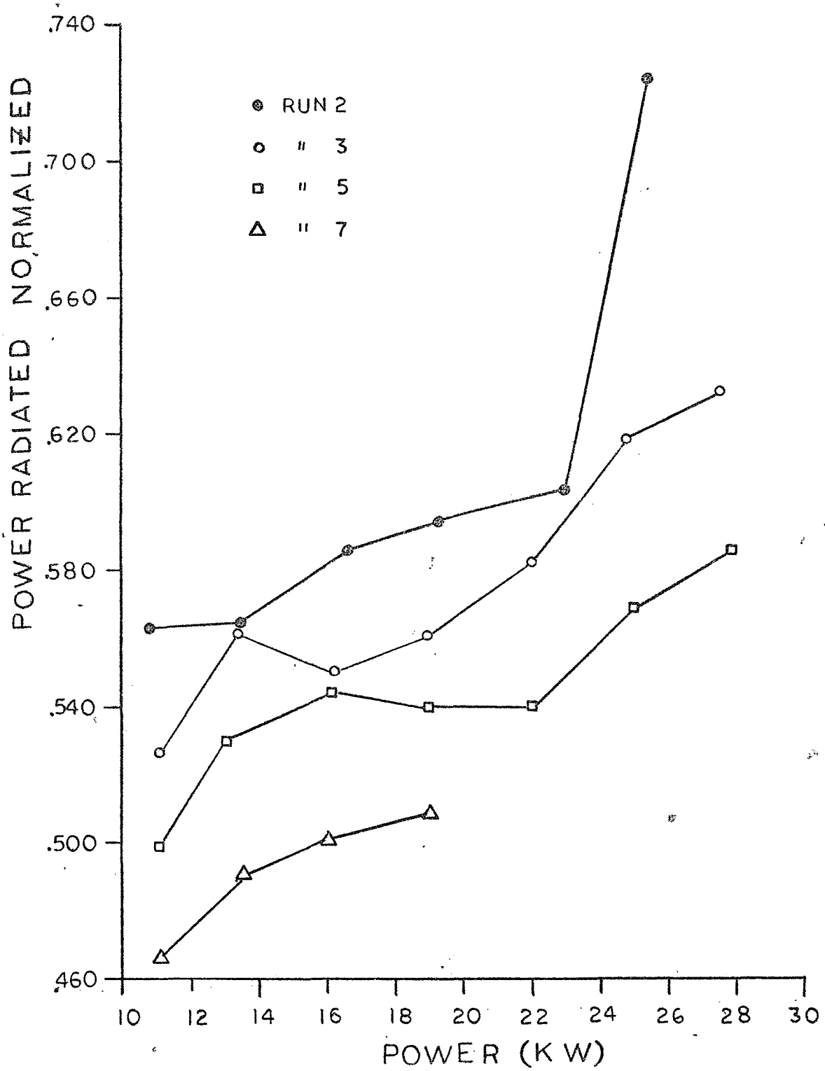
Figure B-10 Normalized Radiated Power versus Lamp Power Lamp #1 (1969)
