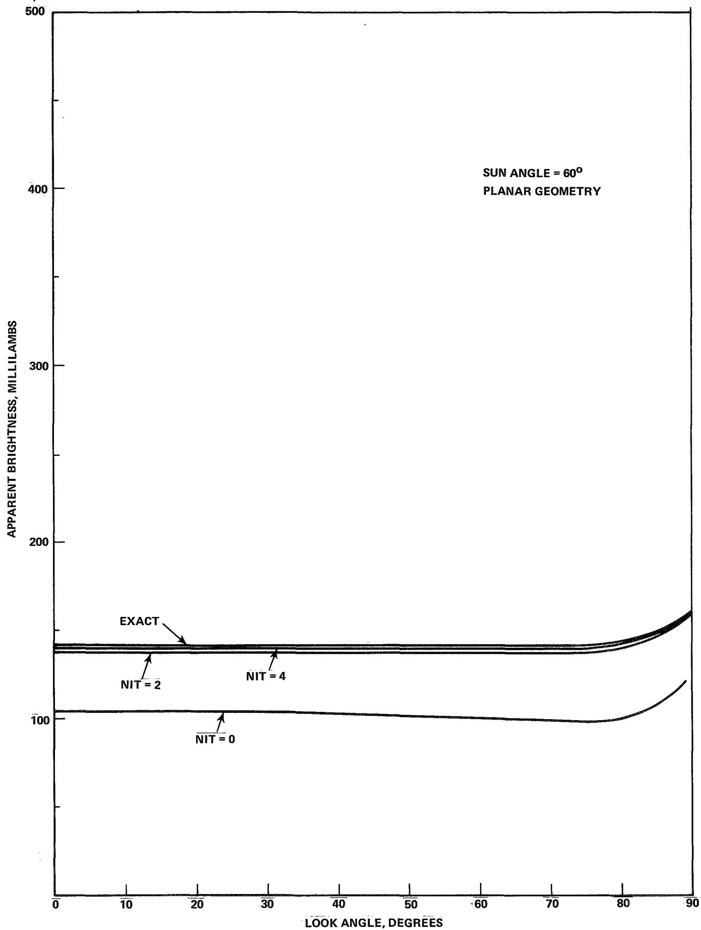
FIGURE 4 - ILLUSTRATION OF THE CONVERGENCE OF THE ITERATIVE CALCULATIONS FOR THE PLANAR HAZE. THE PARAMETER NIT IS THE NUMBER OF ITERATIONS.
