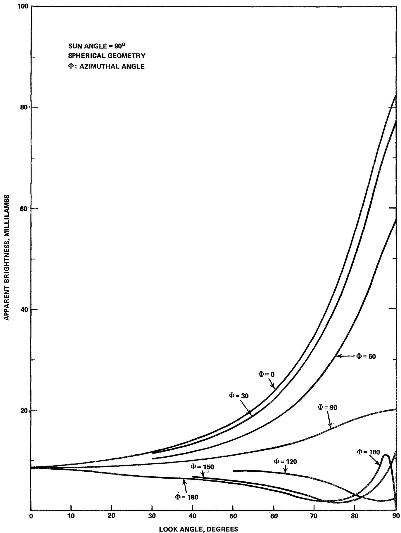
FIGURE 15 - APPARENT BRIGHTNESS FOR SEVERAL VALUES OF THE AZIMUTHAL ANGLE \Phi . THE VERTICAL SCALE HAS BEEN MAGNIFIED OVER THAT USED IN PREVIOUS FIGURES.
