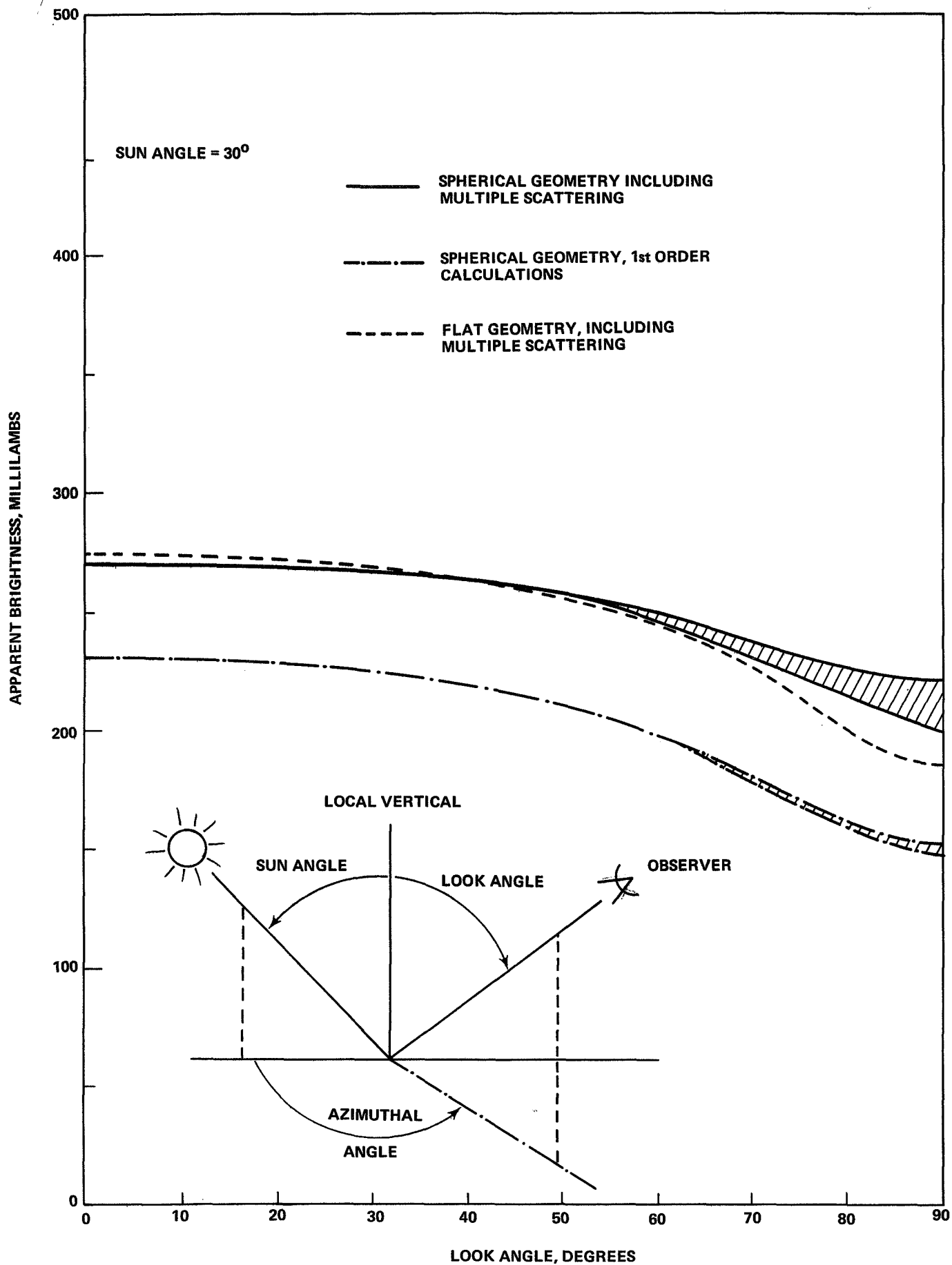
FIGURE 12 - APPARENT BRIGHTNESS FOR A SUN ANGLE OF 30°, CALCULATED BY SEVERAL DIFFERENT TECHNIQUES. THE CROSS-HATCHED AREAS INDICATE THE RANGE OF VARIATION IN THE BRIGHTNESS DUE TO CHANGE IN THE AZIMUTHAL ANGLE.
