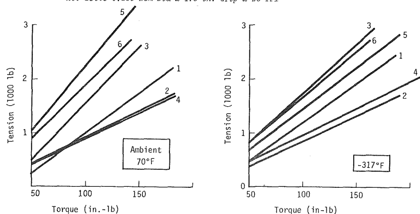
Figure IV-38 Torque vs Induced Load ( 10^{-6} Torr Vacuum -317^\circ\text{F} )
