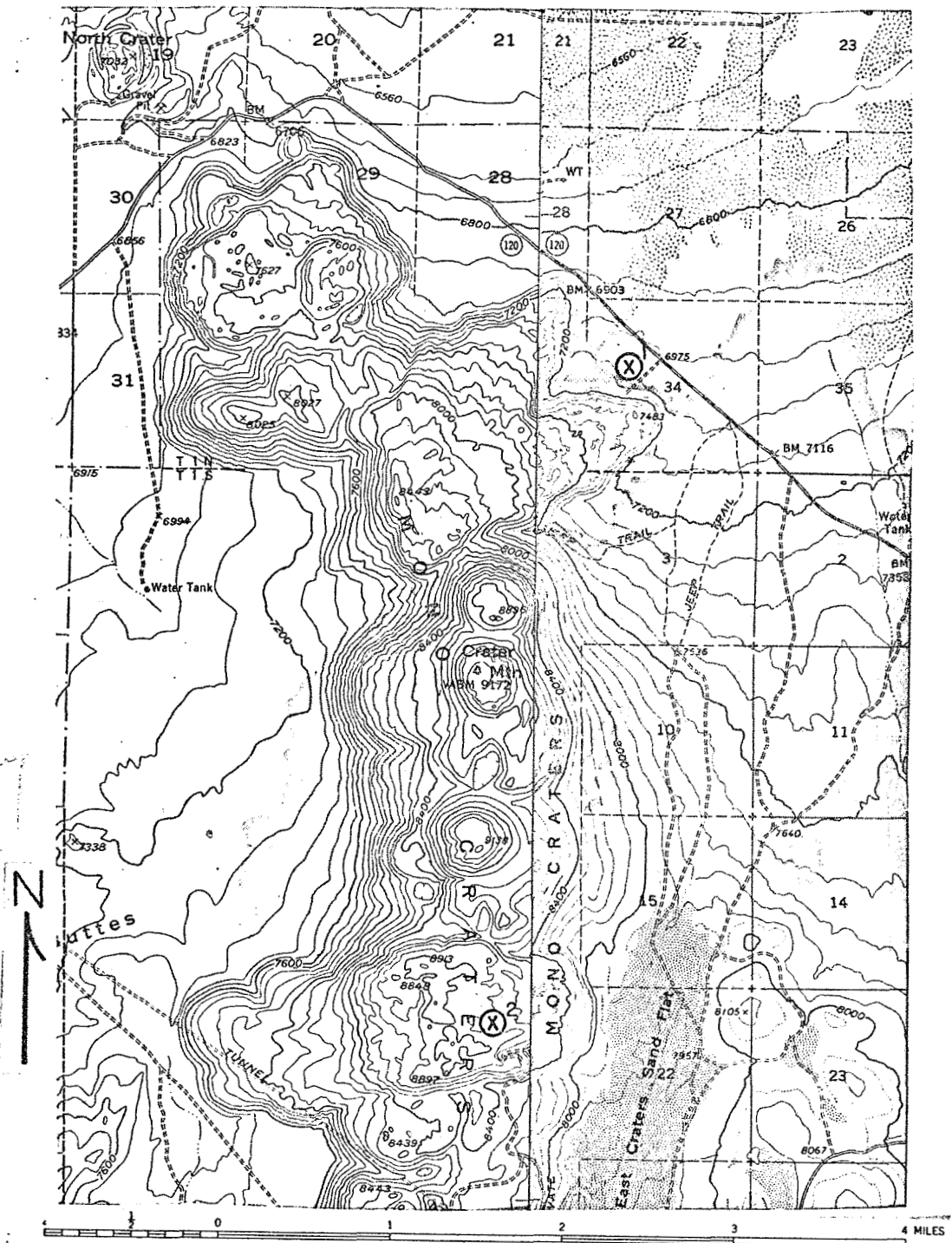
Fig. 4. (Location map). This topographic map of Mono Craters, California shows the location of the Lapilli Surface \otimes^1 and the Pumice Surface \otimes^2 . The map was constructed from the east-central portion of the Mono Craters, California 15-minute topographic quadrangle and the west-central portion of the Cowtrack Mountain, California 15-minute topographic quadrangle.
