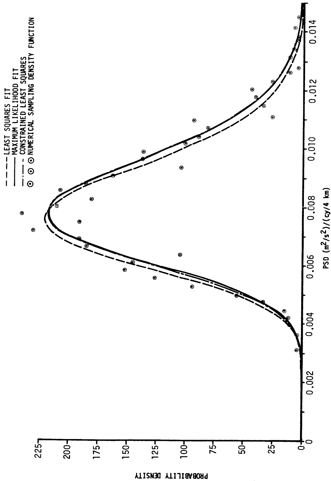
FIGURE 3-8. COMPARISON OF NUMERICAL AND THEORETICAL SAMPLING DISTRIBUTIONS ON THE MEAN AT WAVE NUMBER 10 FOR SAMPLE SIZE 20
