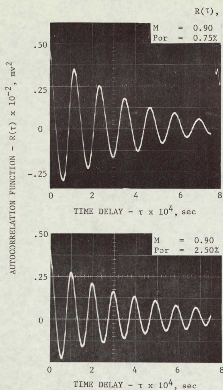
FIGURE 6.13. EFFECTS OF POROSITY ON TRANSONIC TEST SECTION FLUCTUATIONS (TRANSDUCER B 3 , P 0 = 14.5 psi, CONFIGURATION T 1 , SONIC BLOCKS)
