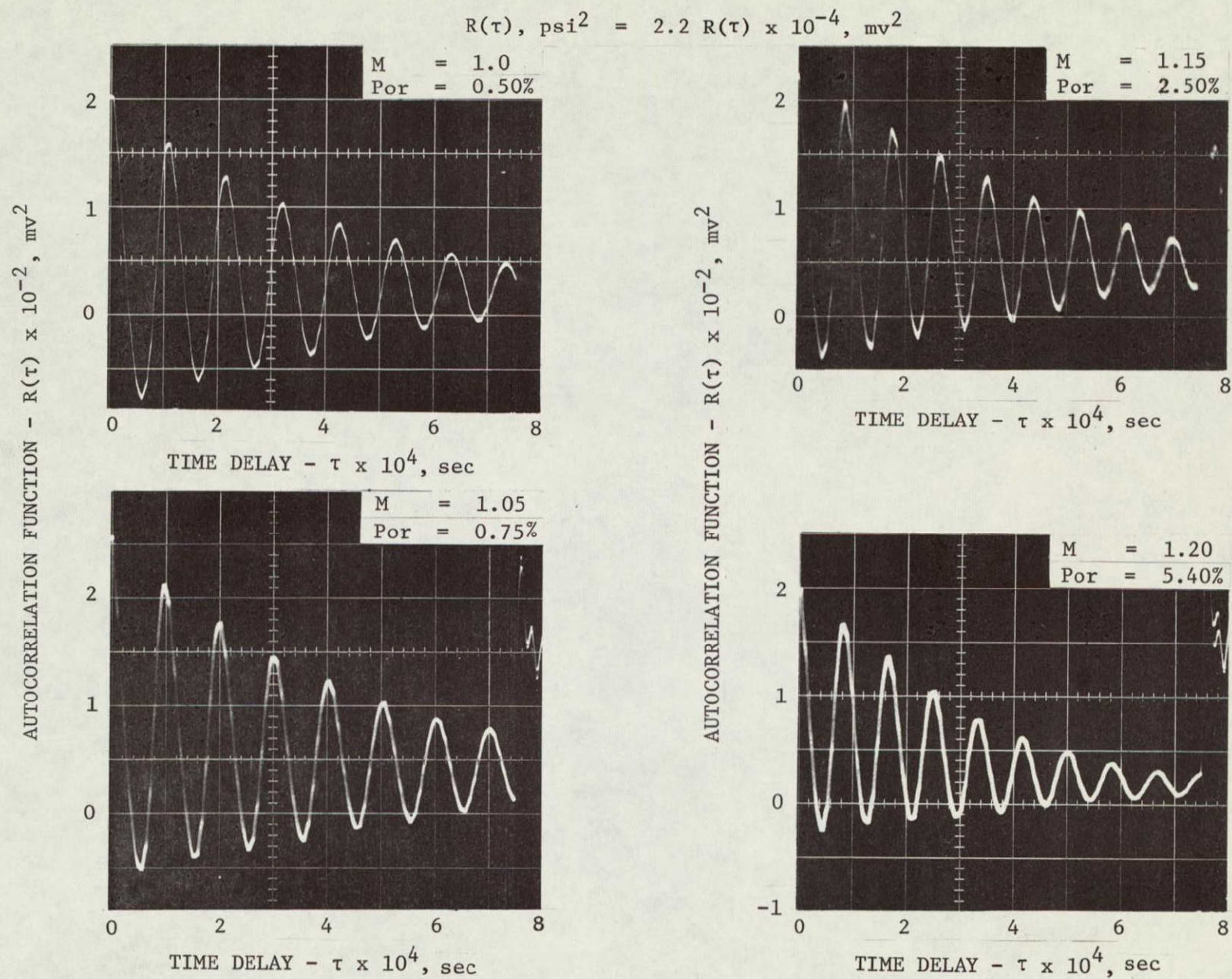
FIGURE 6.10. EFFECTS OF MACH NUMBER ON TRANSONIC TEST SECTION FLUCTUATIONS (TRANSDUCER B 3 , P 0 = 22.0 psi, CONFIGURATION T 1 , SONIC BLOCKS)
