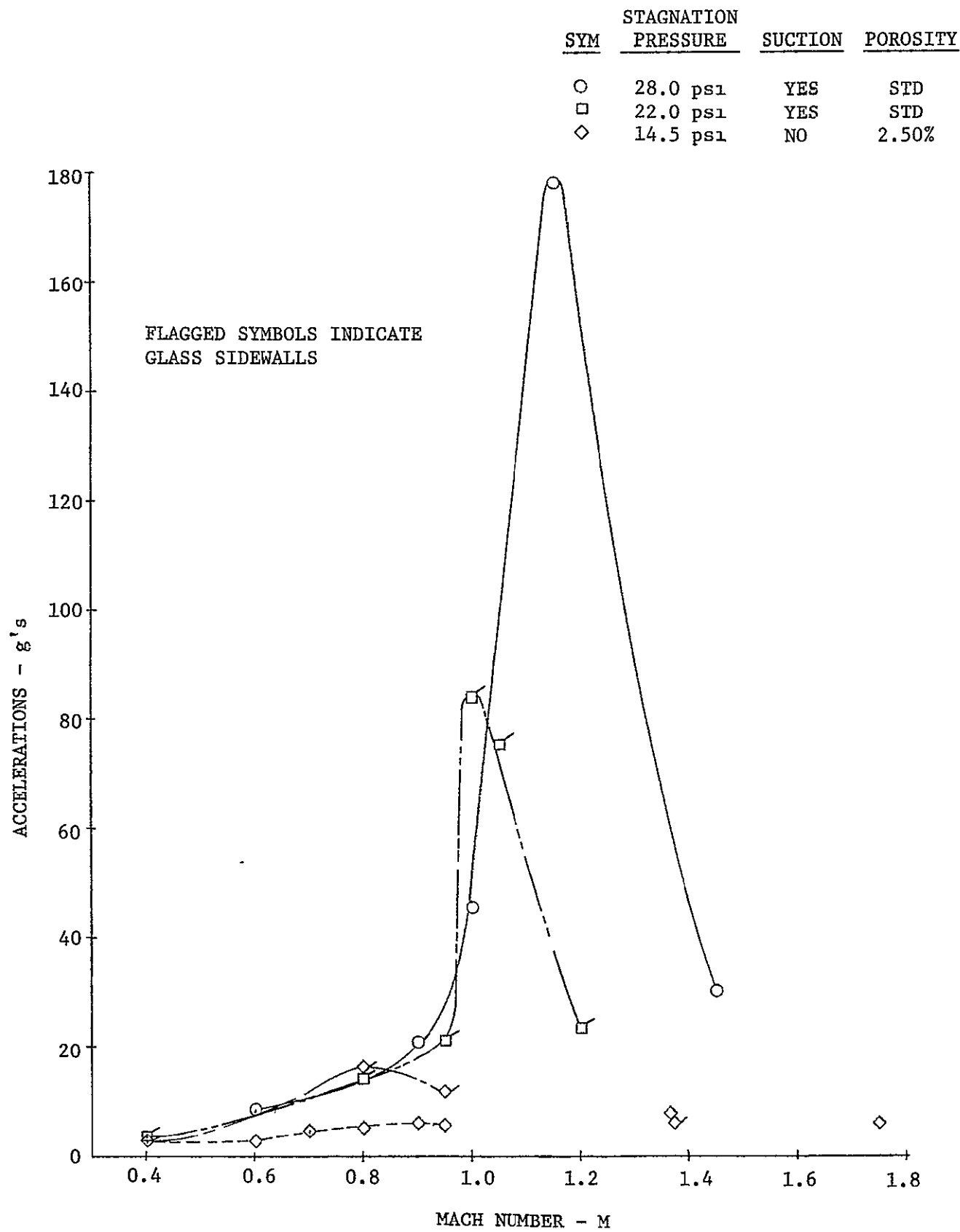
FIGURE 6.6. VIBRATION LEVEL MEASURED ON UPPER POROUS WALL
