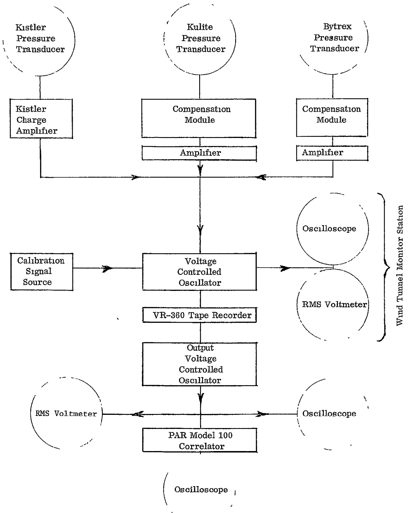
FIGURE 3.2 INSTRUMENTATION BLOCK DIAGRAM FOR MSFC 14 IN. WIND TUNNEL CALIBRATION
