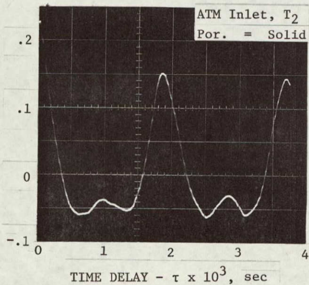
FIGURE 6.16. EFFECTS OF UPSTREAM TURBULENCE ON DIFFUSER FLUCTUATIONS (TRANSDUCER K_6 , M = 0.9 , SONIC BLOCKS)
