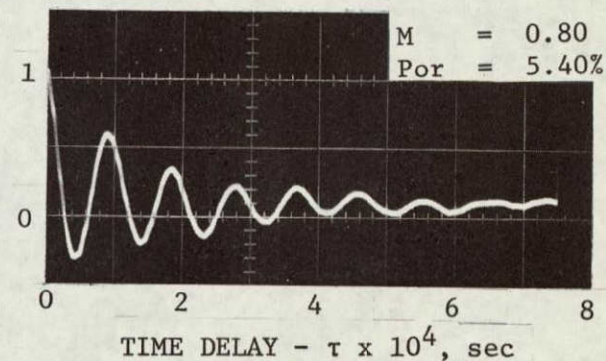
FIGURE 6.10. EFFECTS OF MACH NUMBER ON TRANSONIC TEST SECTION FLUCTUATIONS (TRANSDUCER B_3 , P_o = 22.0 \text{ psi} , CONFIGURATION T_1 , SONIC BLOCKS)
