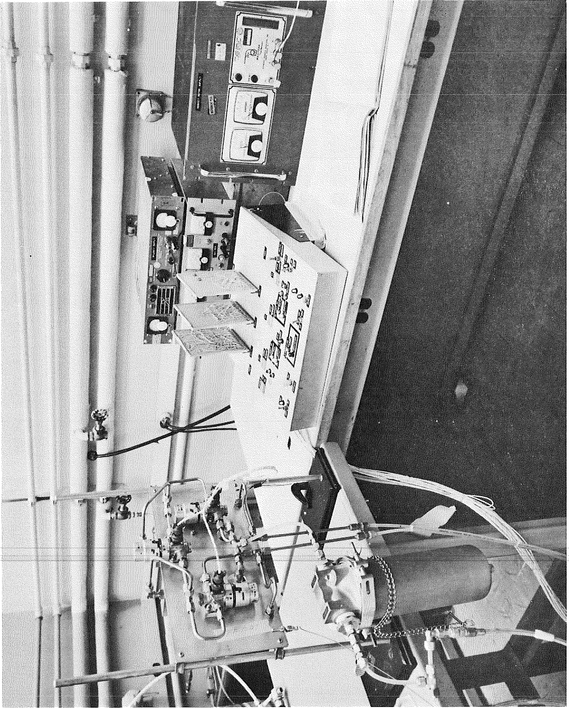
Figure 58 Water System Bacteria Filter and Electronic Controls
