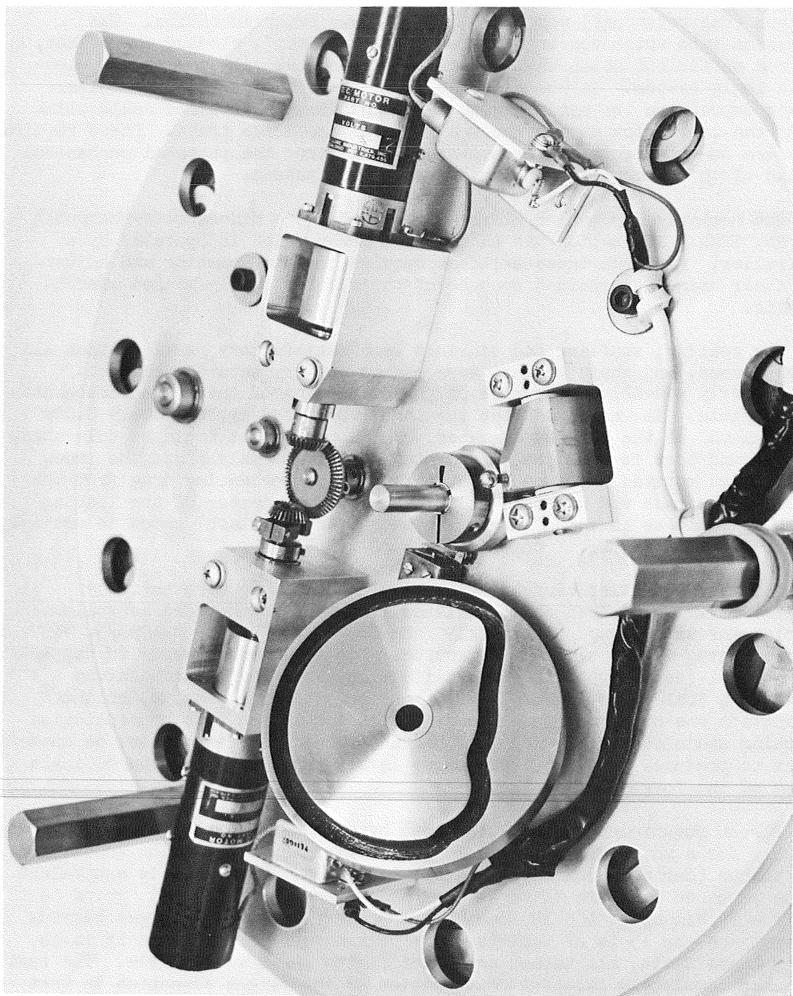
Figure 40 Bottom View of Feeder Mechanism Partly Disassembled
