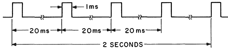
Fig. 5 Waveform Specification
