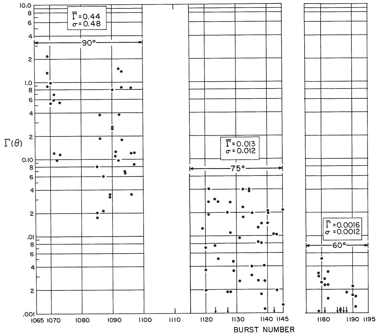
Fig. 26a Scattering Coefficient Measurements as a Function of Time Carson Sink, Nevada (Desert Area)
