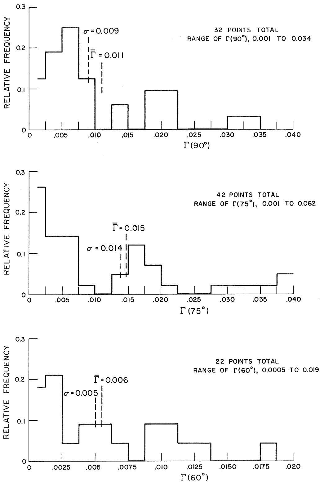
Fig. 22b Histograms of Scattering Coefficient Measurements Malad, Idaho (Mountains)
