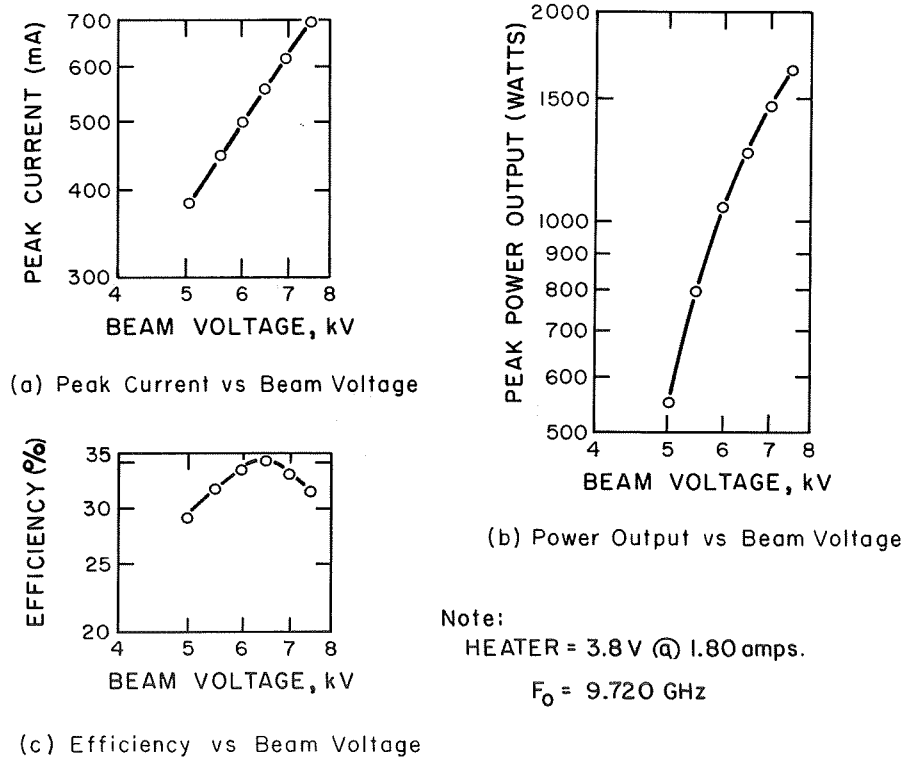
Fig. 7 Characteristic Curves of the VA-909B Klystron
