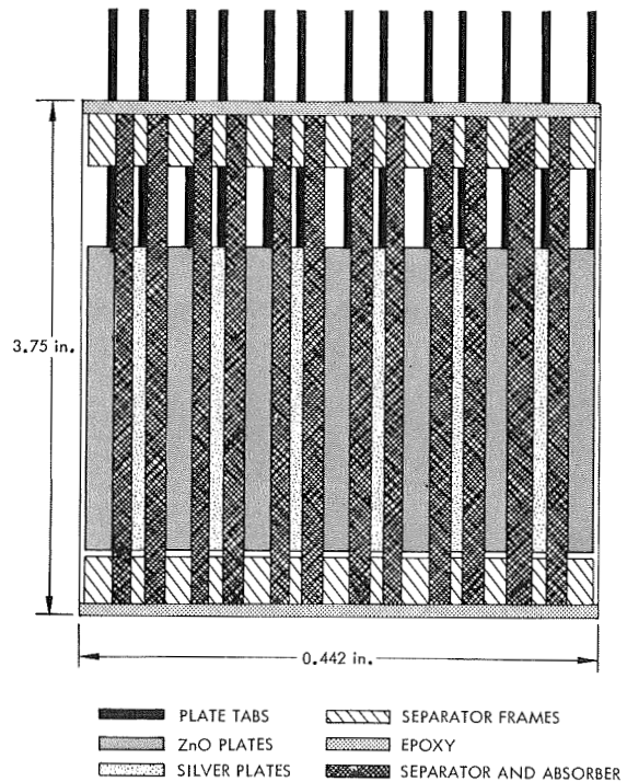
Figure 3. Cross Section of Cell Core Assembly
