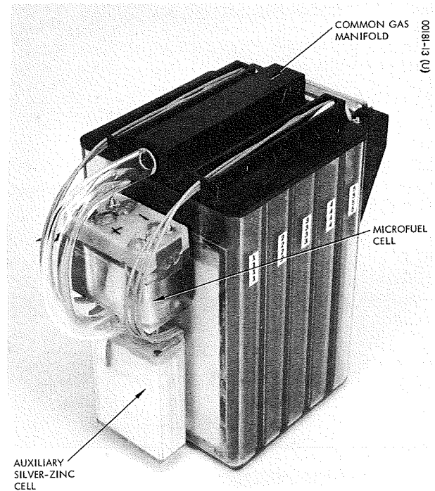
Figure 11. Three-Quarter View of Engineering Model Battery Assembly (Photo A24848)
