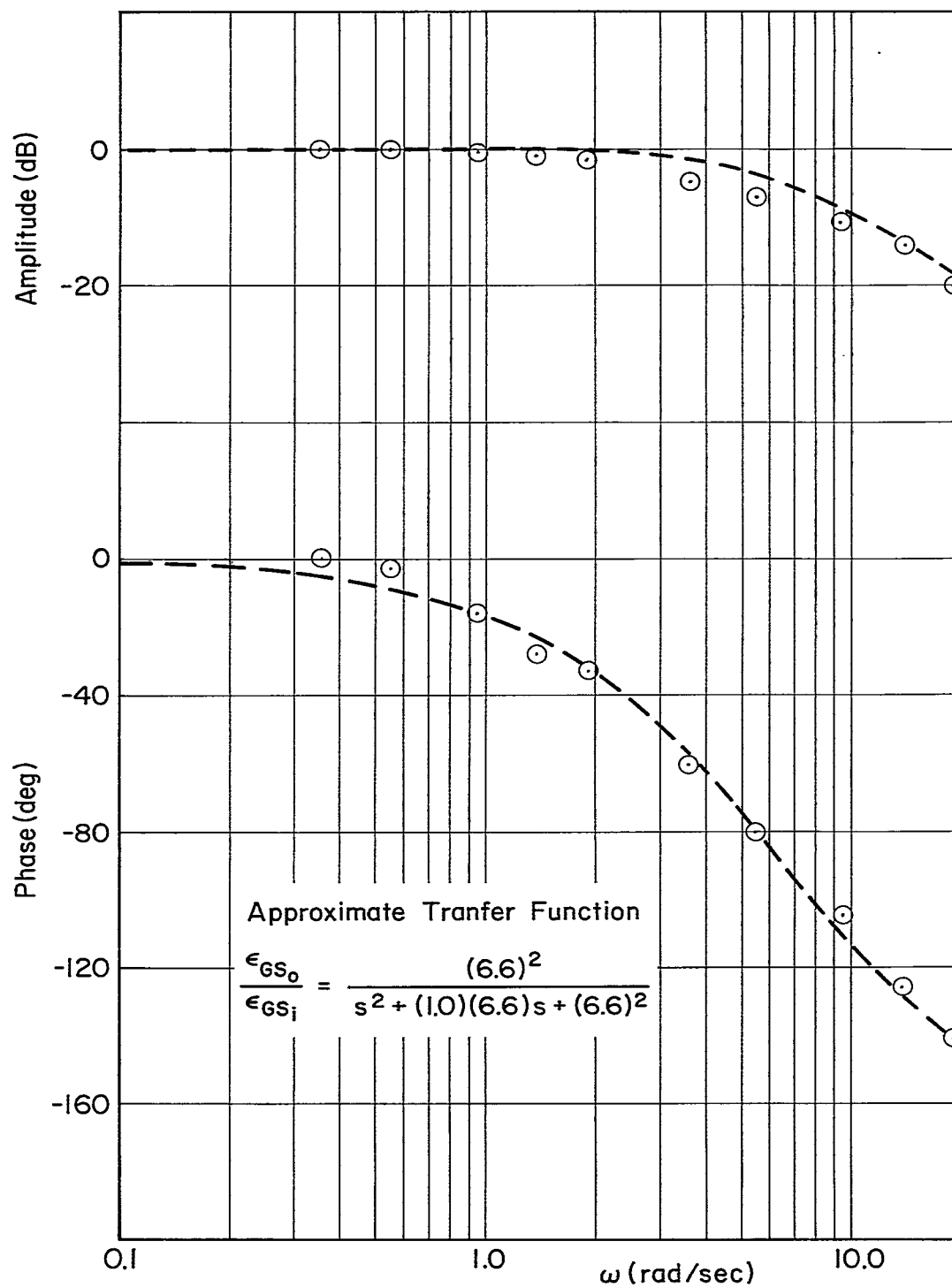
(b) Glide Slope Instrument Frequency Response
