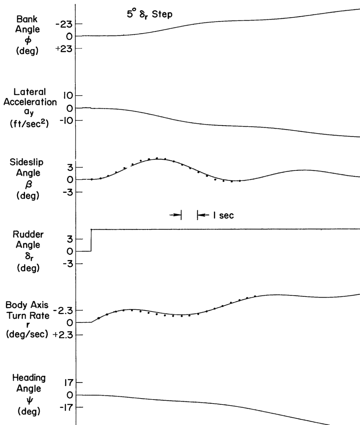
Figure B-3. Open-Loop Transient Response to 5^\circ Rudder Step Input
