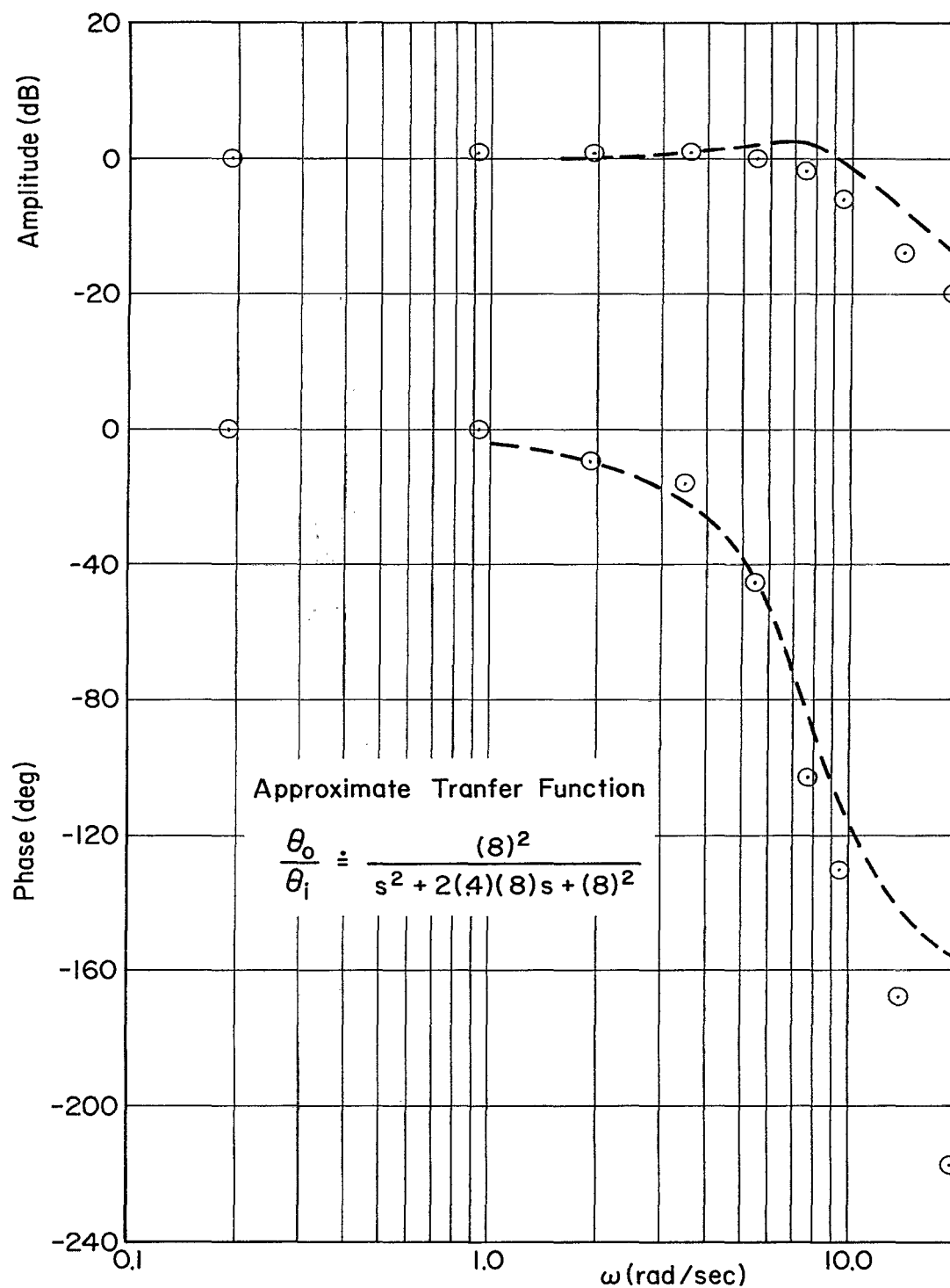
(a) Pitch Angle Instrument Frequency Response Figure B-7. Primary Longitudinal Instruments
