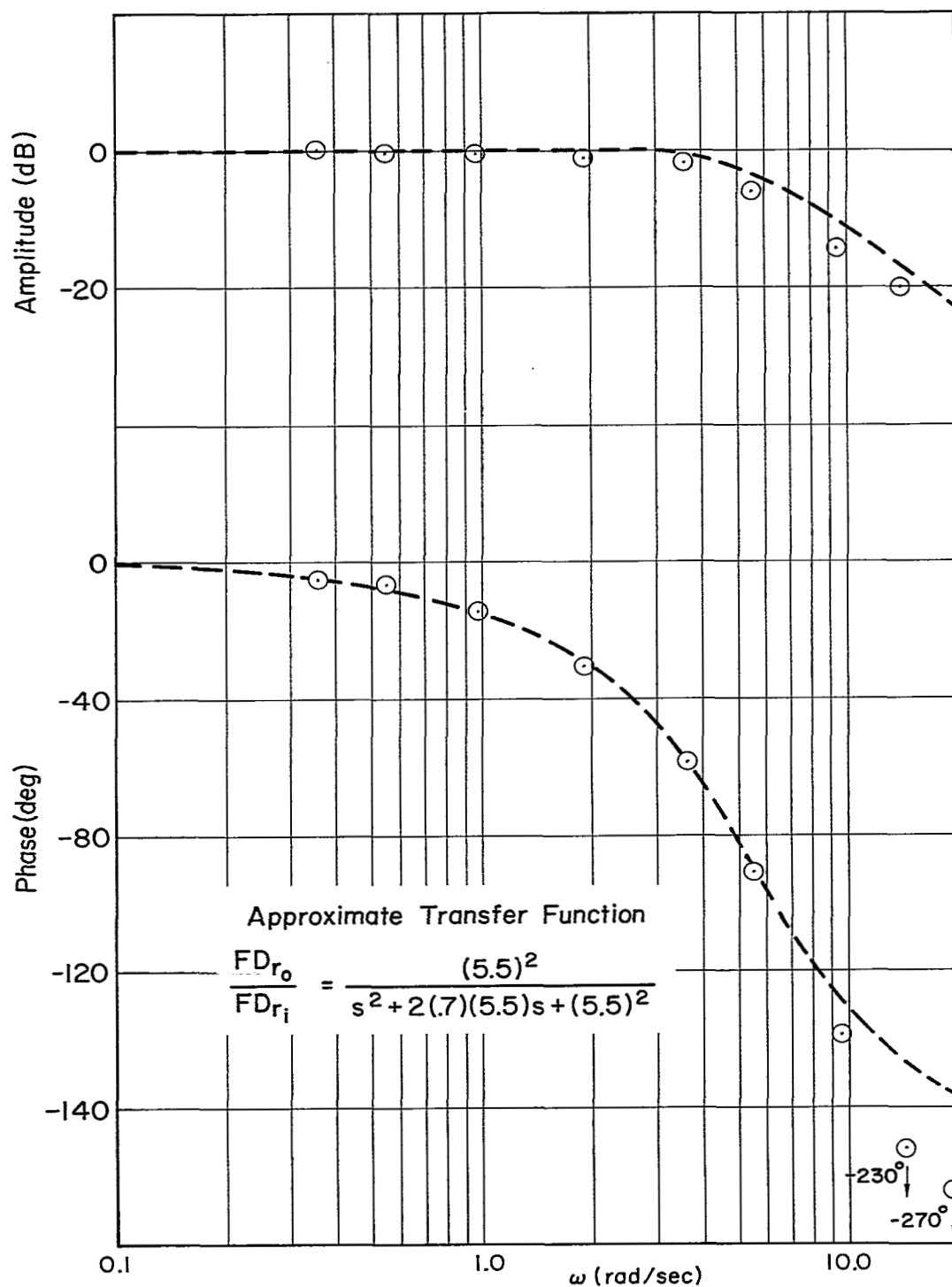
(c) Lateral Flight Director Instrument Frequency Response
