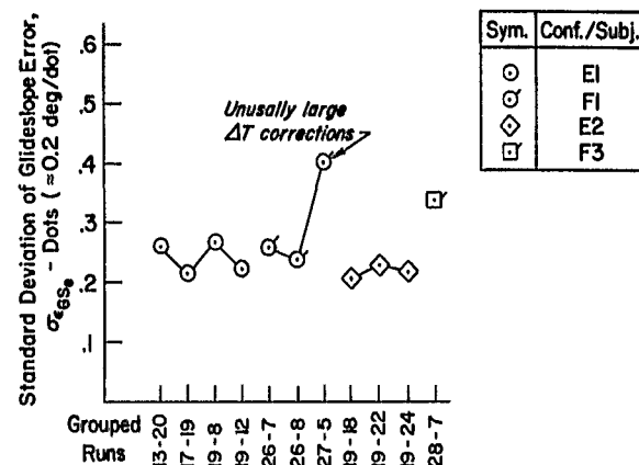
Figure 11. Glide Slope Performance with Flight Director Configurations
