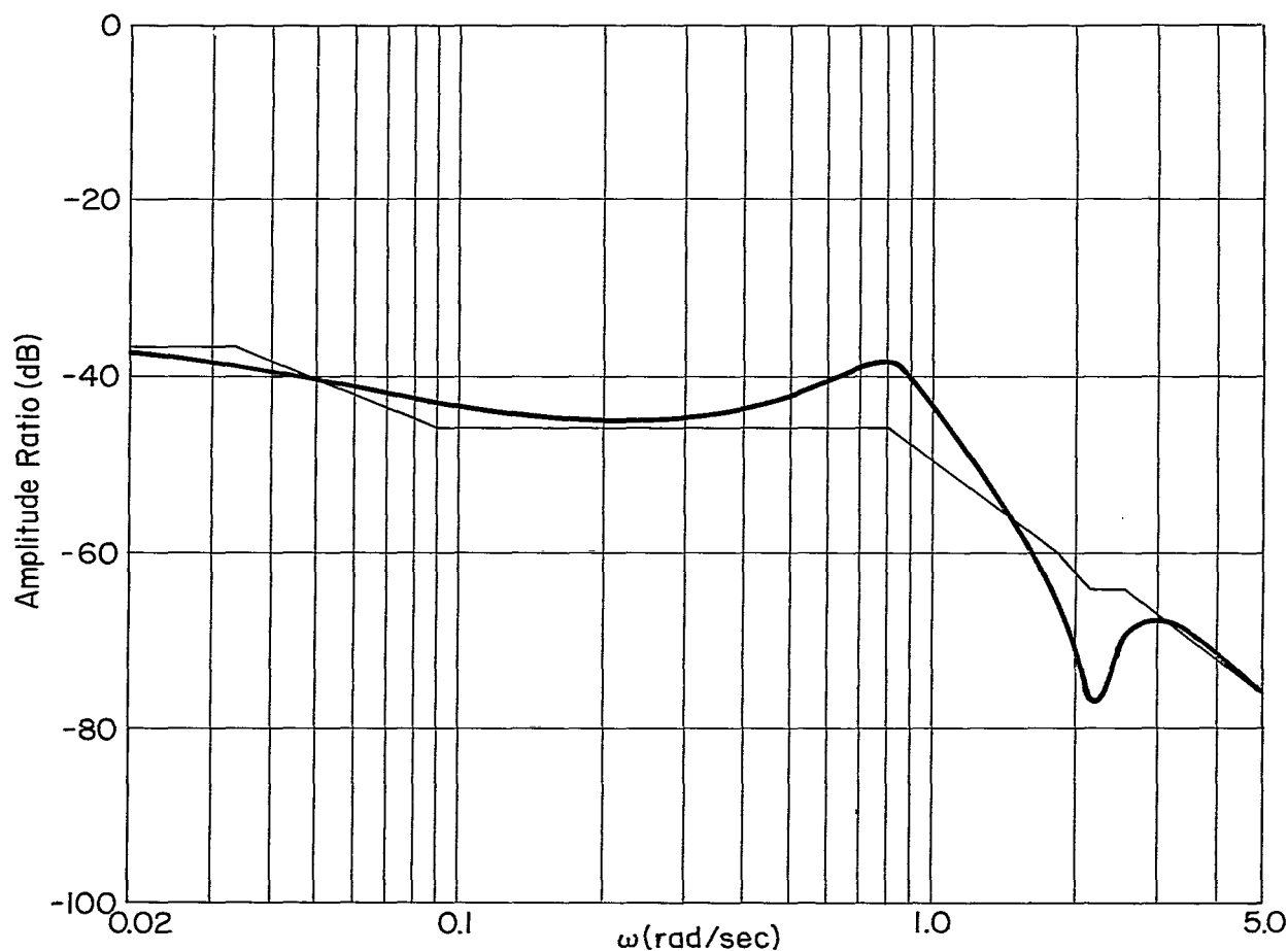
Figure C-2. Amplitude Ratio of \theta/w_g with \theta \rightarrow \delta_e and \epsilon_{GS} \rightarrow \delta_e Loops Closed
