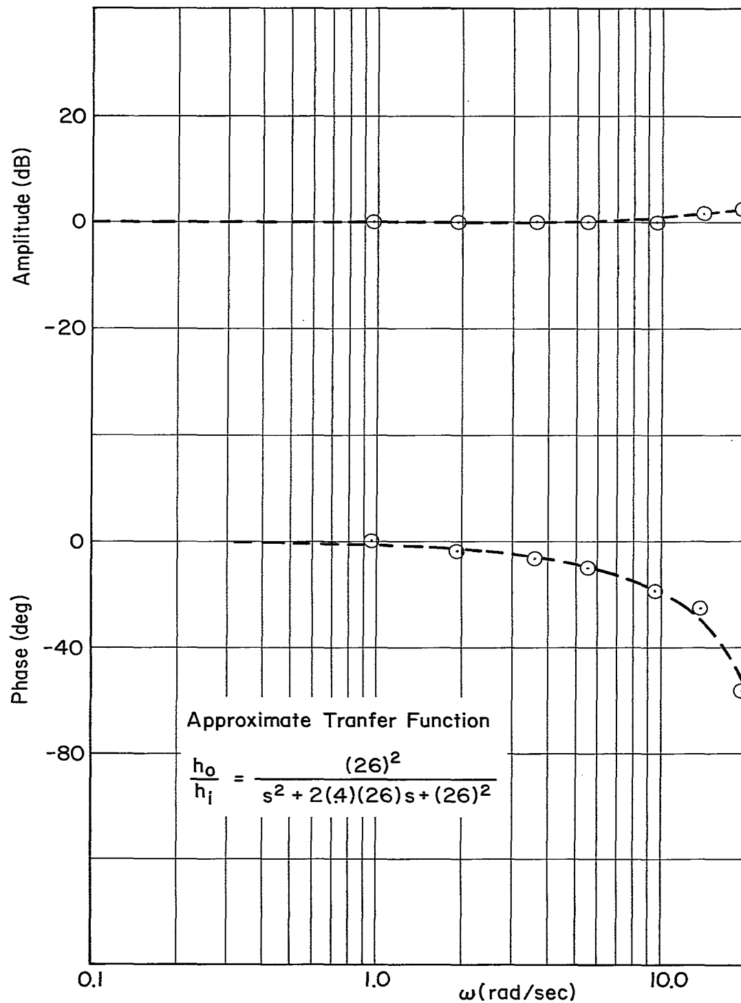
(b) Altimeter Frequency Response Figure B-9 (Continued)
