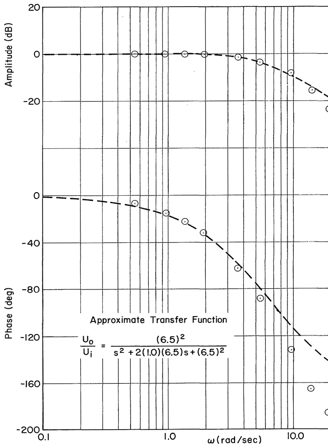
(c) Airspeed Instrument Frequency Response
