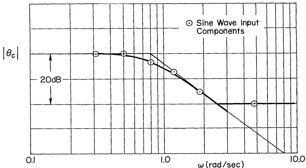
Figure C-3. Power Spectrum of Pitch Angle Forcing Function
