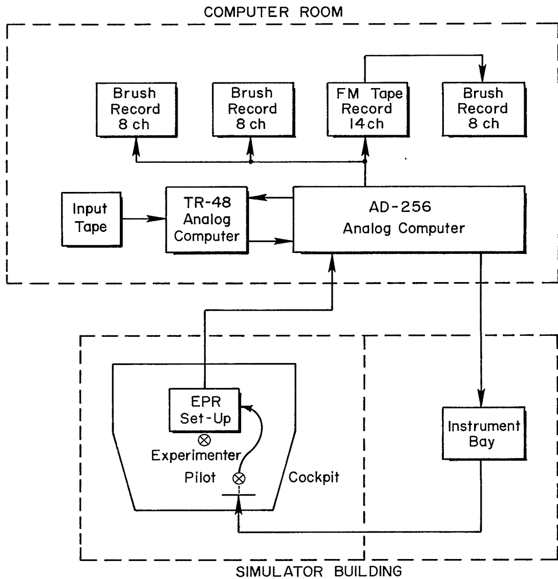
Figure 2. Topological Layout of Equipment
