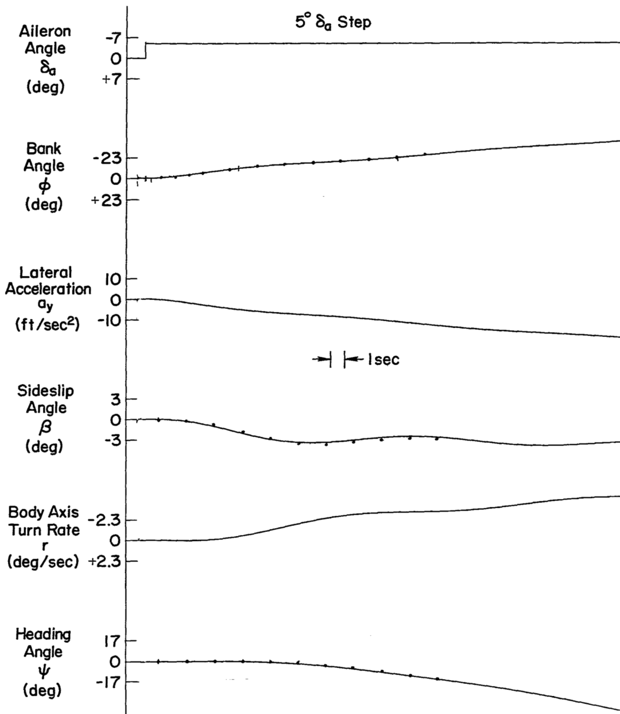
Figure B-2. Open-Loop Transient Response to 5^\circ Aileron Step Input
