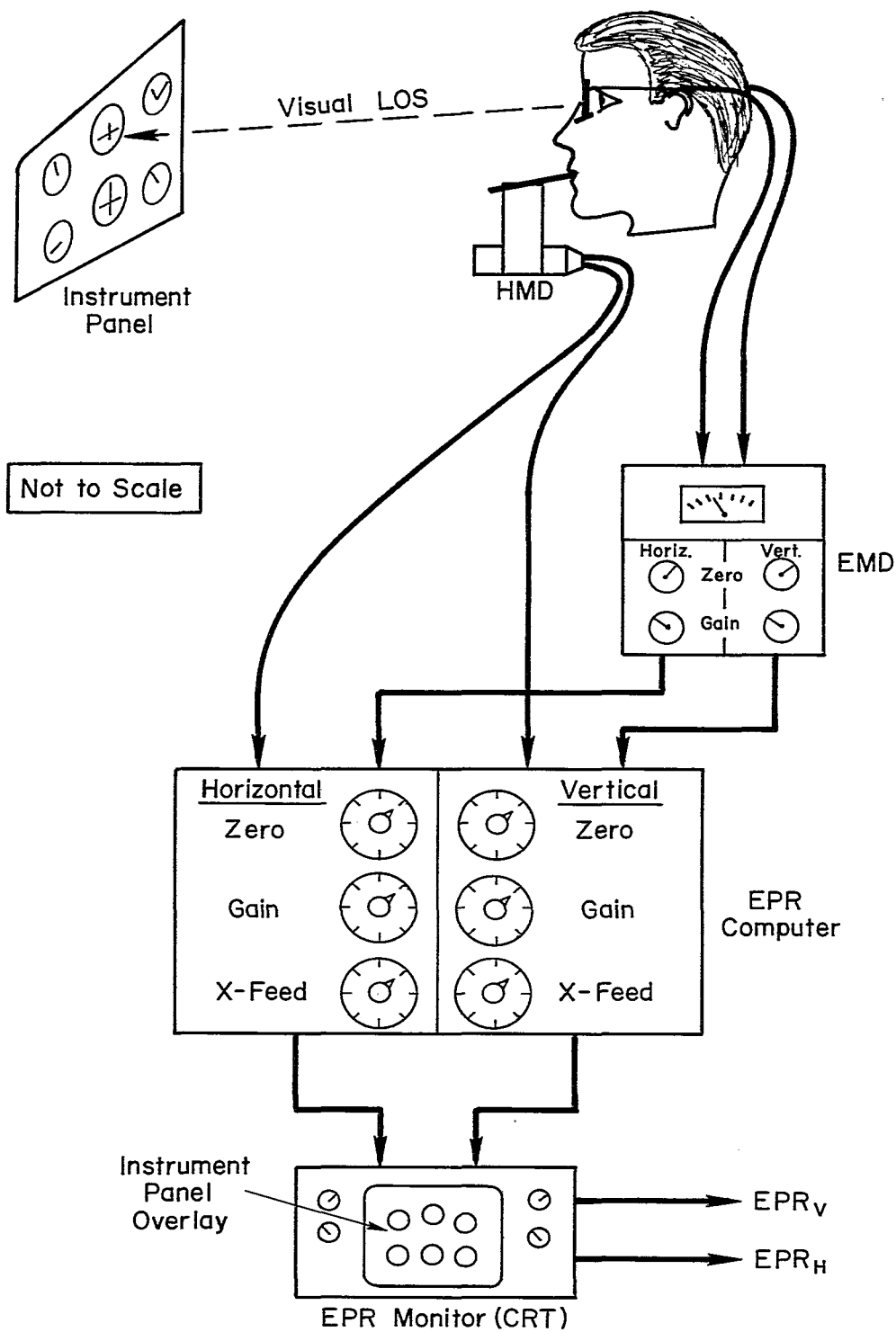
Figure A-2. EPR System Components
