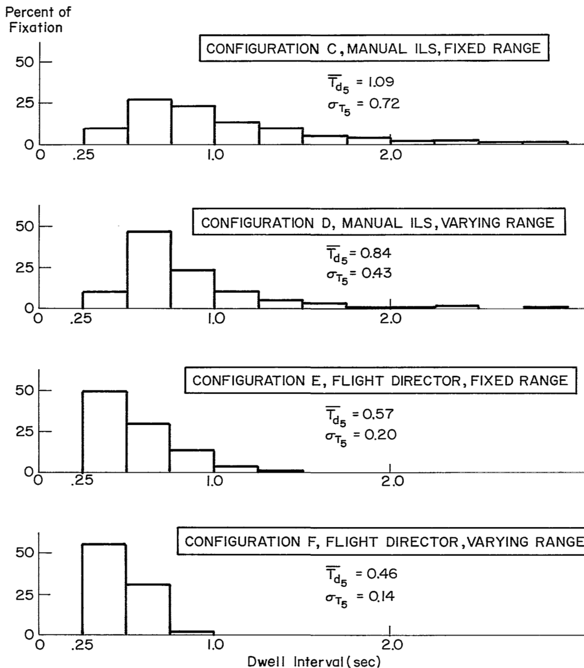
Figure 8. HSI/GSD Instrument Dwell Times for Pilot 1
