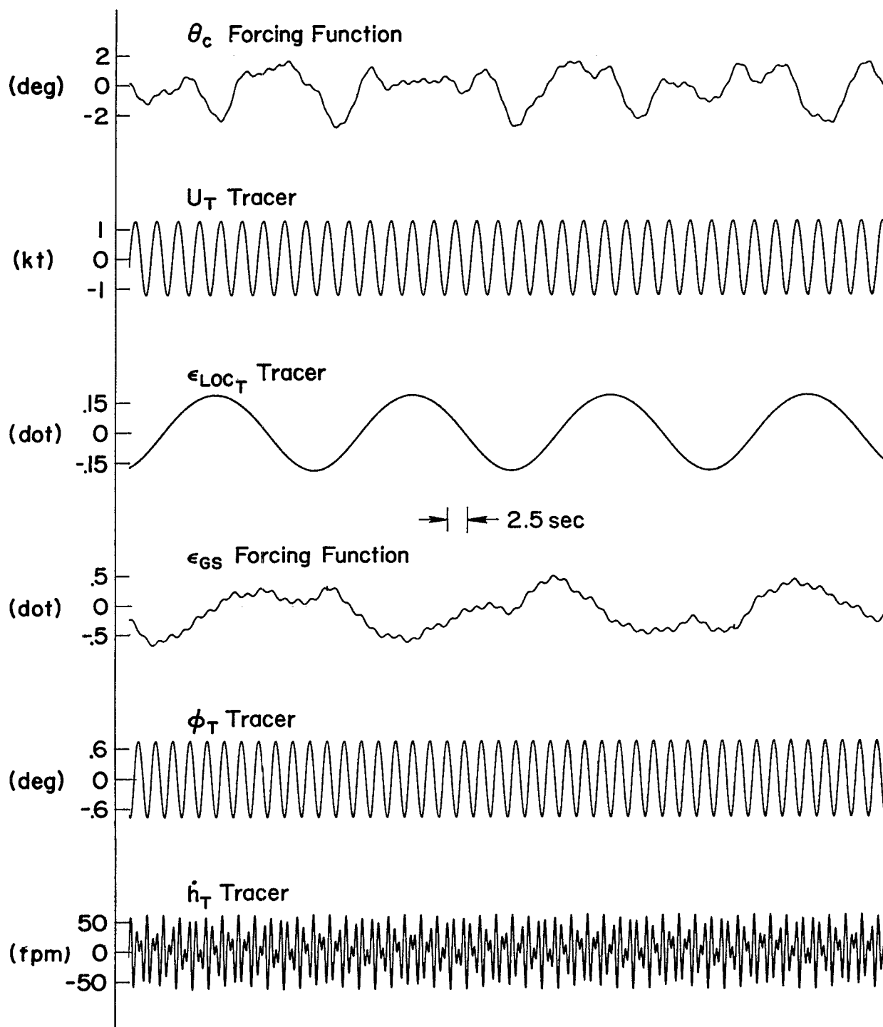
Figure C-5. Sample of Forcing Function and Tracers
