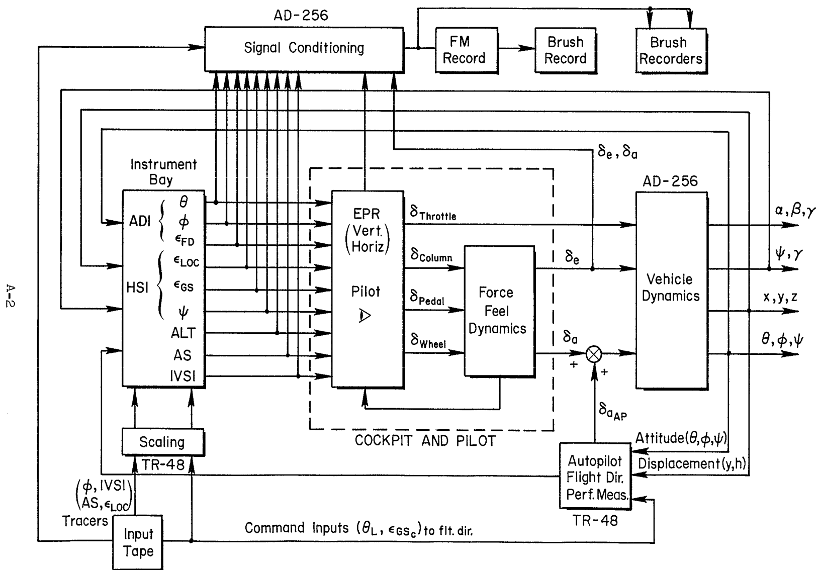
Figure A-1. Signal Flow Diagram and Equipment Functions
