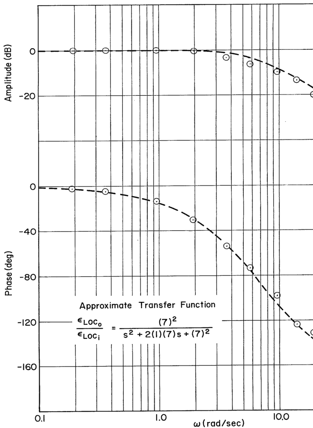
(b) Localizer Instrument Frequency Response
