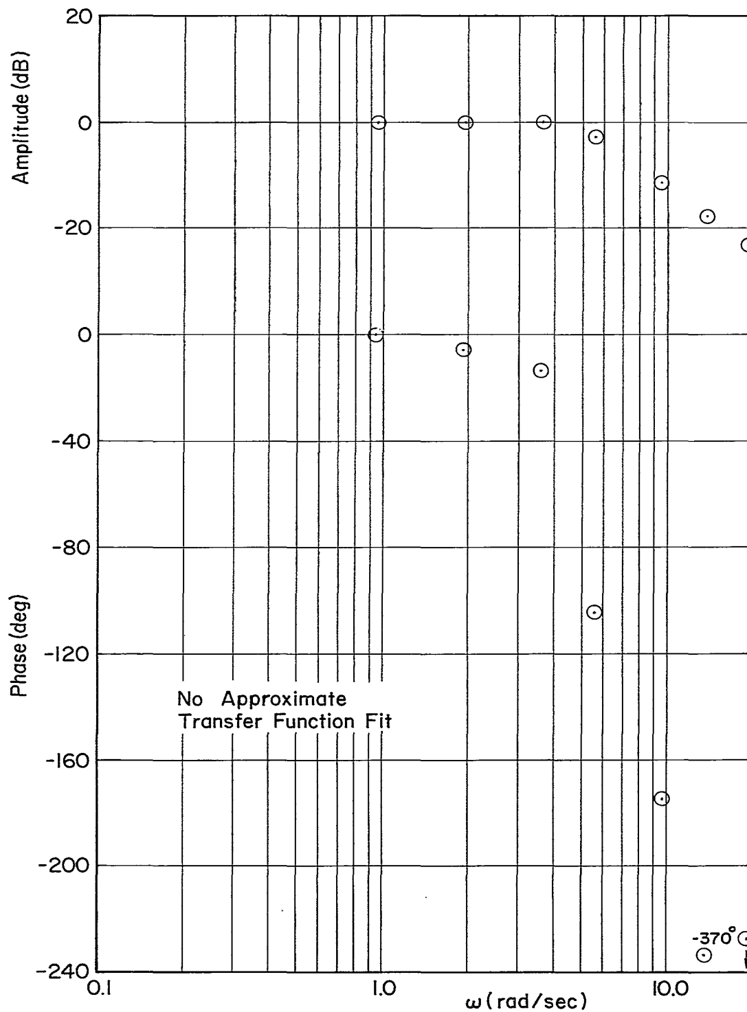
(a) Bank Angle Instrument Frequency Response
