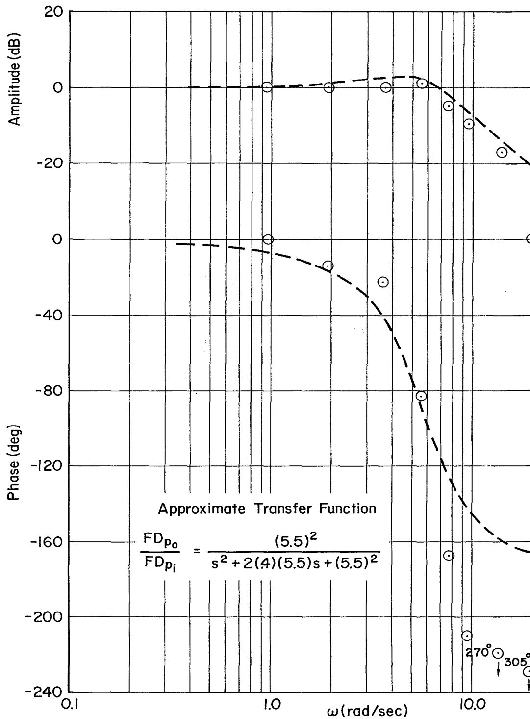
(c) Longitudinal Flight Director Instrument Frequency Response
