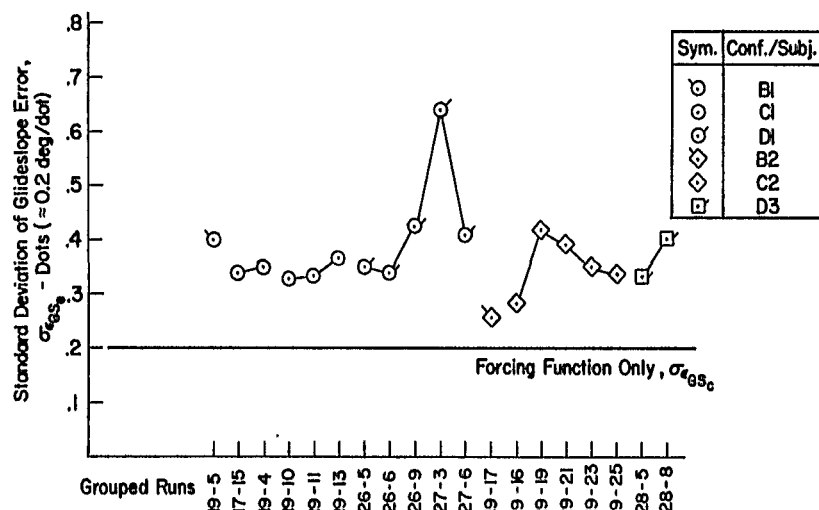
Figure 10. Glide Slope Performance with Manual ILS Configurations
