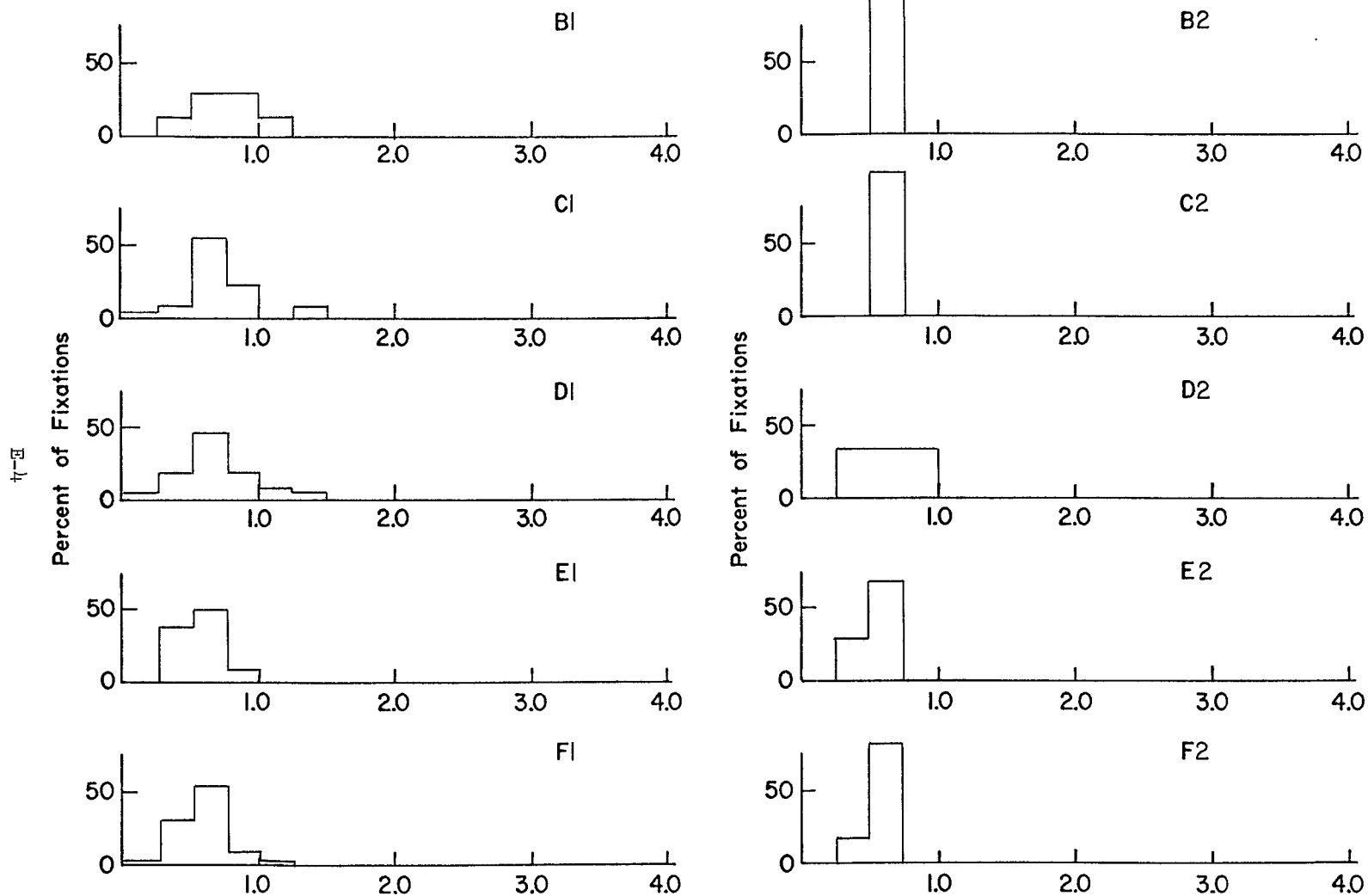
Figure E-1. Dwell Time Histograms for Instrument 1, IAS
