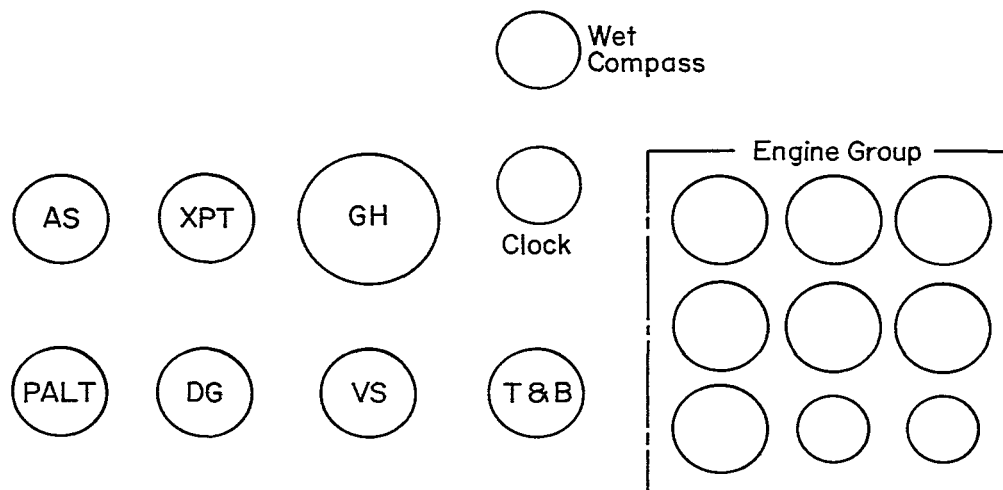
Figure 15. Experimental Instrument Arrangement Used by Fitts (Refs. 4 and 5)
