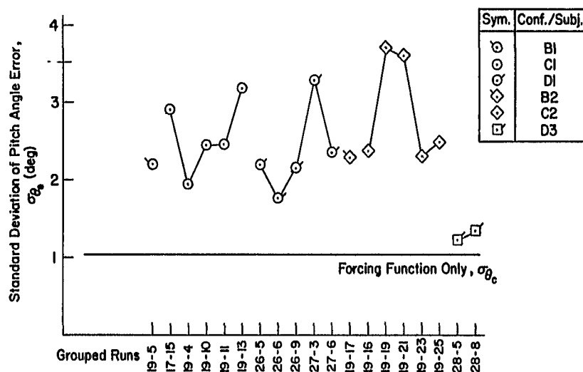
Figure 12. Pitch Attitude Performance with Manual ILS Configurations
