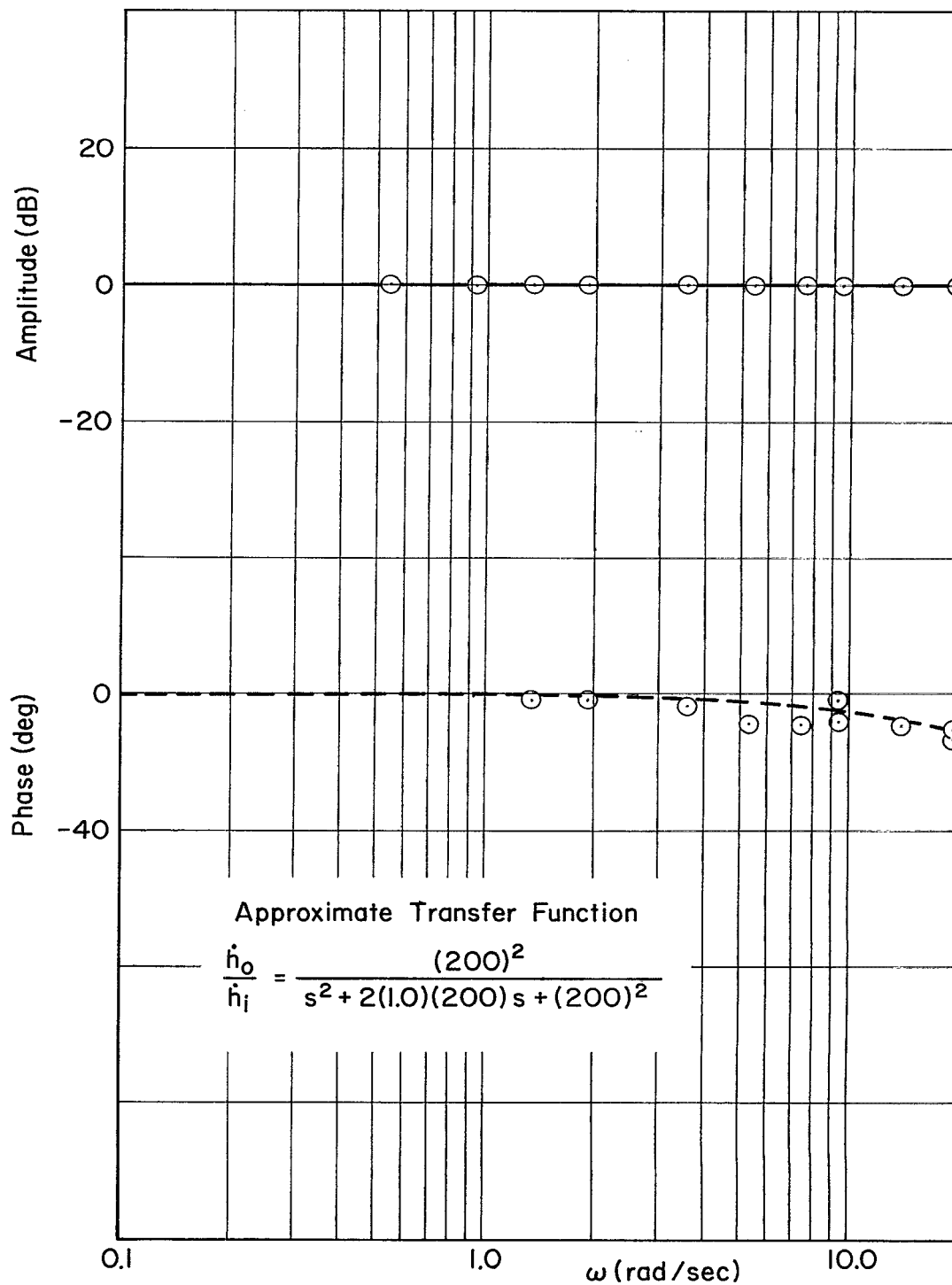
(a) Rate of Climb Instrument Frequency Response Figure B-9. Peripheral Longitudinal Instruments
