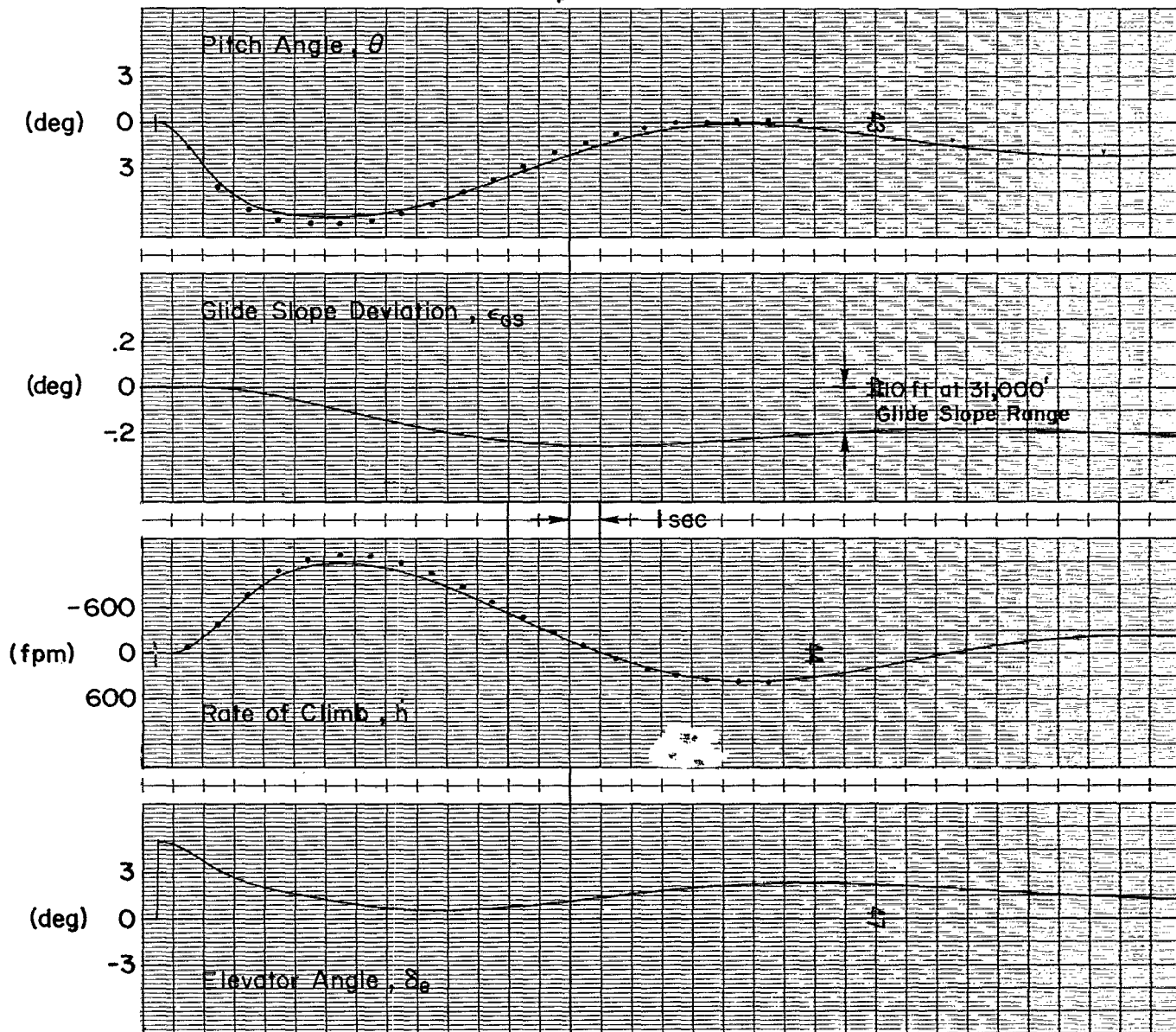
Figure B-4. Check of Closed-Loop Longitudinal Flight Director Response
