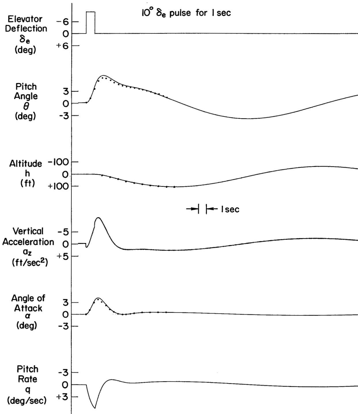
Figure B-1. Open-Loop Transient Response to 1 sec Elevator Pulse of 10^\circ
