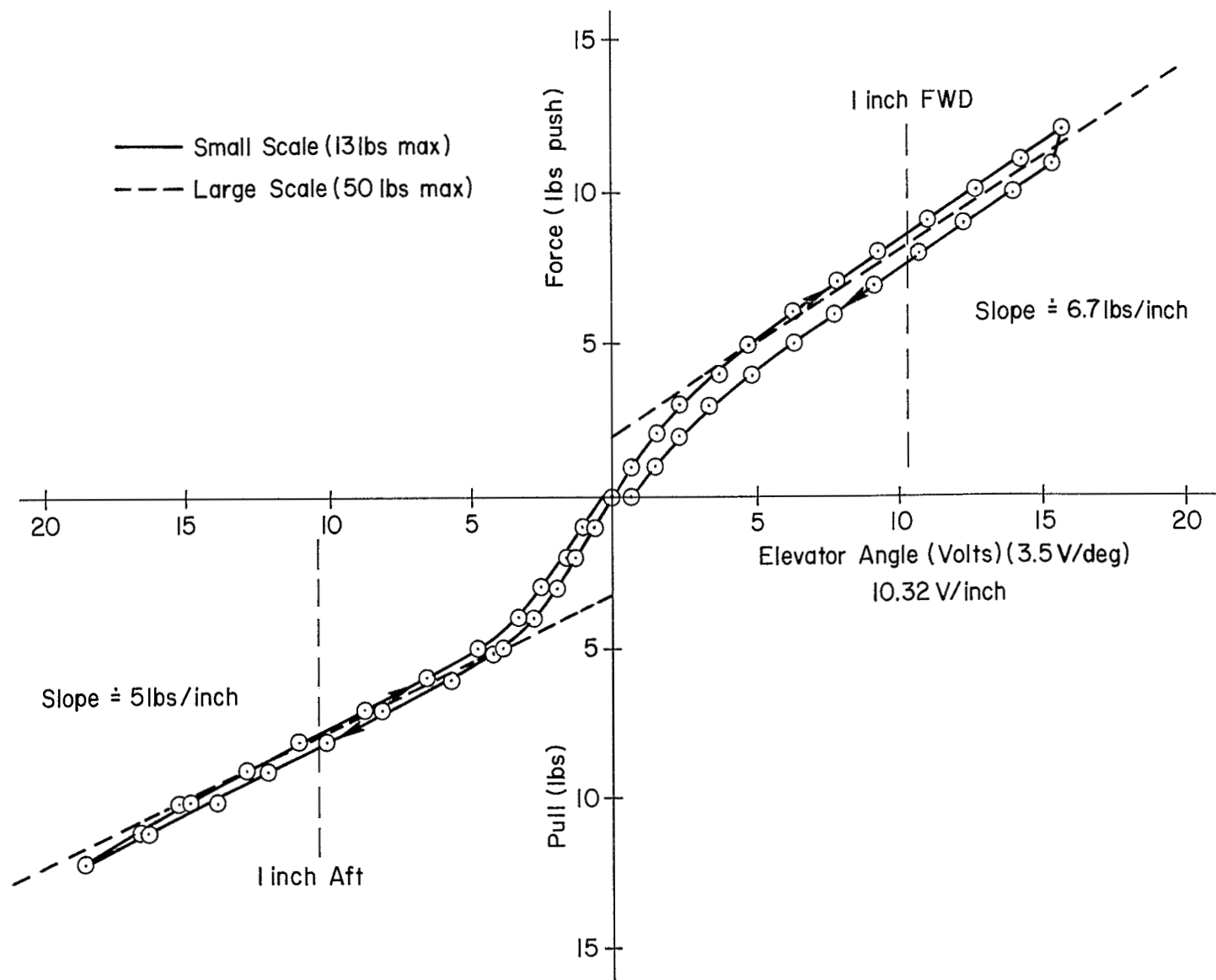
Figure B-10. Elevator Control Force Characteristics
