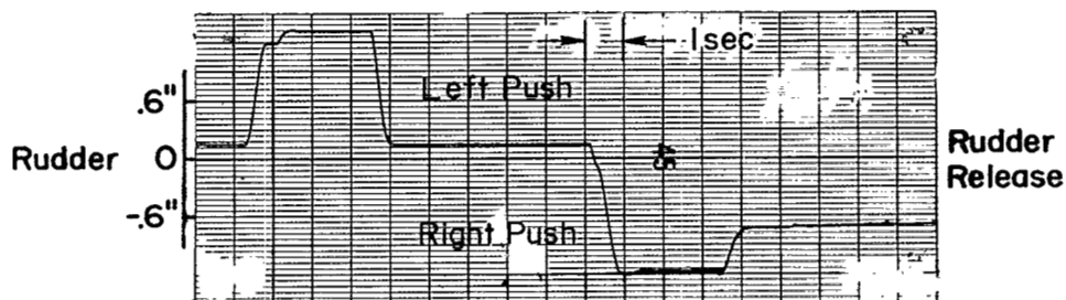
Figure B-12. Control Response from a Displacement Release
