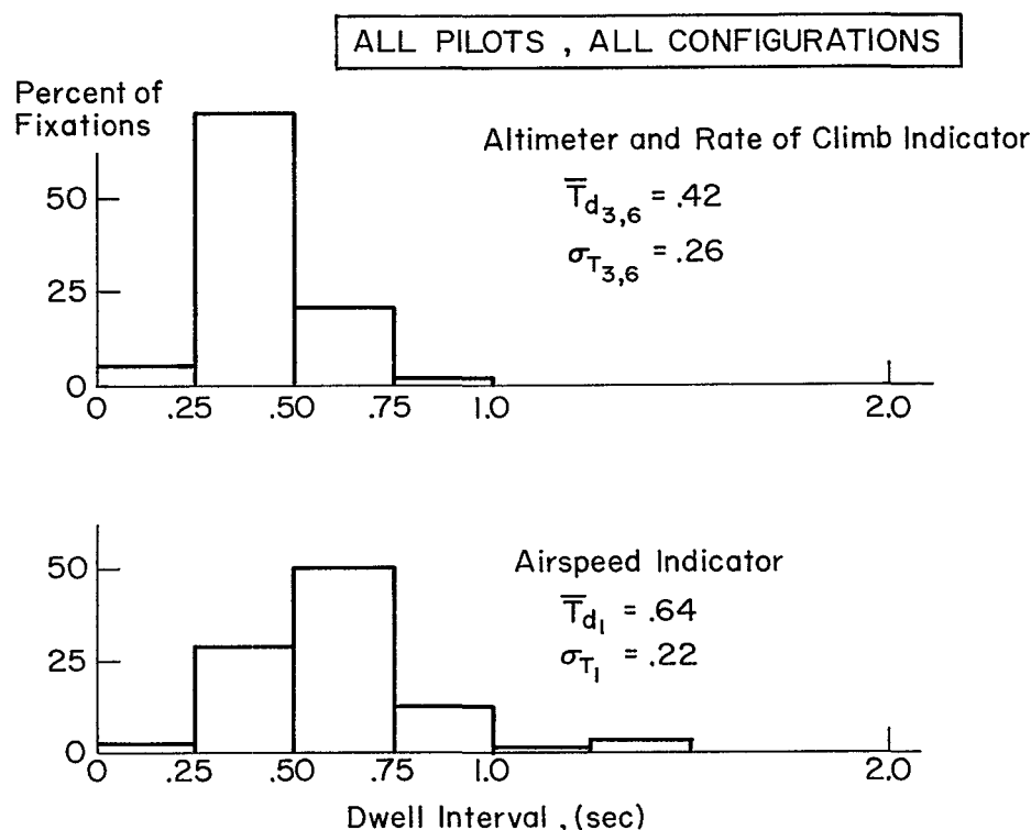
Figure 6. Peripheral Instrument Dwell Times
