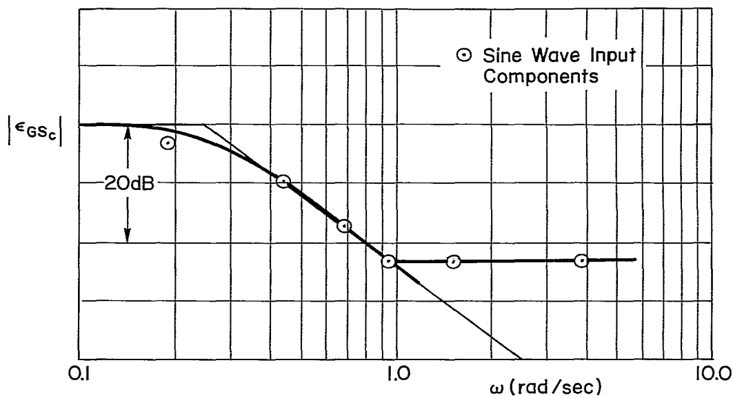
Figure C-4. Power Spectrum of Glide Slope Forcing Function
