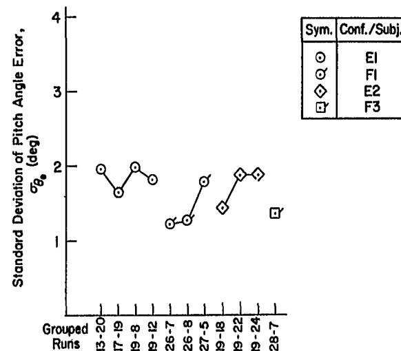
Figure 13. Pitch Attitude Performance with Flight Director Configurations
