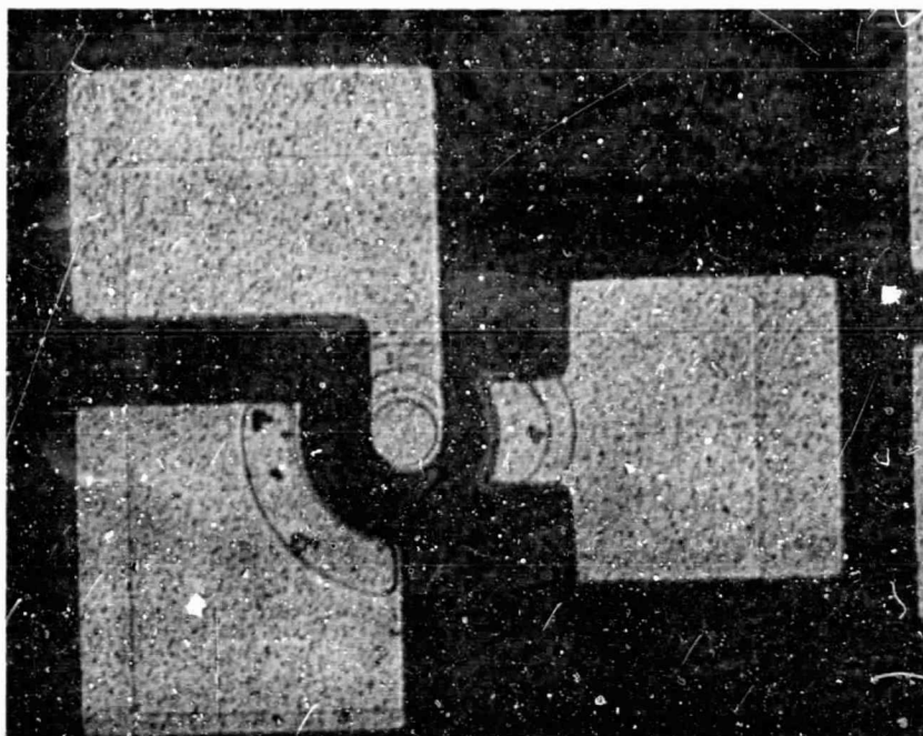
Figure 18. Micropower PNP
