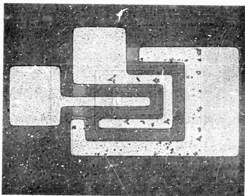
Figure 13. Lateral PNP Transistor - Single Emitter
