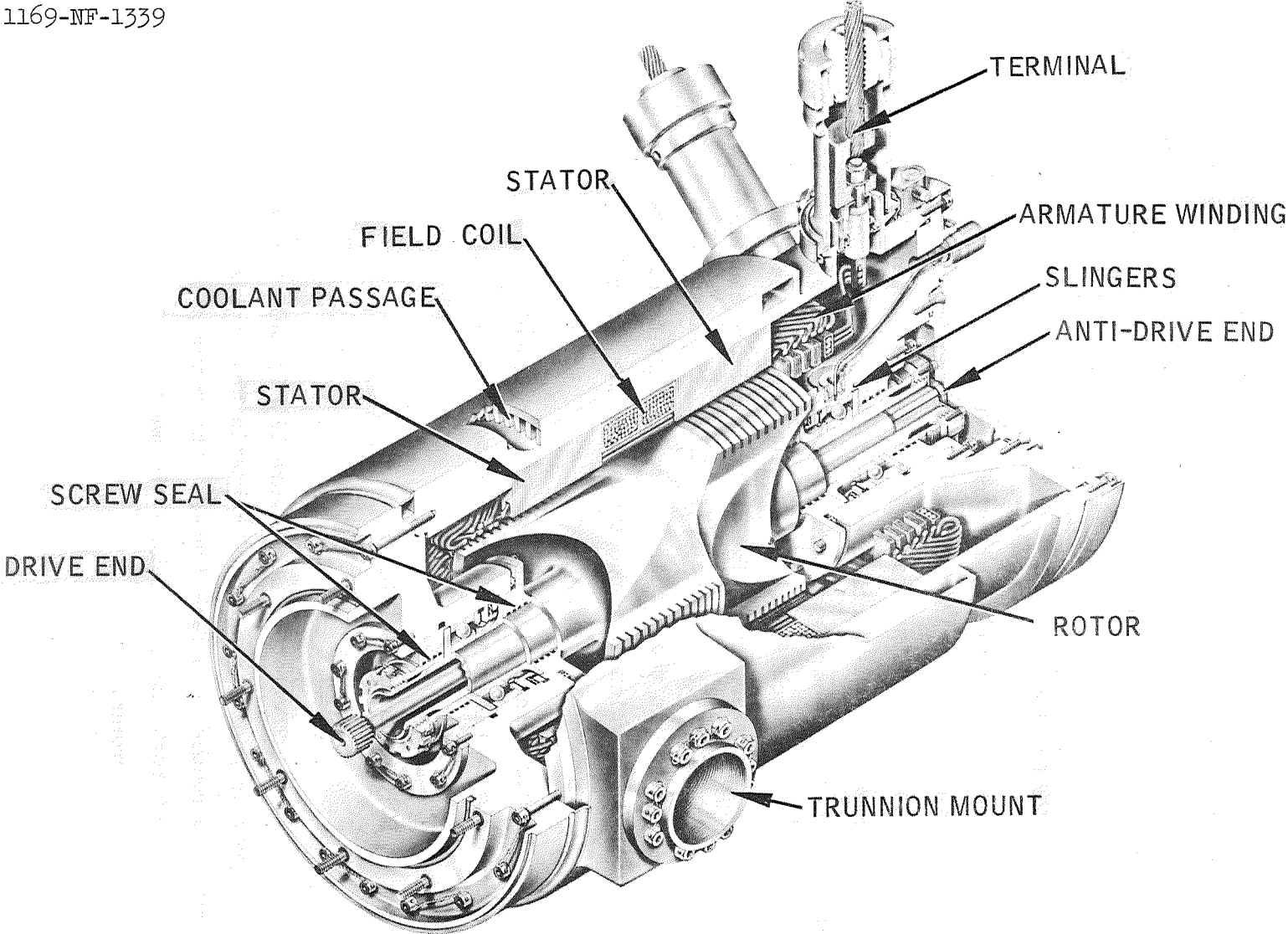
Figure 9. SNAP-8 Alternator
