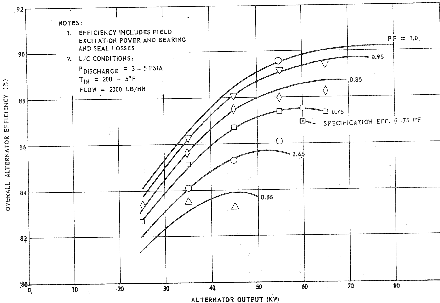
Figure 12 Alternator 181189 Efficiency Characteristics
