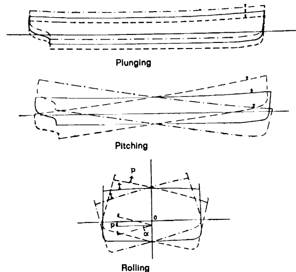
FIGURE 1.—Three types of oscillations of a ship's movements on rough seas.
