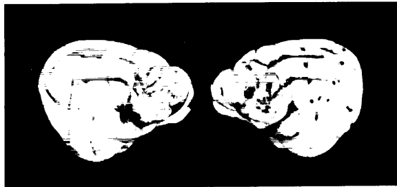
FIGURE 18.—Bilateral ablation of the gyrus ecto- and suprasylvius anterior. (From ref. 4.)
