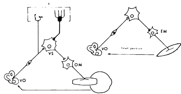
FIGURE 13.—Possible three-neuron arcs with (A) or without (B) cerebellar control. VS: Superior vestibular nucleus. EM: Extensor motoneuron. Explanation is in text.
