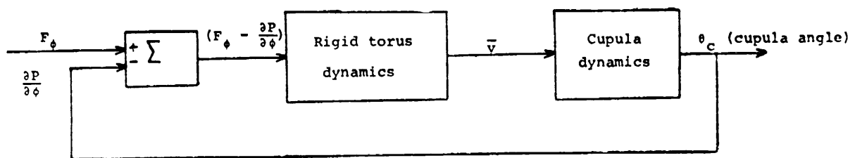
FIGURE 1.—Schematic diagram for dynamics of the semicircular canal.
