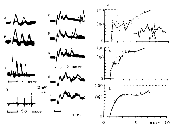
FIGURE 5.— Multiple discharges in vestibular nerve fibers which occurred in response to single vestibular nerve stimulation. A through D: Partial intracellular recording from three vestibular nerve fibers (A, B, C, D) within the nucleus of Deiters. E through I: Extracellular recording from the nucleus of Deiters. Double-shock stimuli, each being supramaximal for P-wave, were given to the vestibular nerve at various intervals. The test stimuli were switched off in about half of the trials at the moments indicated by dots. J: Relates the amplitudes of the test P-wave in the records partly illustrated in E through I (ordinate) to the shock intervals (abscissa). Inset diagram in J indicates how to measure the size of the P-wave, which is the sum of the respective peak amplitudes of the positive (p) and negative (n) phases of P-wave as measured from the potential curves following the conditioning stimuli alone (broken line). K, L: Similar to J, but taken immediately after (K), and about 2 hours after (L), destruction of the vestibular organ. (From ref. 18.)
