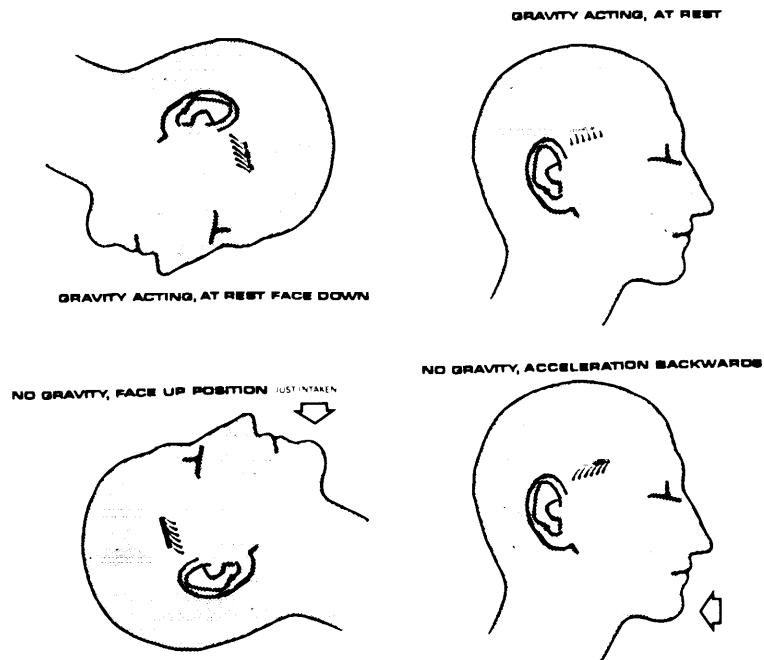
FIGURE 24.—Visualization of the macular spatial illusion.
