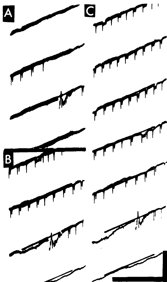
FIGURE 10.—A, B: Decerebrate cat with 13\text{-M}\Omega resistance microelectrodes (3 M KCl pipets) inserted into the tuber vermis. Single electrical stimuli were given. Records read from below upward. Calibration, 50 msec (horizontal) and 1 mV (vertical). C: Cat under Chloralose medication (70 mg/kg). Record reads from below upward. Single electrical shock introduced first a fast burst of activity, then an enduring inhibition. Calibration, 50 msec and 1 mV.
