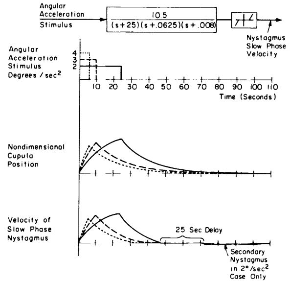
FIGURE 4.—Model response for Aschan and Bergstedt experiment (ref. 3).
