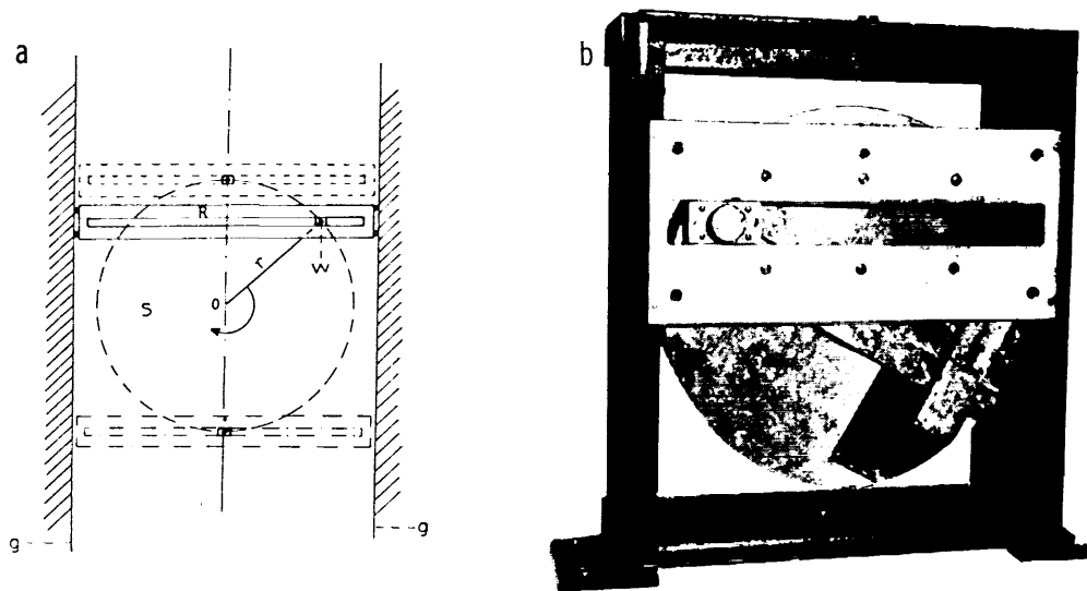
FIGURE 6.—Apparatus for producing vertical harmonic pendulous motion and inducing motion sickness experimentally. (a) Schematic of wheel shown in (b) that rotates at different constant rates and drives a frame up and down between two guide rails (b).
