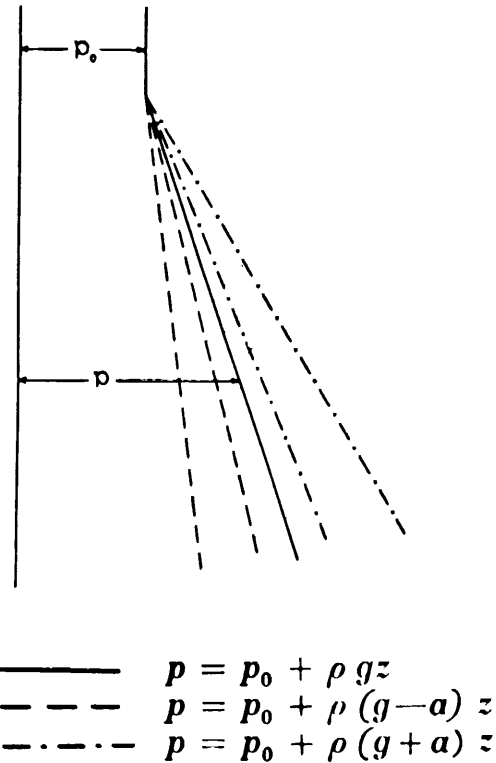
FIGURE 9.—Container in linear vertical motion with constant upward acceleration resulting in increased pressure.
