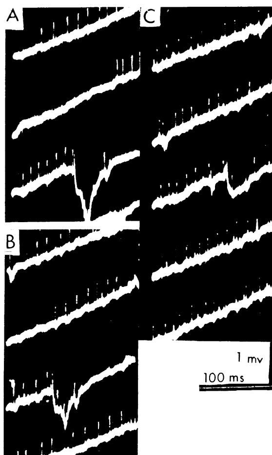
FIGURE 11.—A, B, C: Shows data collected when a 10\text{-m}\Omega , 3 M KCl-filled micropipet was inserted into the Purkinje-cell layer of the tuber vermis and used as a recording electrode. Single electrical shocks were given at 1\frac{1}{2} times threshold. Note prestimulatory and poststimulatory effects. Record reads from below upward. Same recording and stimulating sites for A, B, and C. Calibration, 100 msec (horizontal) and 1 mV (vertical). Two percent strychnine applied locally 2 minutes before B was taken and 5 minutes before C was taken.
