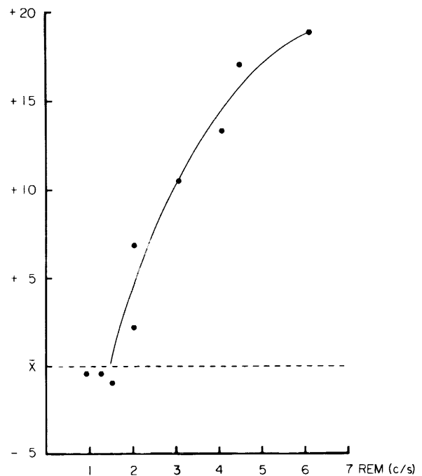
FIGURE 7.—Relationship between rate of ocular movements within bursts of REM and the enhancement of the antidromic group II cutaneous volley. Same animal and experiment as in figure 6. The dots represent the amplitudes of the antidromic group II cutaneous volley recorded from the left superficial radial nerve on single-shock stimulation of the ipsilateral cuneate nucleus during the REM periods of desynchronized sleep. The abscissa indicates the repetition rate (c/s) of ocular movements within the bursts of REM; the ordinate indicates the amplitude of the antidromic response during the trains of REM calculated as percentage of the mean control value \bar{X} obtained during the intervals between the REM. Each point represents the average value of measurements taken during 3 bursts of REM. The enhancement of the antidromic response is clearly related with the repetition rate of the ocular movements within the bursts of REM. (From ref. 31.)
