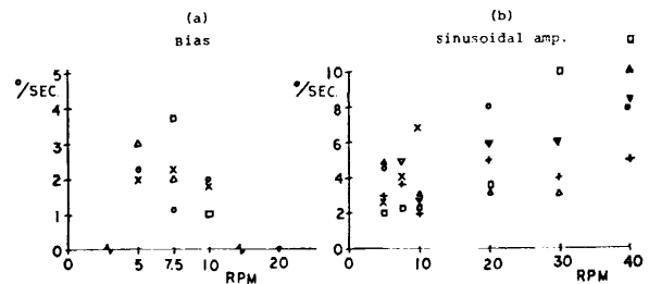
FIGURE 6.—Bias (a) and sinusoidal amplitude (b) of slow-phase nystagmus from rotation in 0.3-g field.
