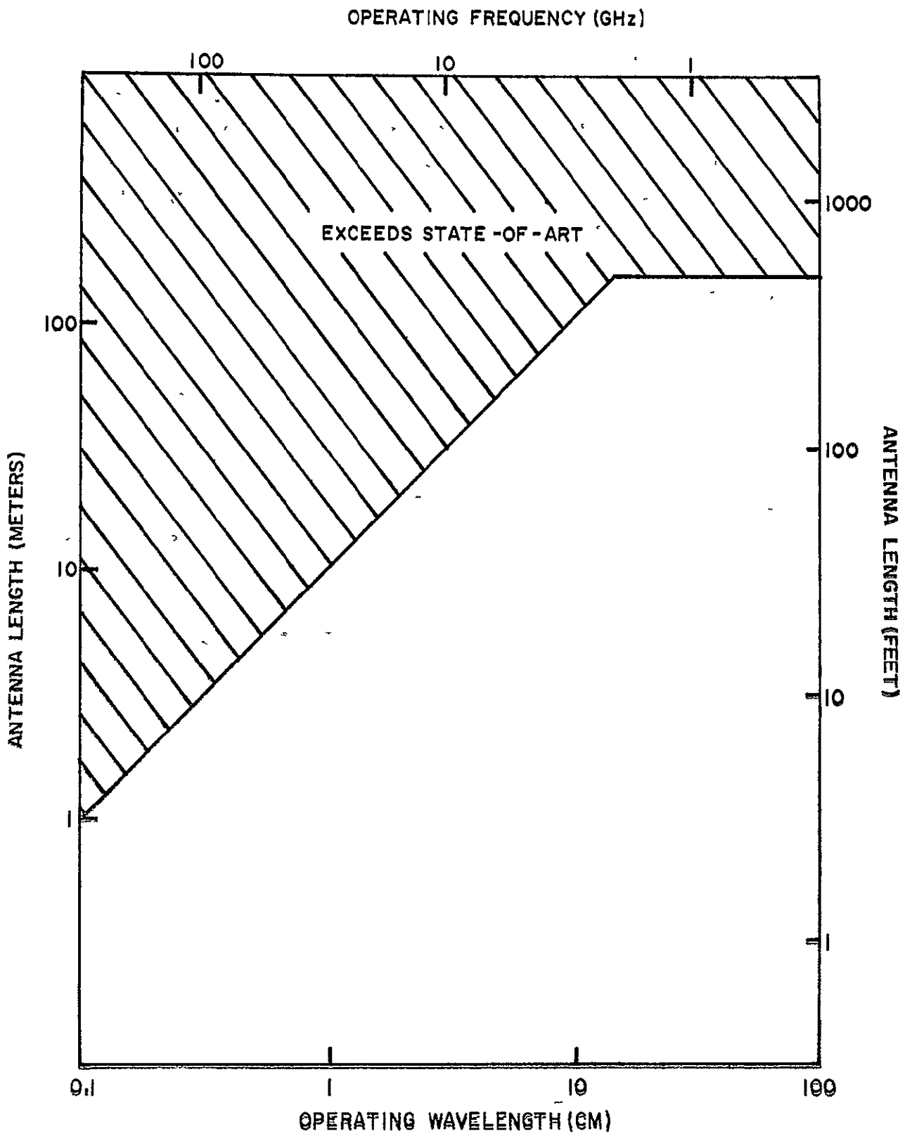
FIGURE 8-2. MAXIMUM ANTENNA LENGTHS
