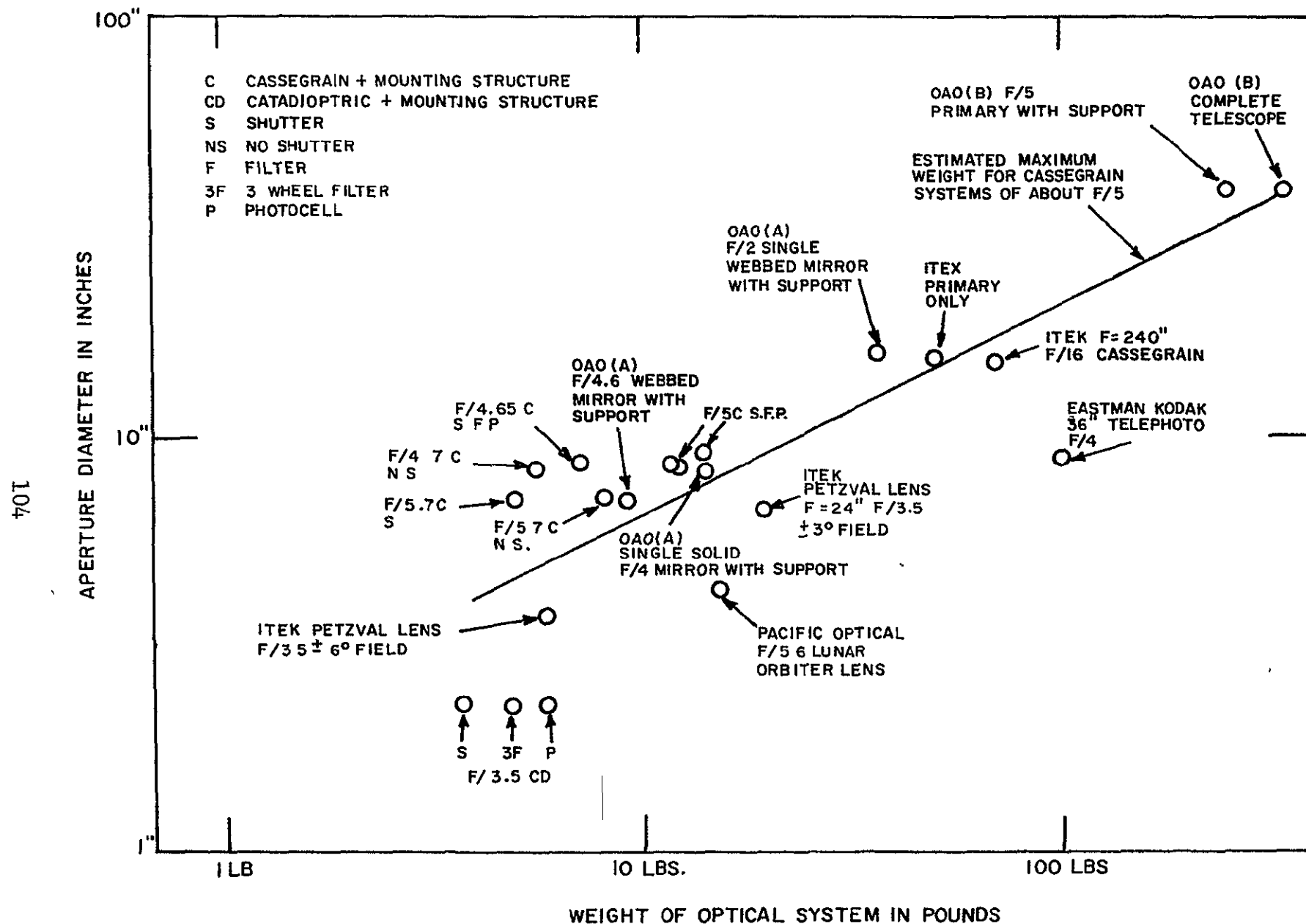
FIGURE 4-11 APERTURE DIAMETER VERSUS WEIGHT FOR A VARIETY OF SPACE OPTICAL SYSTEMS
