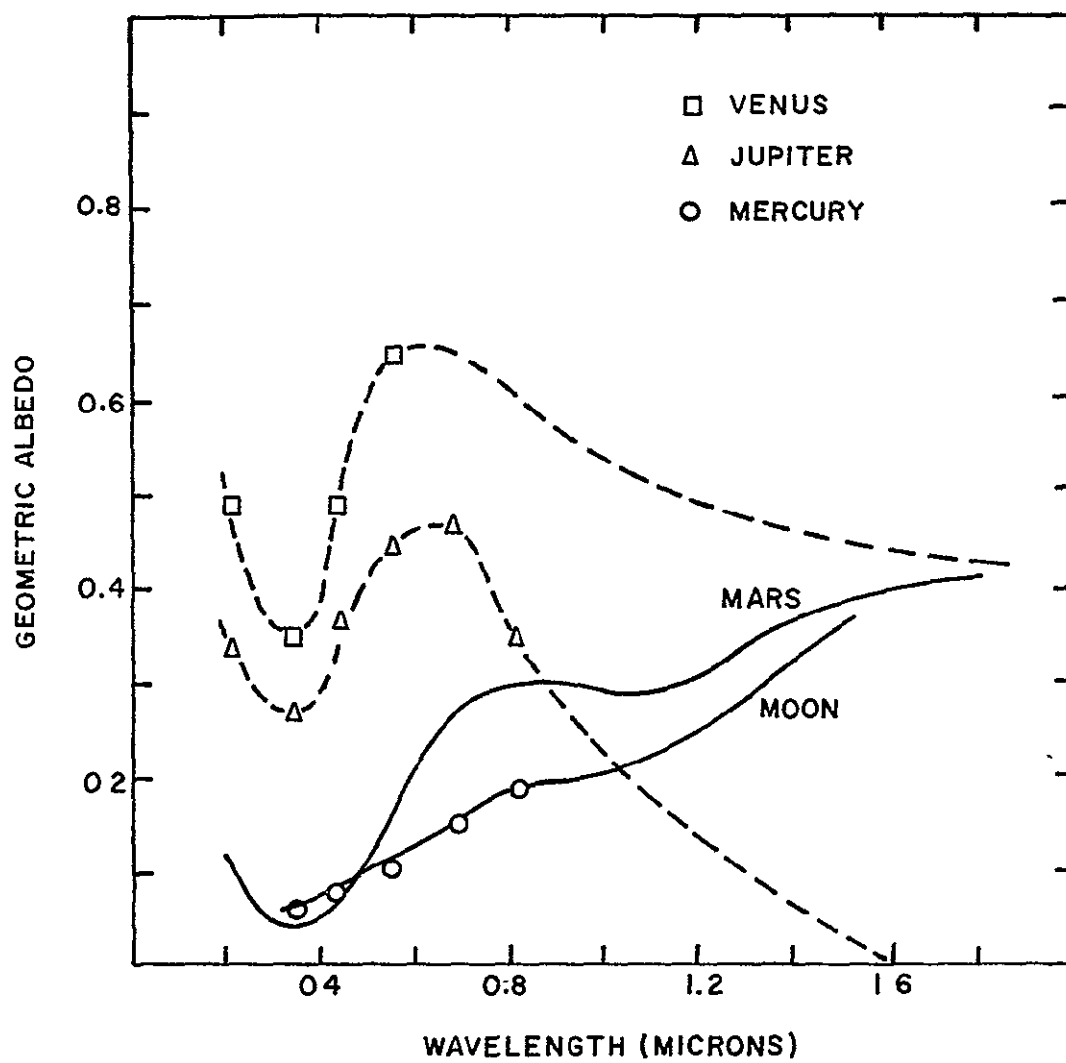
FIGURE 2-5. PLANETARY ALBEDOES
