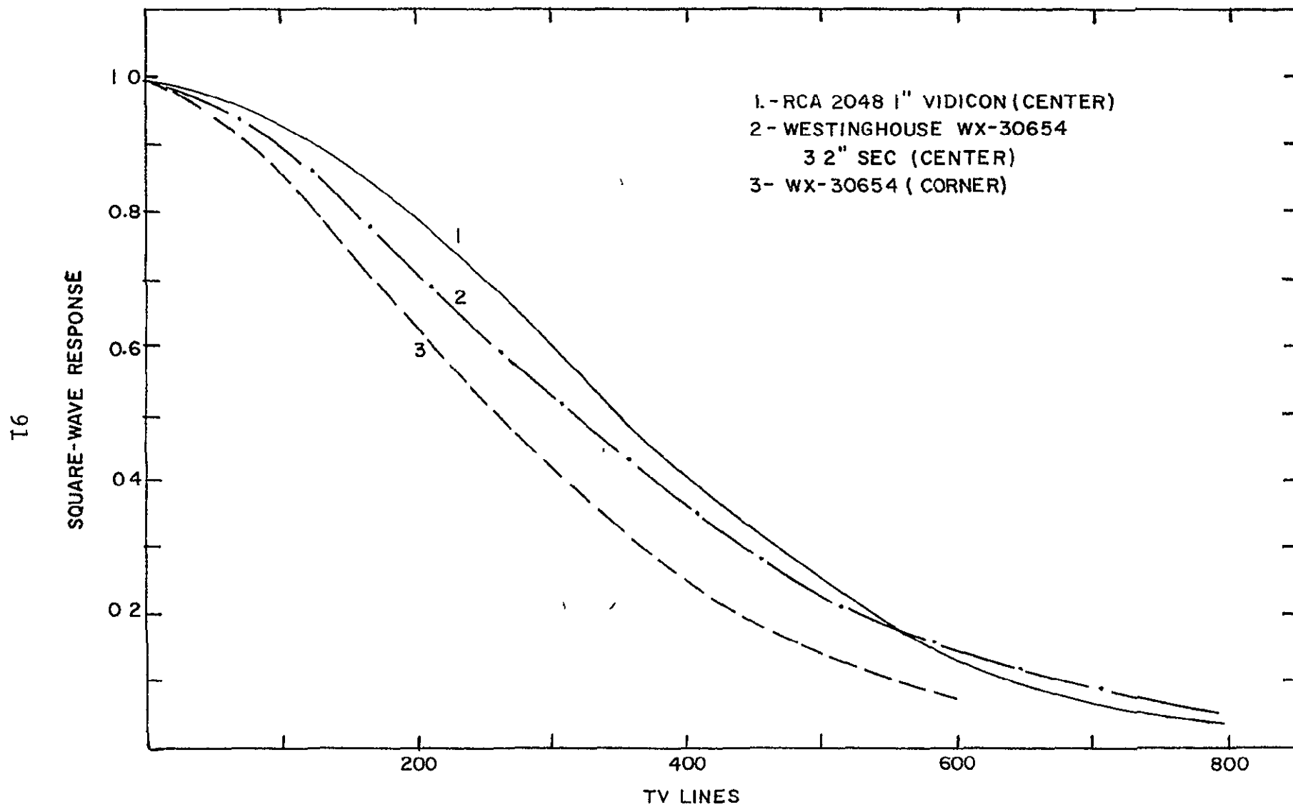
FIGURE 4-6 TV TUBE SQUARE-WAVE RESPONSE
