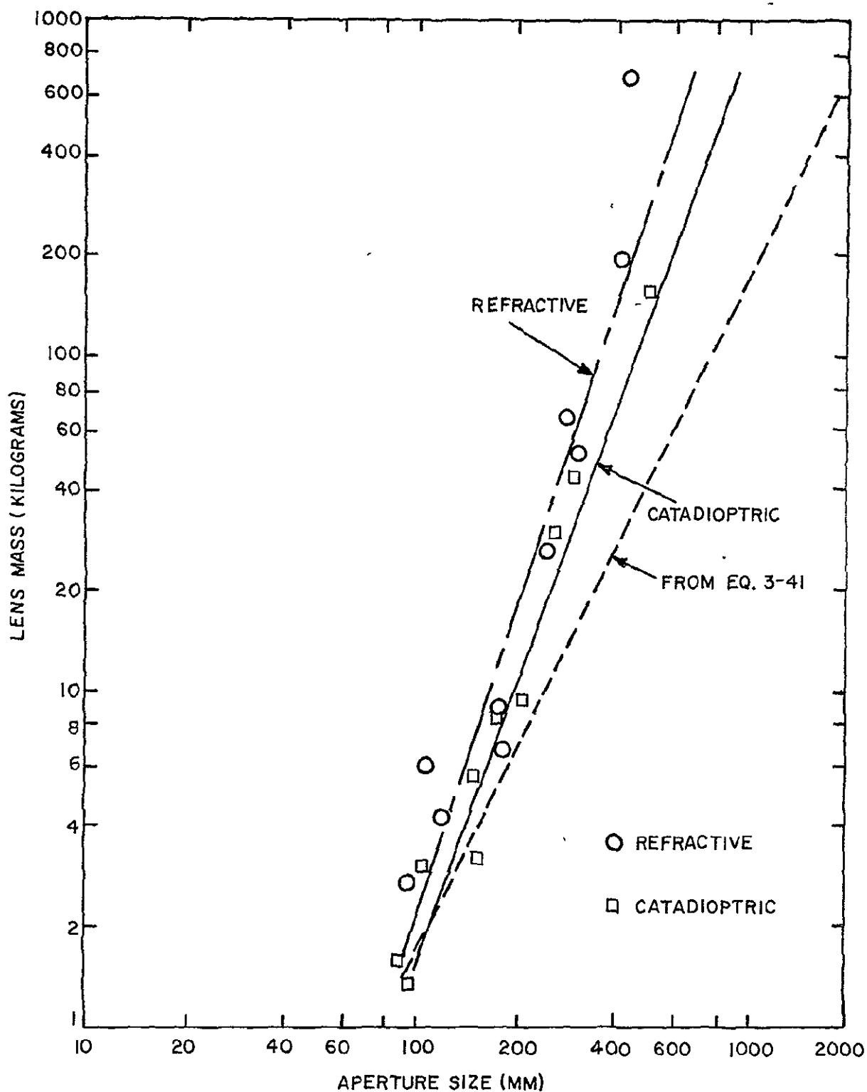
FIGURE 3-4. APERTURE SIZE VS. MASS FOR REFRACTIVE AND CATADIOPTIC OPTICAL SYSTEMS.
