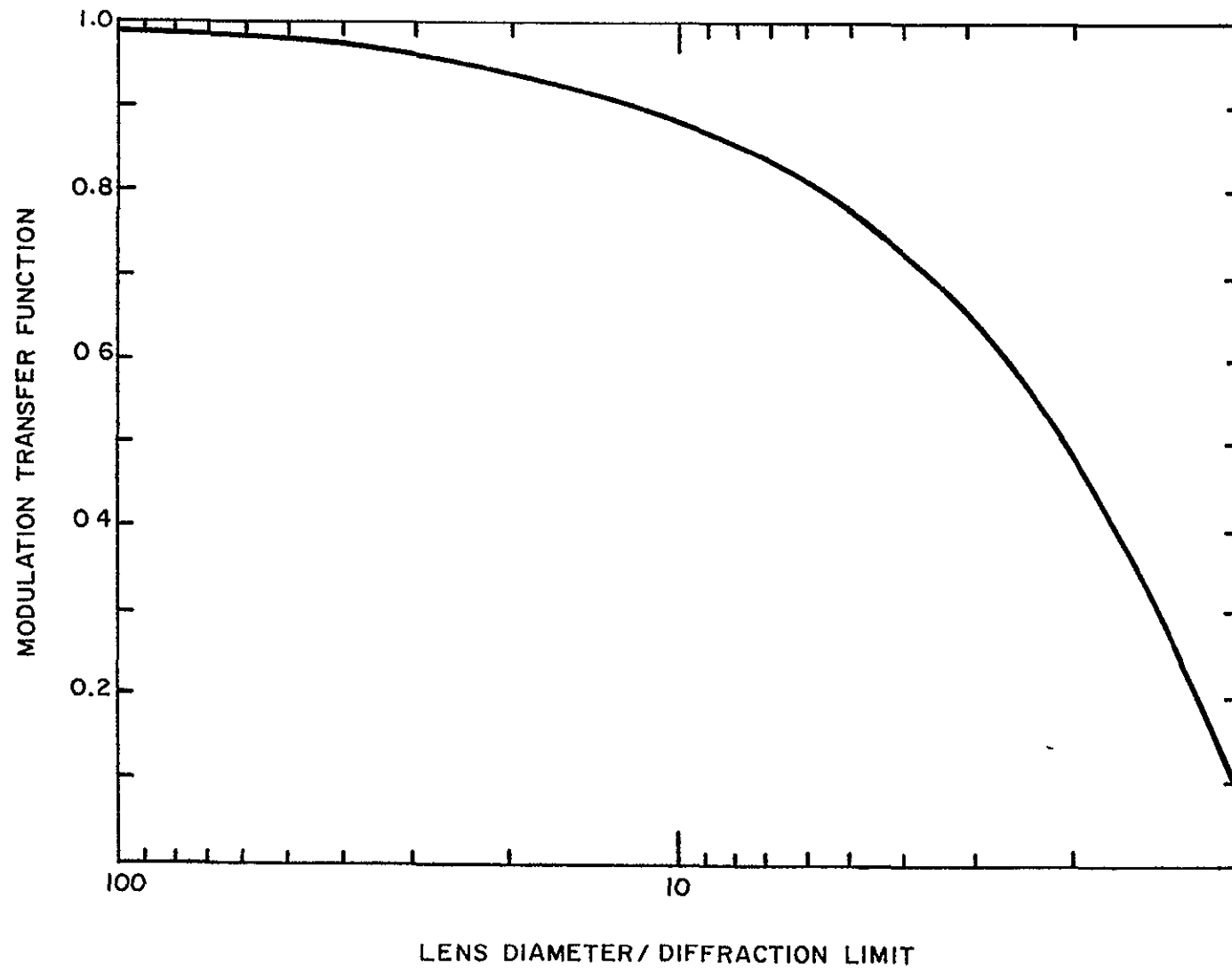
FIGURE 4-4 LENS TRANSFER FUNCTION
