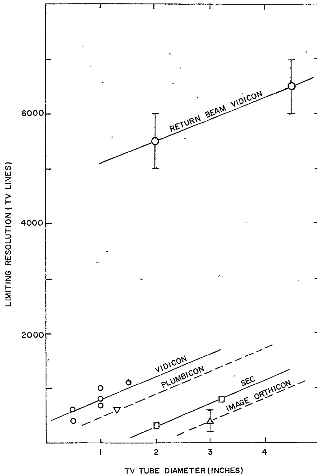
FIGURE 4-7 TV LIMITING RESOLUTION
