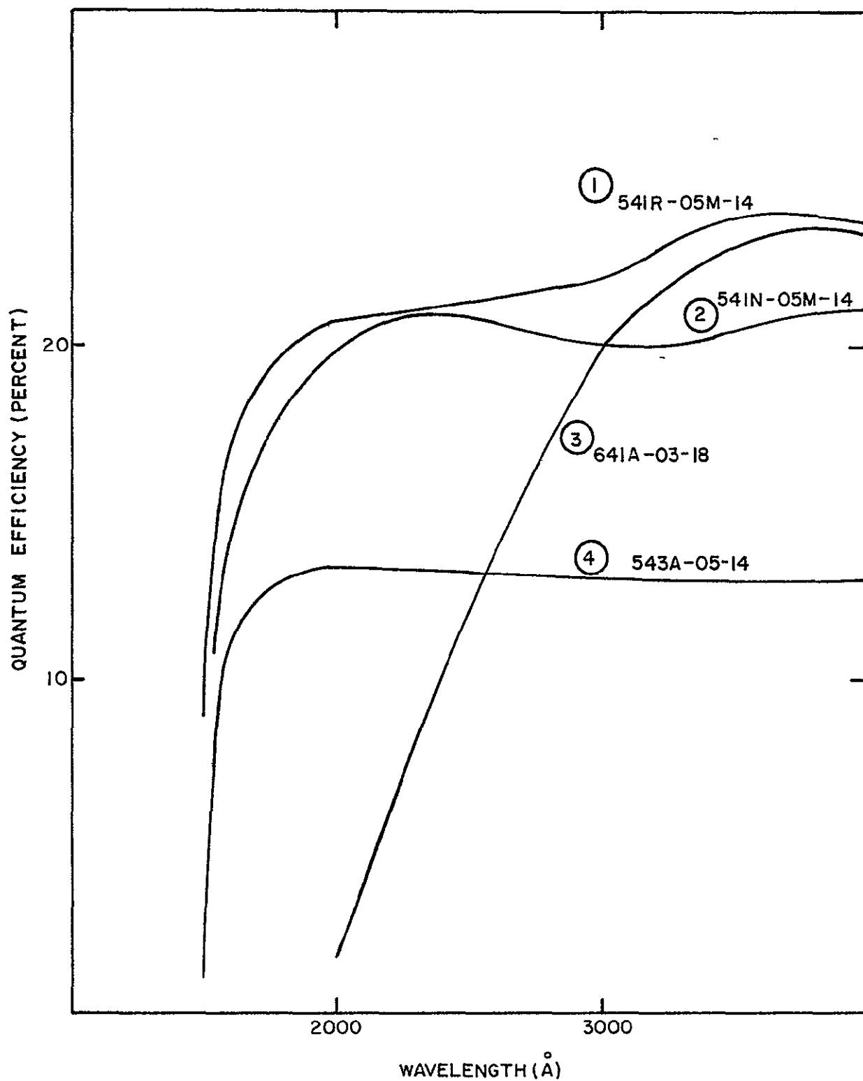
FIGURE 3-2. TYPICAL QUANTUM EFFICIENCIES
