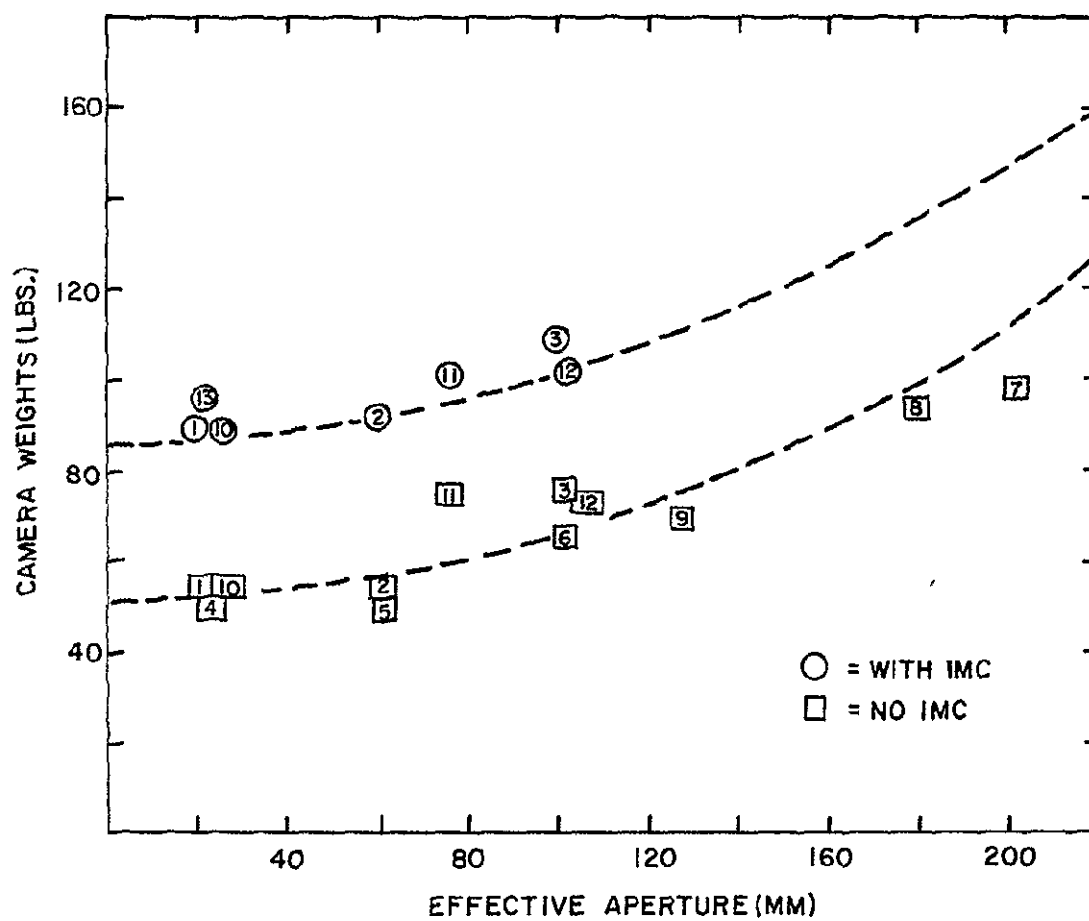
FIGURE 5-6. 9 \frac{1}{2} INCH FILM CAMERA WEIGHTS (W/ MAGAZINE)
