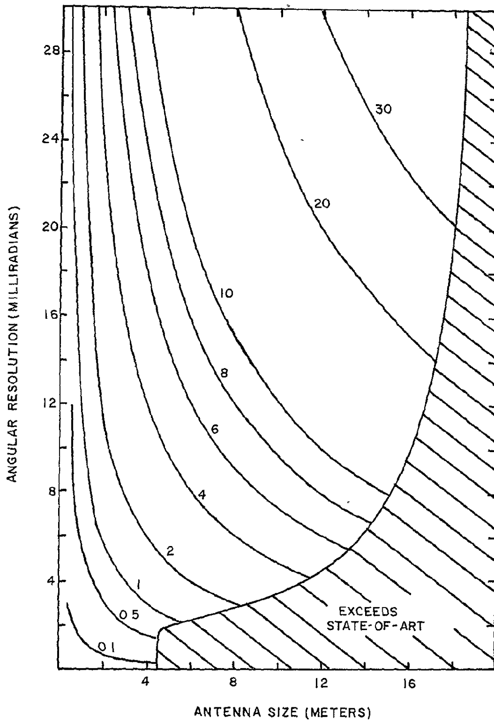
FIGURE 7-2 ATTAINABLE ANGULAR RESOLUTION (PARAMETRIC VALUES GIVE WAVELENGTH IN CM)
