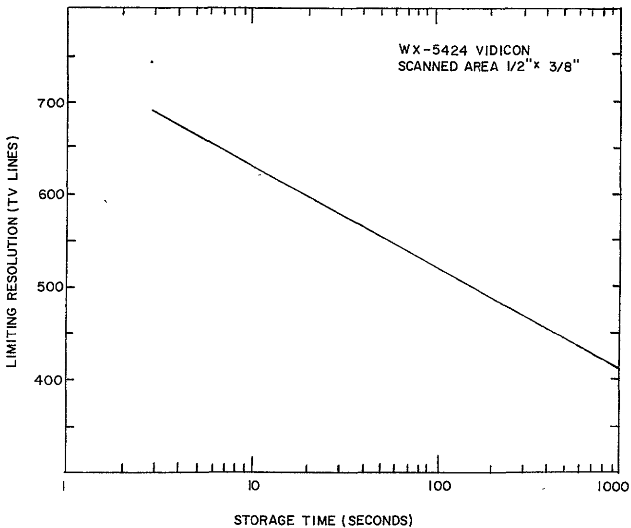
FIGURE 4-17. LOSS OF RESOLUTION WITH STORAGE TIME
