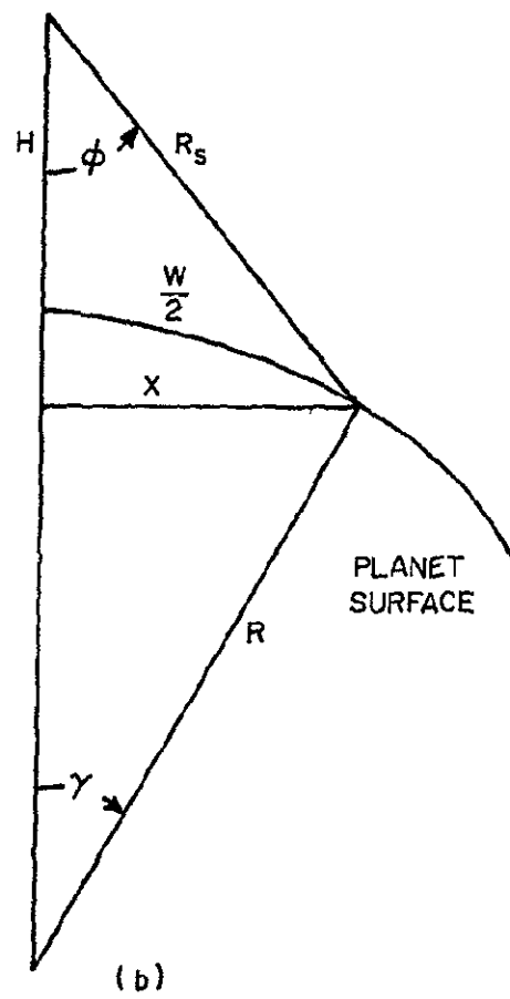
FIGURE 1-4. SCANNING SYSTEM GEOMETRY
