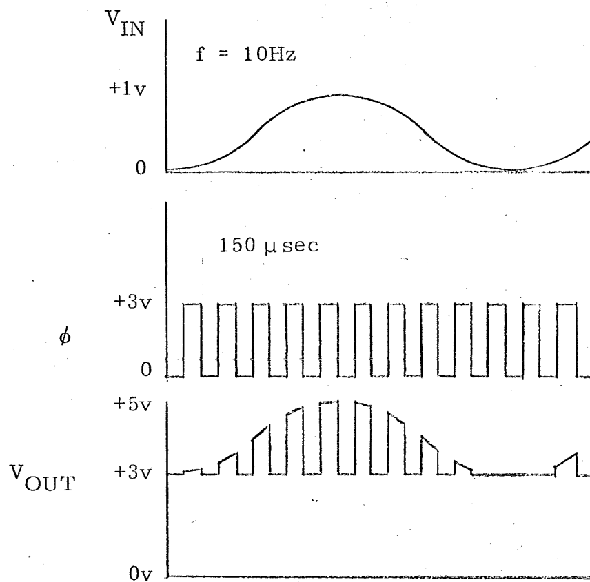
Figure 8. Analog delay with gain
