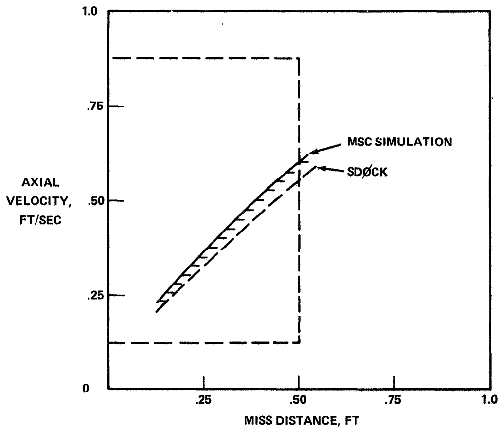
FIGURE 3—TYPICAL CAPTURE BOUNDARY
