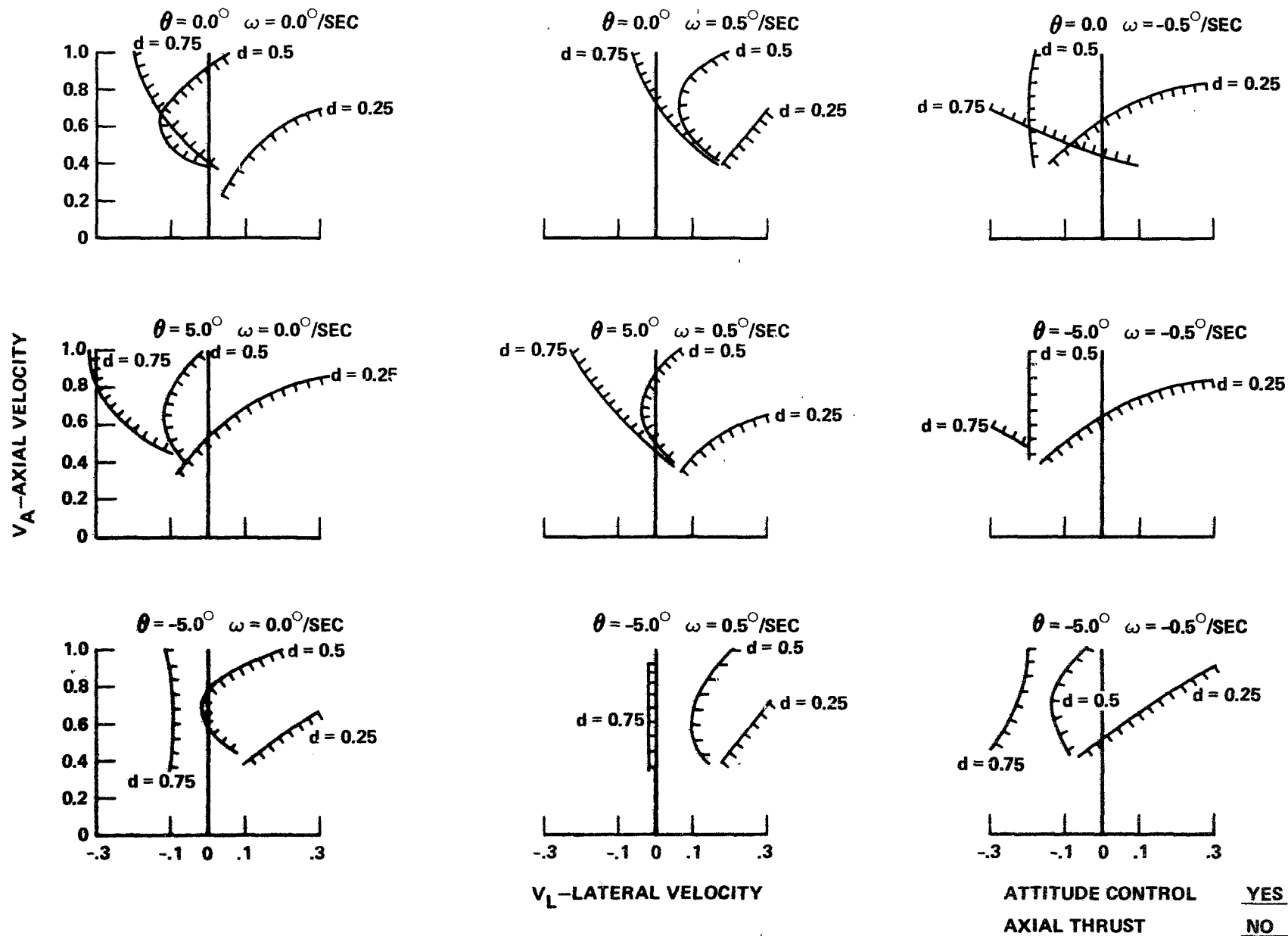
FIGURE 4 - CAPTURE BOUNDARIES
