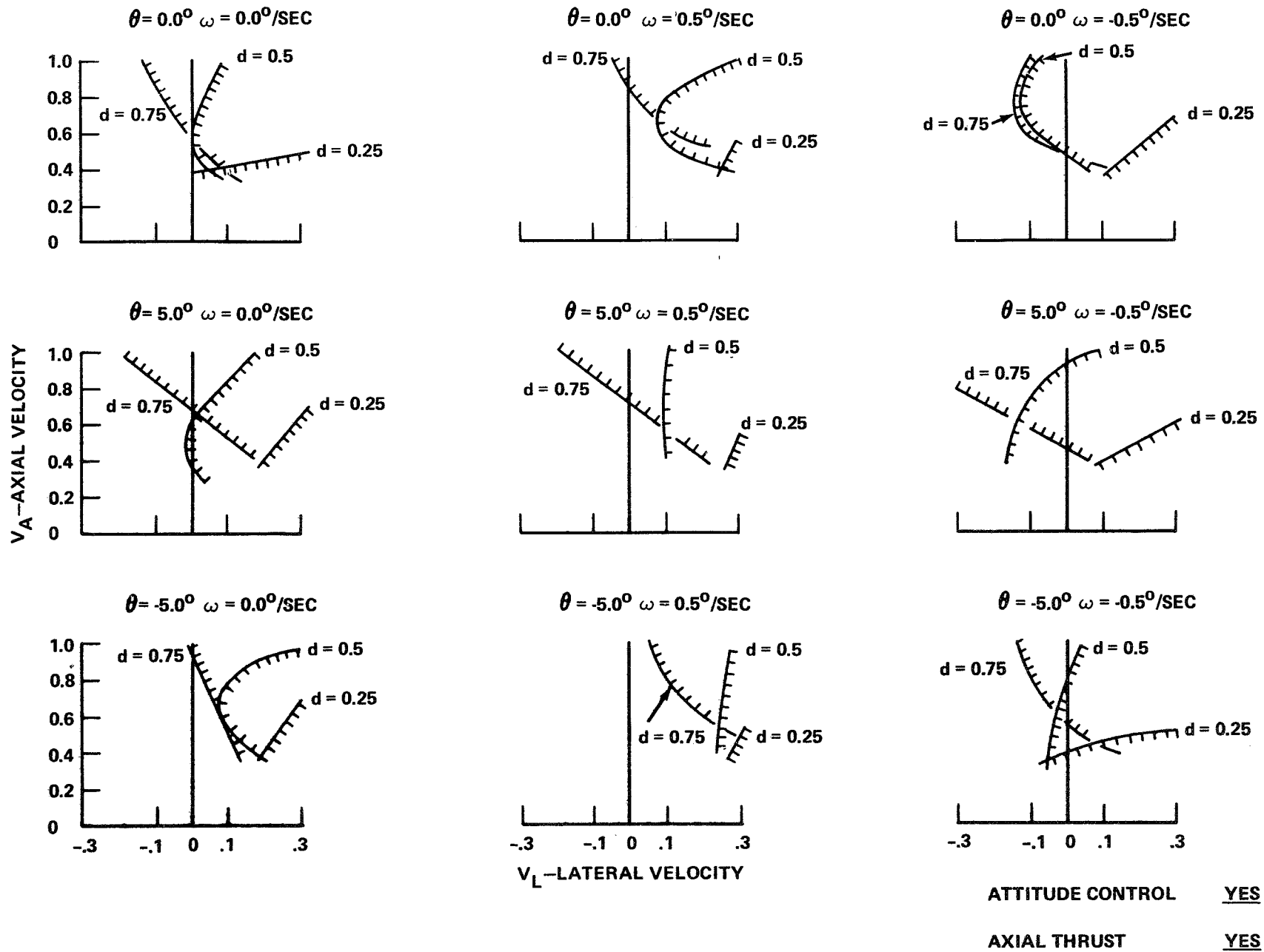
FIGURE 5 - CAPTURE BOUNDARIES
