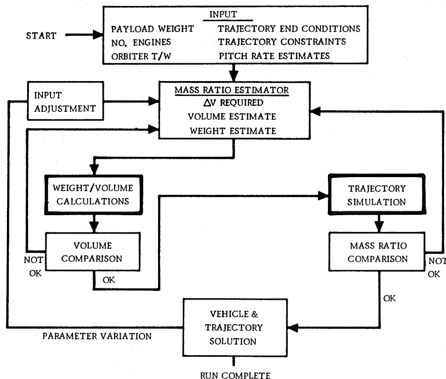
Figure 3-2. TSP Organization
