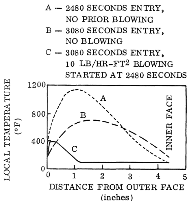
Figure 4-29. Gas Injection Through Insulation
