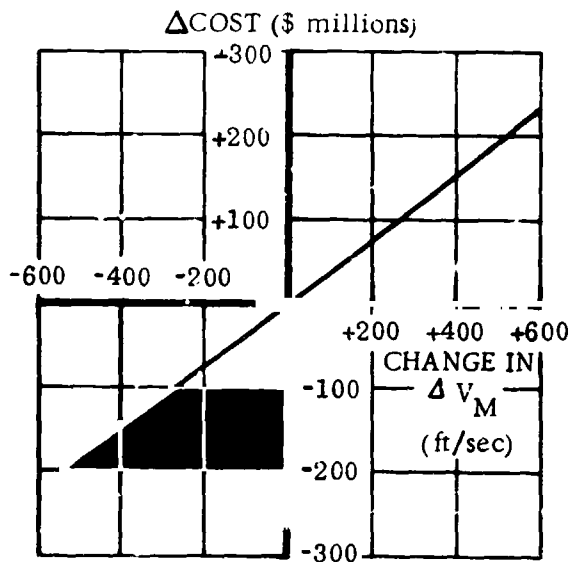
Figure 3-8. FR-3 Program Cost Sensitivity to Maneuver \Delta Velocity Requirements
