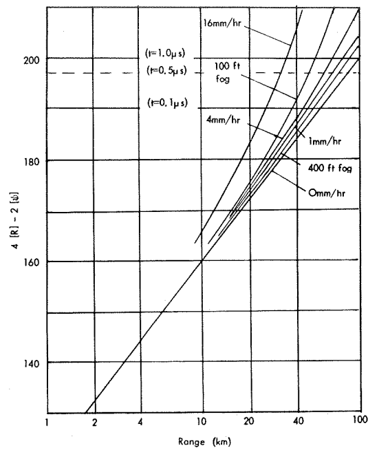
Figure III-34. 4[R] - 2[\psi] for X band.
