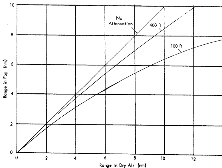
Figure III-15. Reduction in Range for Fog (Ku-Band at 18°C)
