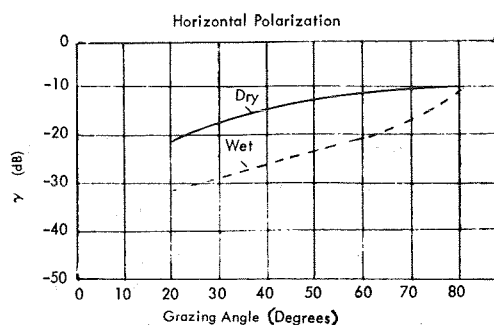
Figure III-9. Effects of Rain on an Asphalt Road at Ka band.
