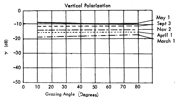
Figure III-11. Seasonal Changes of Grass at Ka band.
