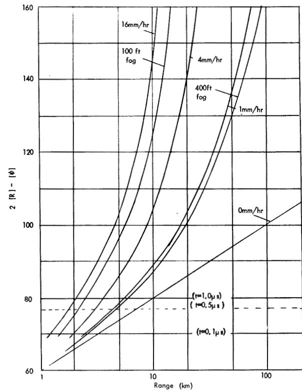
Figure III-41. Values of 2[R] - [\psi] for V band.
