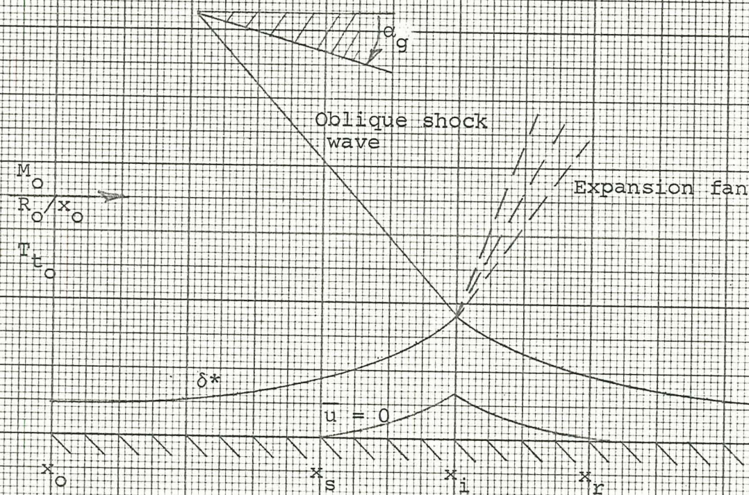
Figure 2.- Separated laminar flow on a flat plate as a result of shock wave-boundary-layer interaction.
