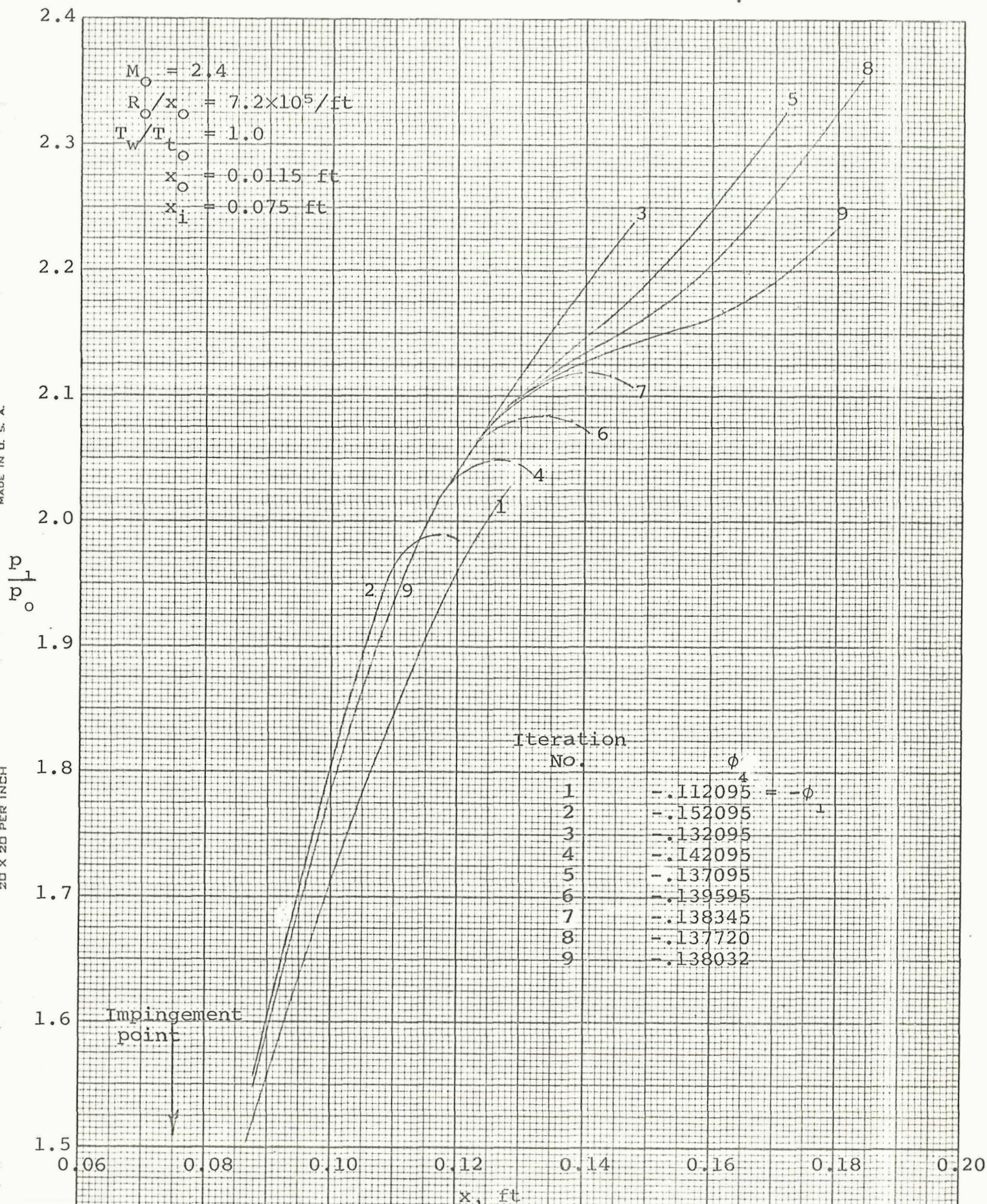
Figure 3.- Typical results of iteration for value of \phi_4 which satisfies downstream pressure boundary condition.
