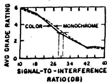
*Fig. 6 SNR requirement
