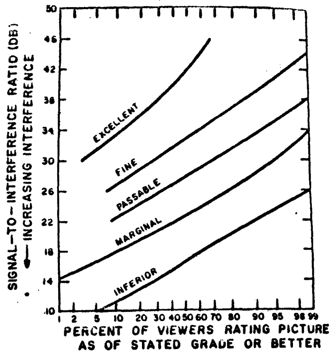
*Fig. 5 Subjective test of television system
