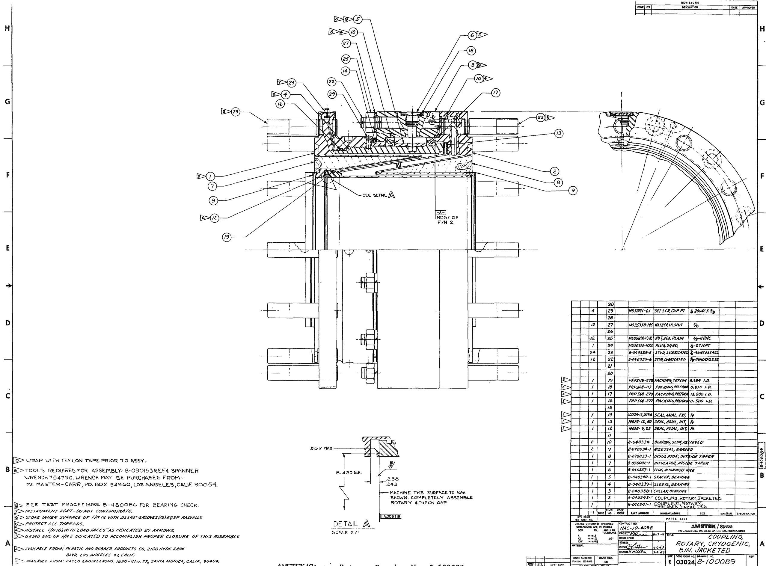
AMETEK/Straza Rotary, Drawing No. 8-100089
