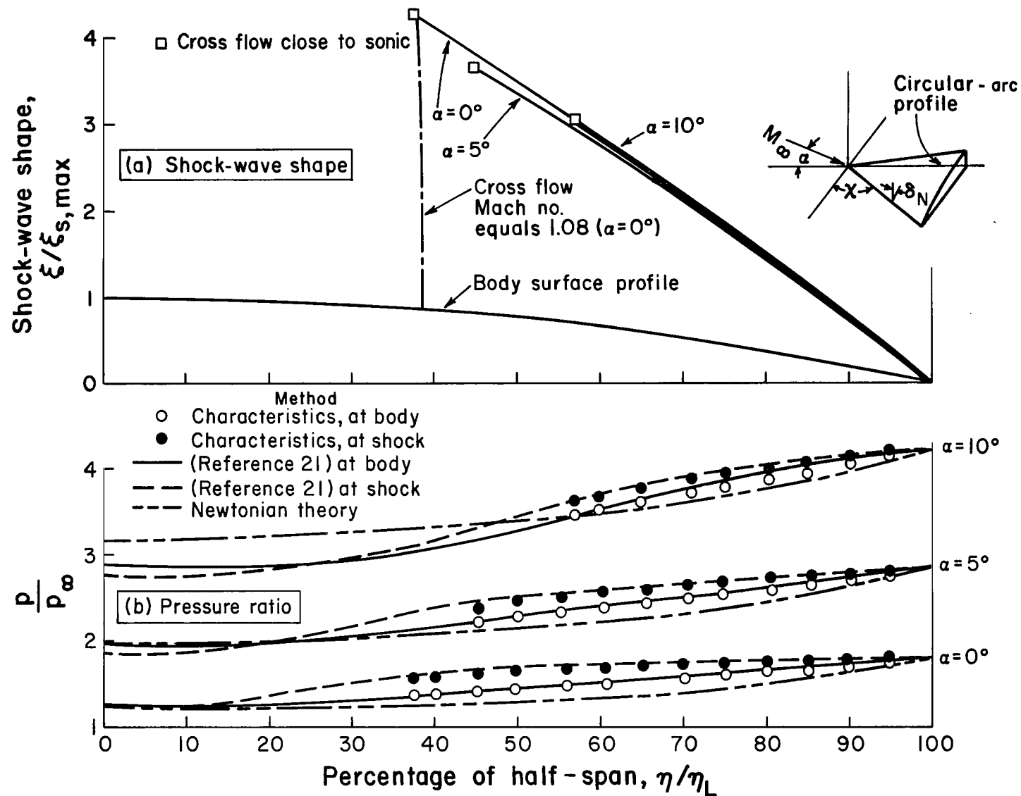
Figure 7.- Shock-wave shape and pressure ratio as a function of percentage of half-span for a circular-arc wing. \gamma = 1.40 ; M_\infty = 4.0 ; \delta_N = 90.18^\circ ; \chi = 50^\circ .
