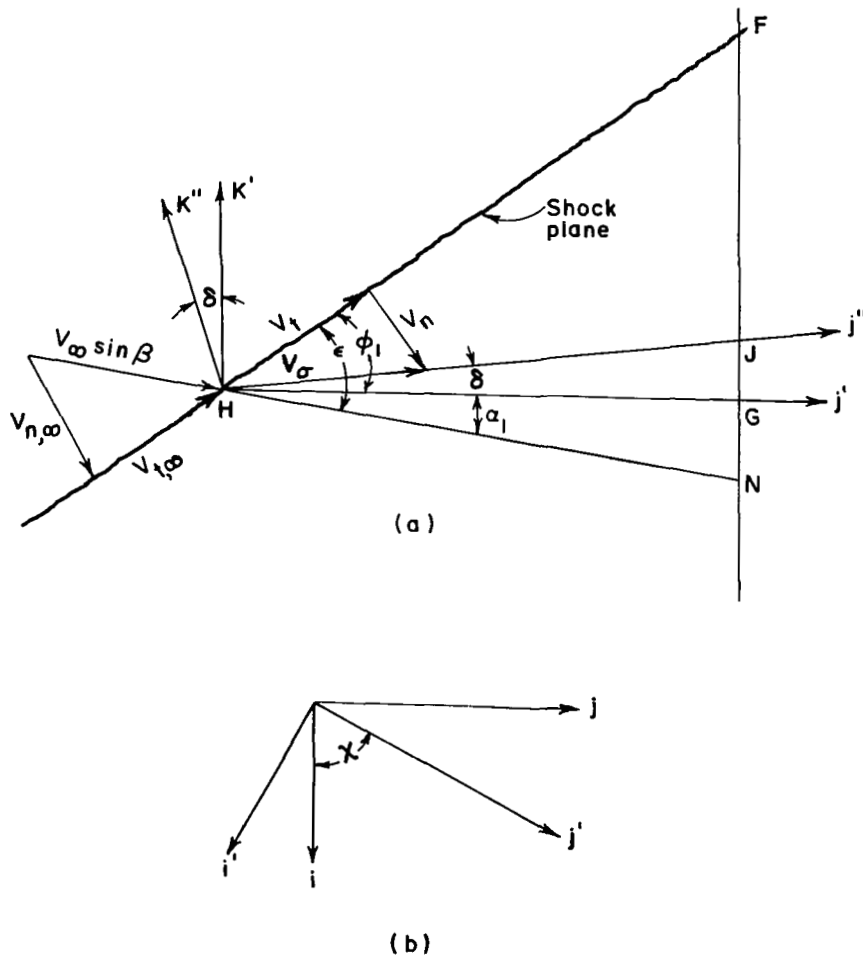
Figure B2.- Velocity components with rotating axes.
