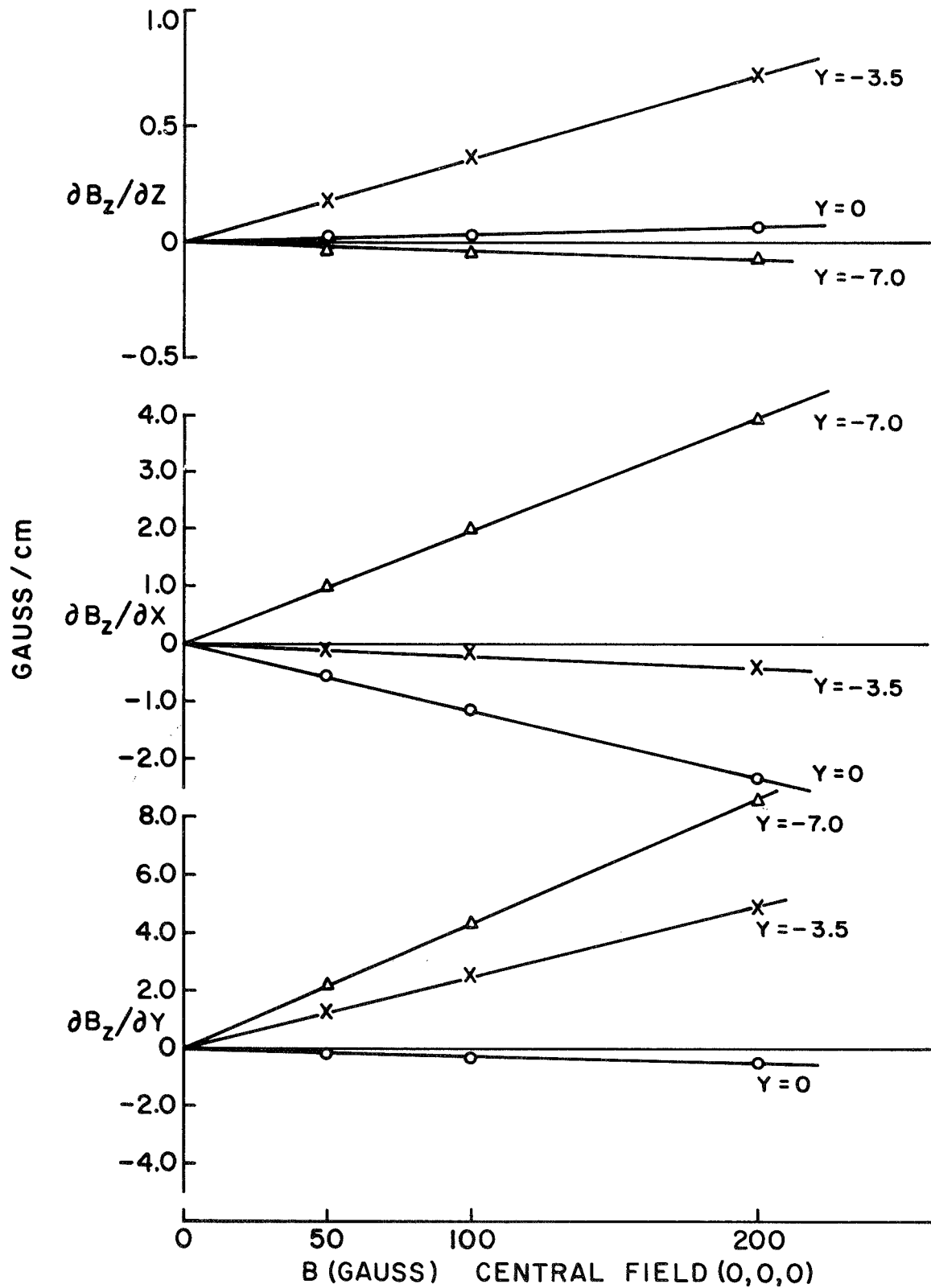
GRADIENT OF B_z VS RADIAL POSITION AND MAGNETIC FIELD FIGURE 9
