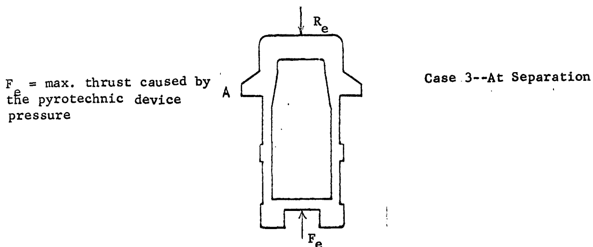
Force-Reaction Diagram
