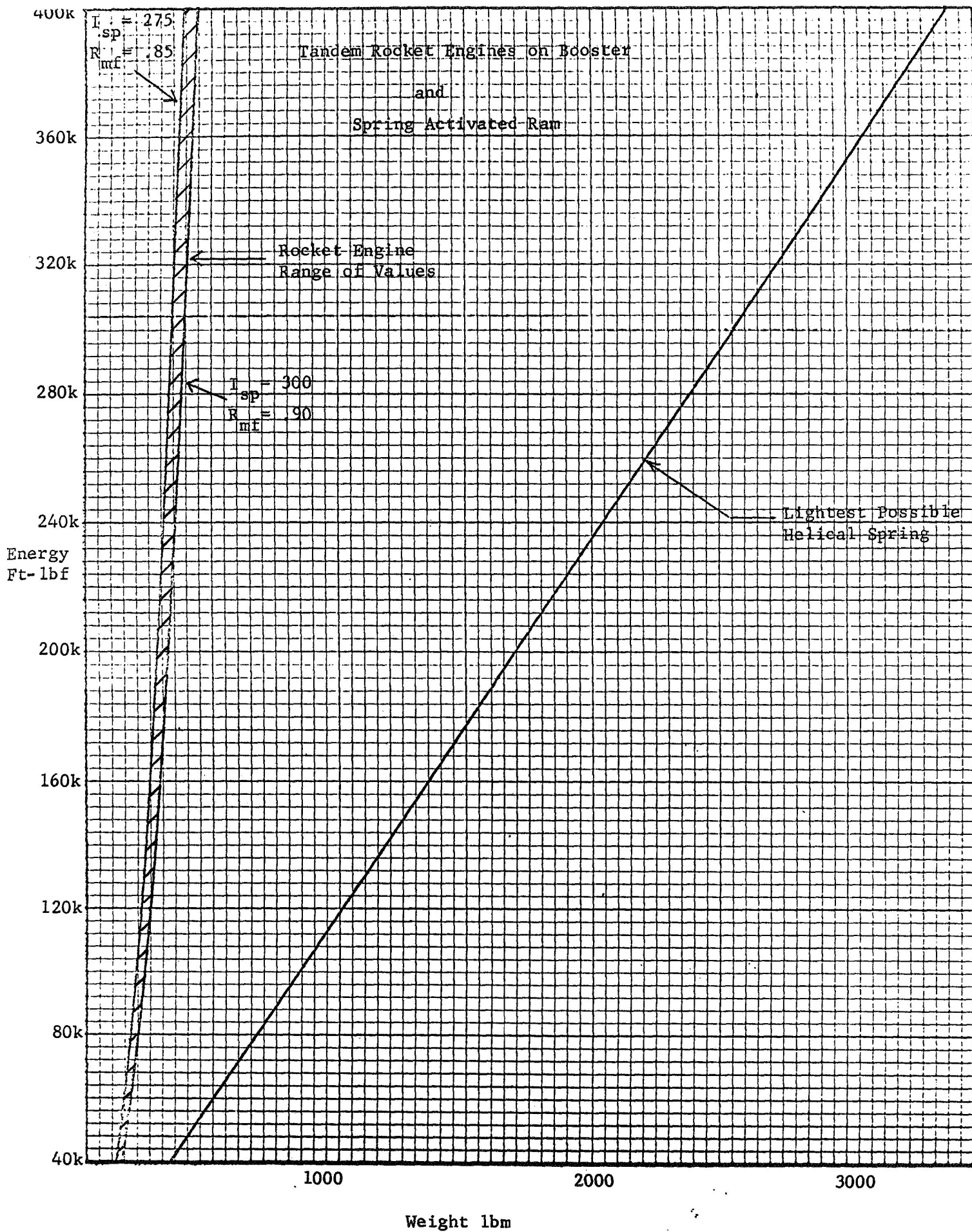
Figure (A-1) SEPARATION ENERGY VERSUS SYSTEM WEIGHT
