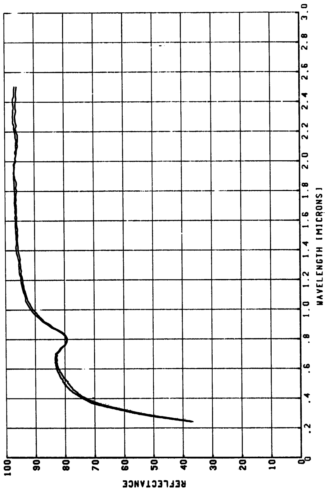
FIGURE 54. IN AIR/IN VACUUM REFLECTANCE PROPERTIES OF NASA-GODDARD ALUMINIZED 10-MIL TEFLON (TA-10)
