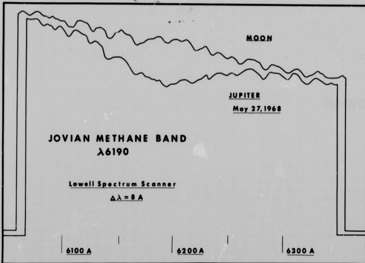
Fig. 1. A spectrum scan of the center of the Jovian disk shown normalized to the standard moon scan. The regions \lambda\lambda 6045-6120\text{\AA} and \lambda\lambda 6285-6360\text{\AA} were used to determine normalizing factors.
