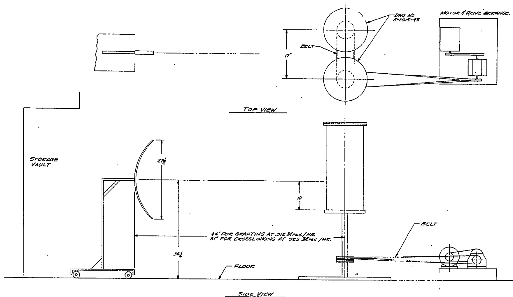
FIGURE 2. IRRADIATION CONFIGURATION
