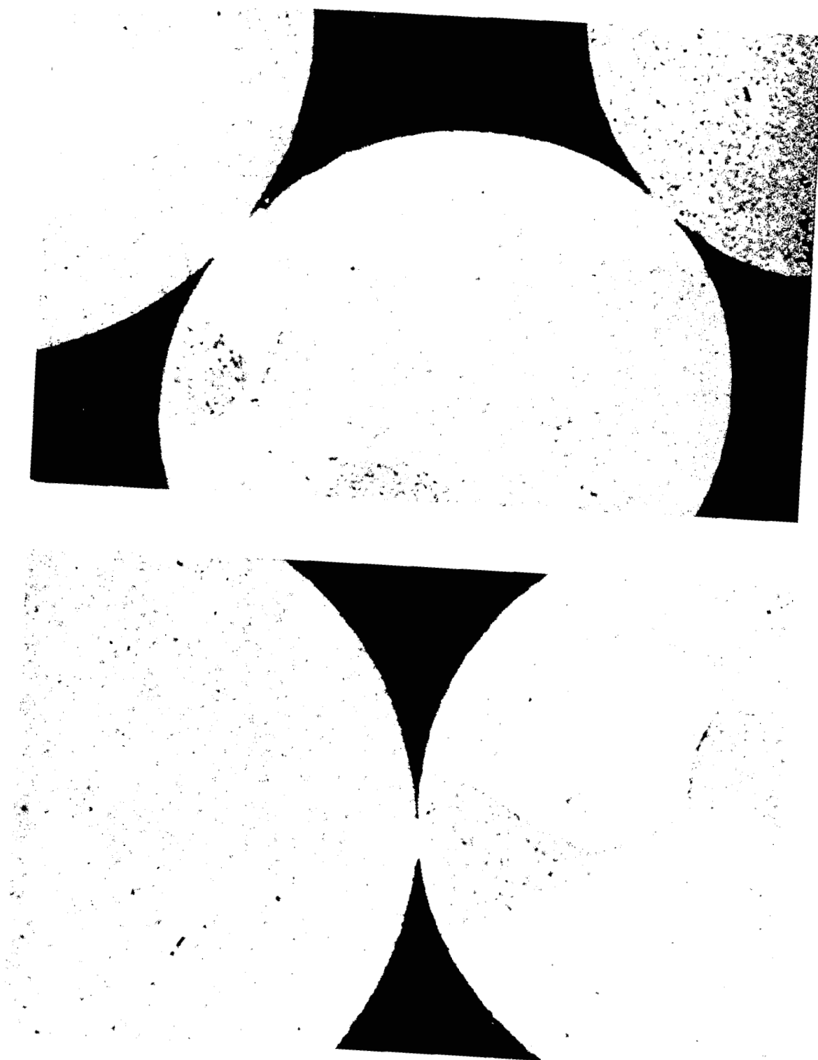
Fig. 55 Evidence for Interconnection of Silver Spheres After Electrode Operation. 3000×
