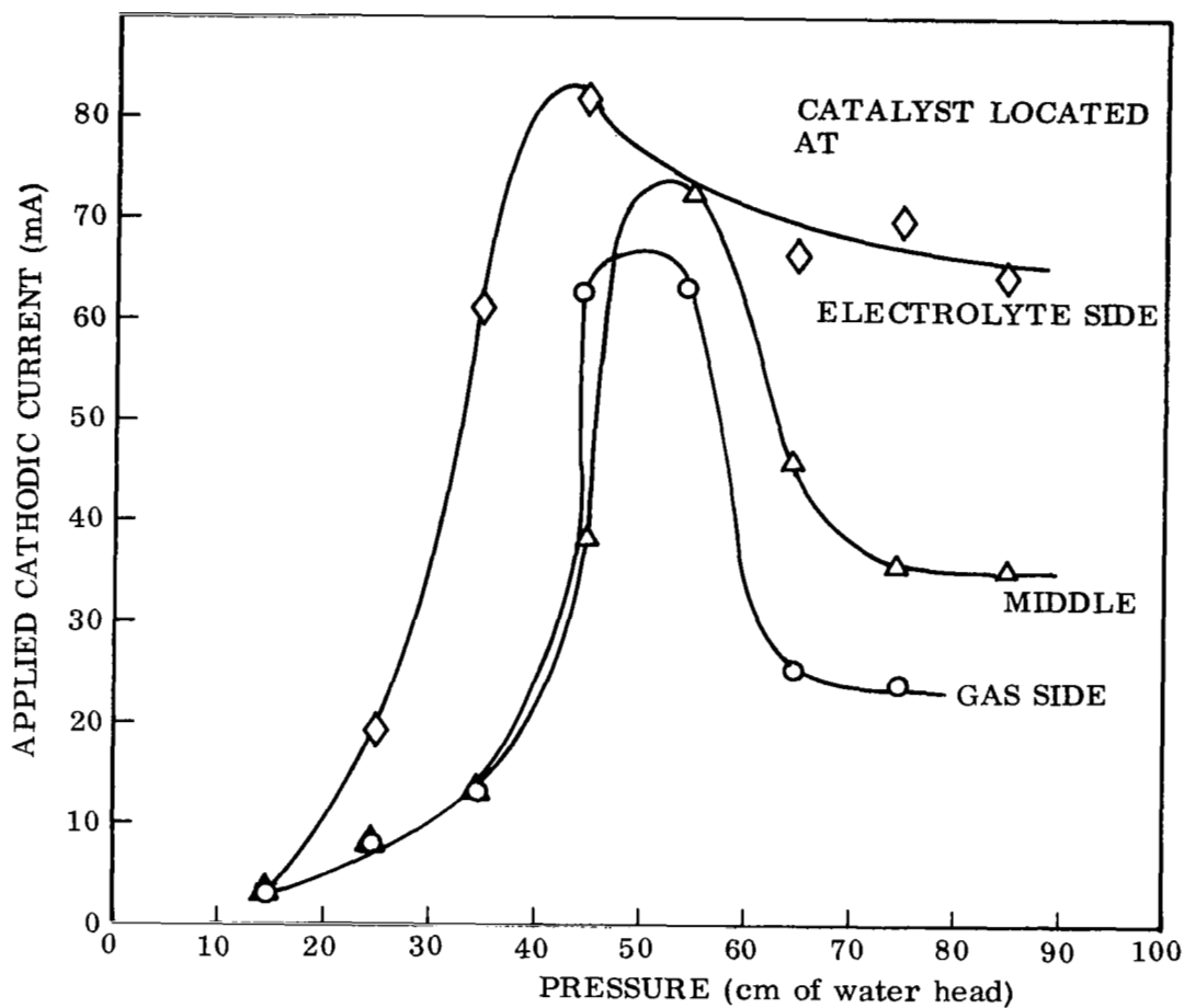
Fig. 45 Comparison of Performances With Three Types of Catalyst Distribution at 500 mV Versus Hydrogen Reference in Same Solution. Silver oxygen electrodes are compared with small amount of platinum catalyst at gas side, middle, and electrolyte side of coarse layer
