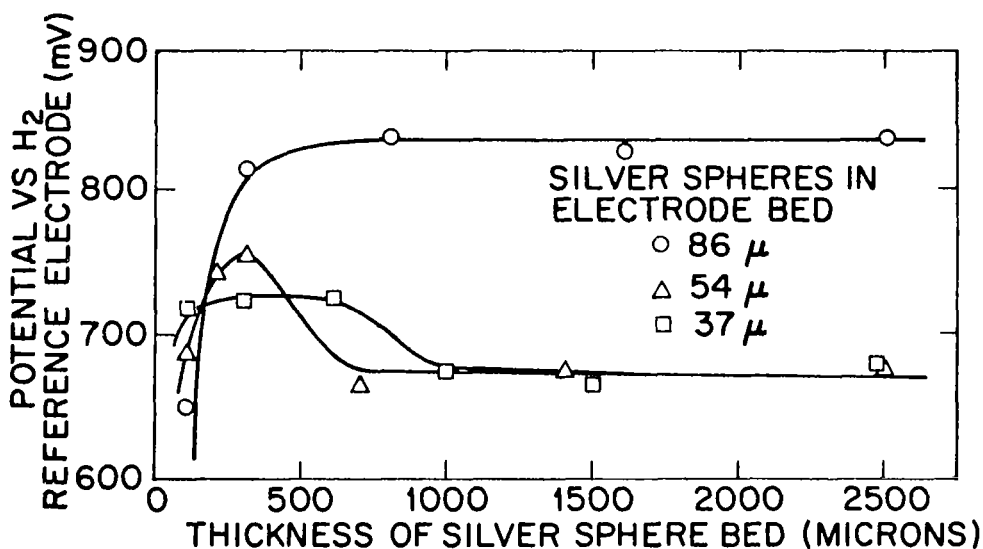
Fig. 31 Effect of Electrode Thickness on Electrode Potential for Various Sphere Sizes. Oxygen Differential Pressure, 25 cm of Water; Cathodic Current Density, 4.2\ \text{mA cm}^{-2}
