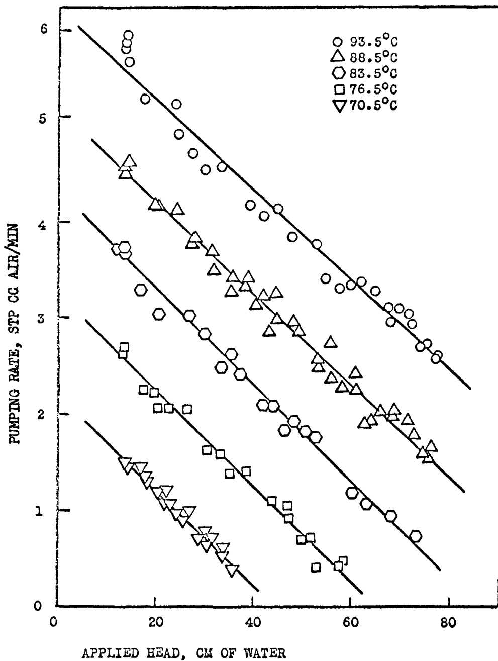
Fig. 71 Effect of Applied Head on Pumping Rate (Air-Water System; Flow-by Rate, 43.0 STP cc/min; 1.17 cm 2 Area; Microporous Teflon Membrane; 263 \mu Thick)
