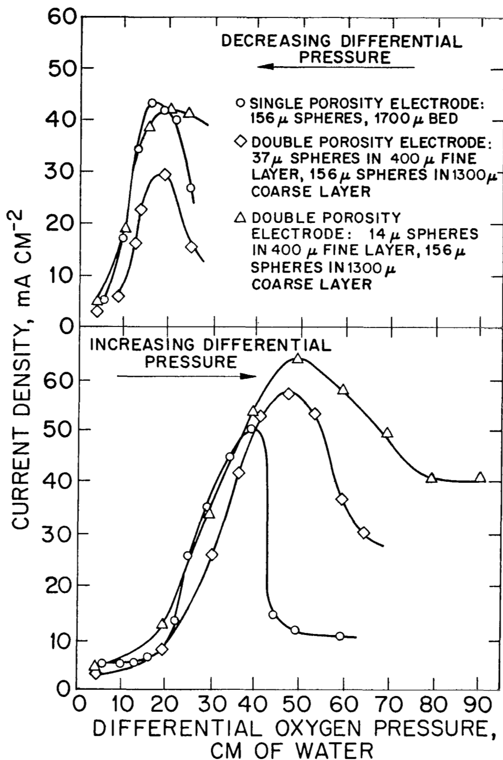
Fig. 36 Comparison of Single- and Double-Porosity Electrodes as Differential Pressure Is Changed. Silver Sphere Beds With Total Thickness at 1700 \mu at Potential of 500 mV Versus Hydrogen Reference Electrode
