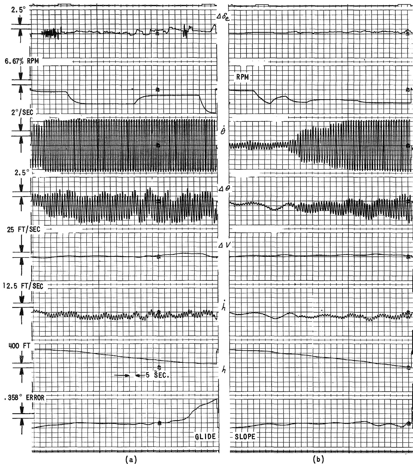
Figure 8a LONGITUDINAL DATA - \zeta_{sp} = 0 , \omega_{sp} = 3.0 - FIRST PRACTICE RUN
