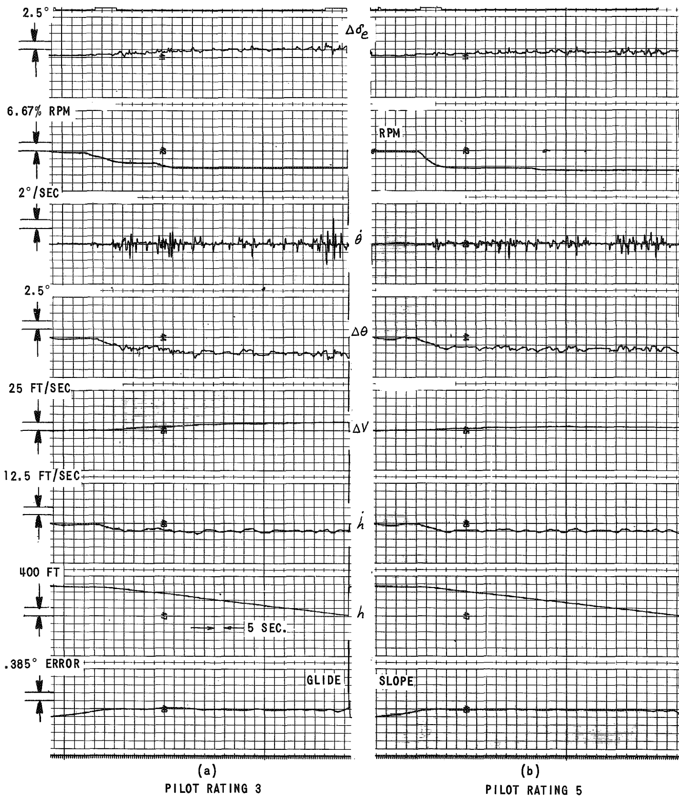
Figure 11a LONGITUDINAL DATA - \zeta_{sp} = 0.6 , \omega_{sp} = 6.0
