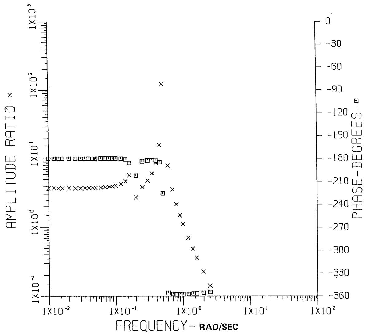
Figure 14 \alpha/\text{Se} BODE PLOT
