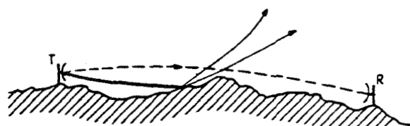
(d) Effect of insufficient ground clearance and upward bending of the rays
