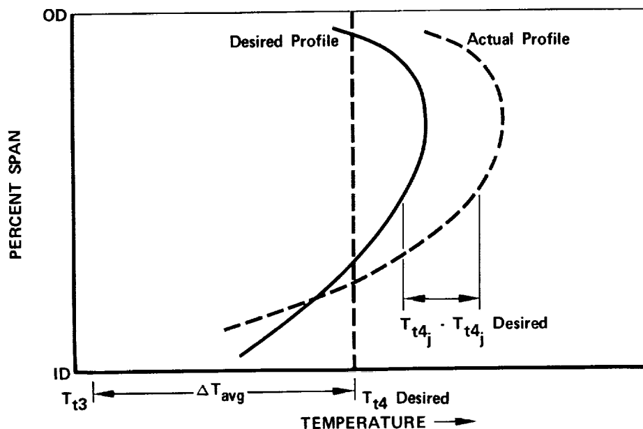
Figure 4. Explanation of Terms in \delta_{\text{rotor}} Expression
