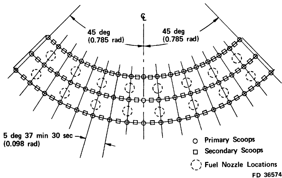
Figure 21. Opposed Scoop Pattern, Model 7 Combustor
