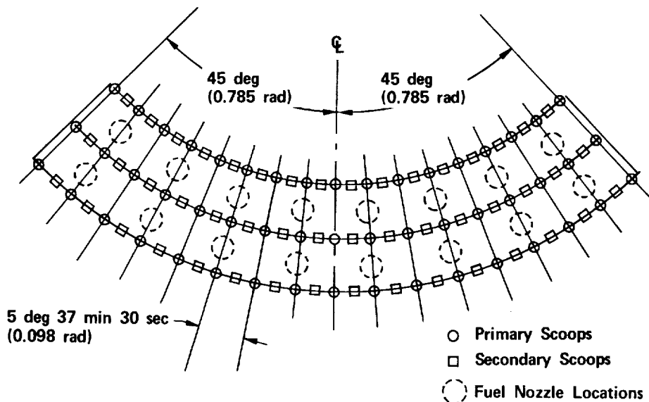
Figure 49. Opposed Scoop Pattern, Model 7 Combustor
