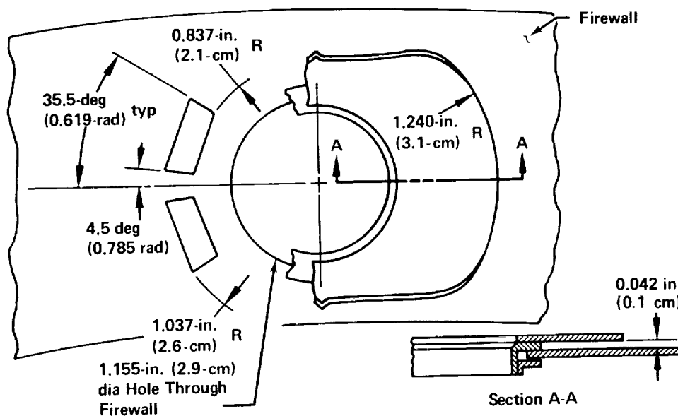
Figure 33. Final Firewall Cooling Deflector Design
