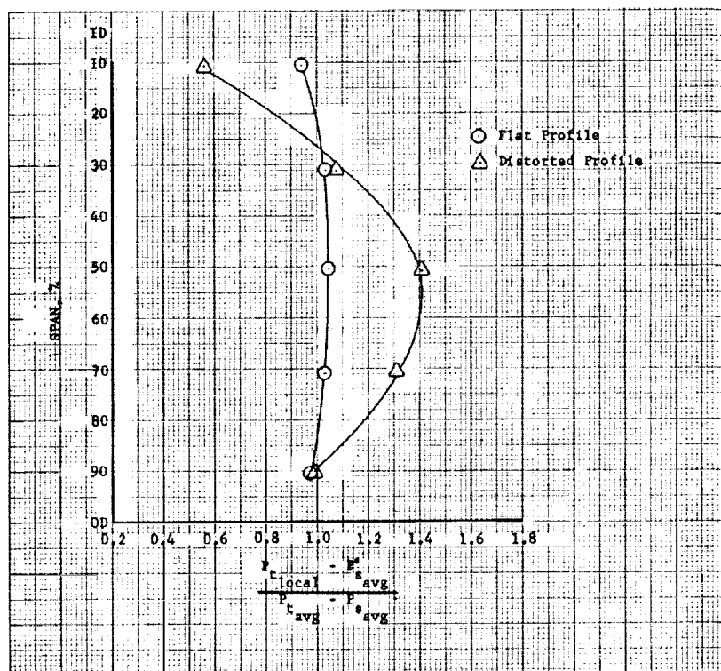
Figure 6. Typical Diffuser Inlet Velocity Head Profiles
