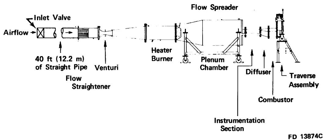
Figure 55. Double-Annular Combustor Test Rig
