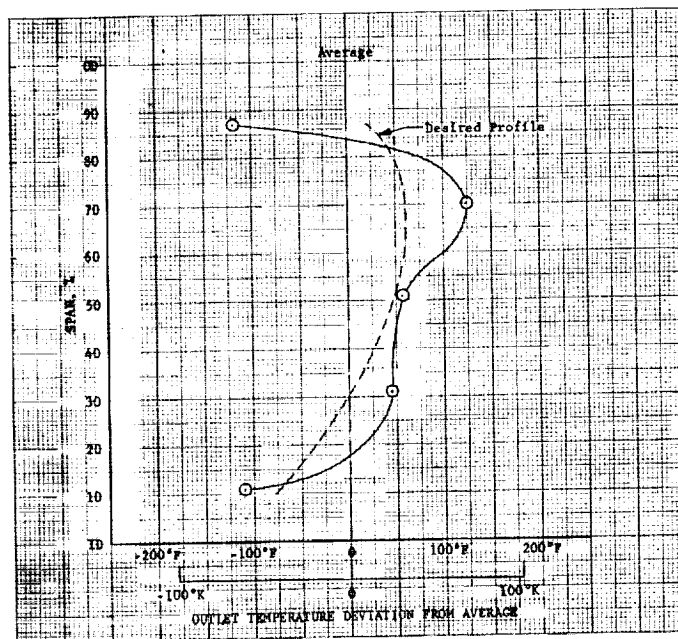
Figure 22. Outlet Radial Temperature Profile, Model 7 Combustor
