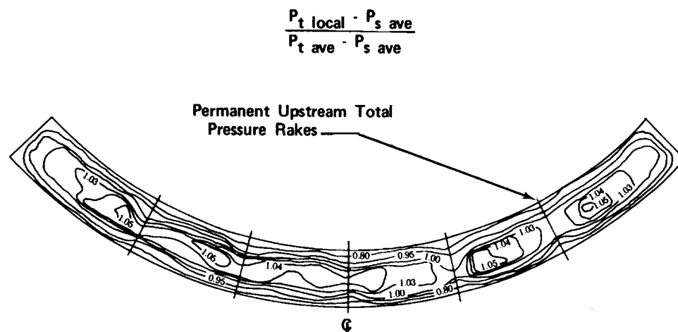
Figure 58. Velocity Head Contour Map, Instrumentation Section Exit
