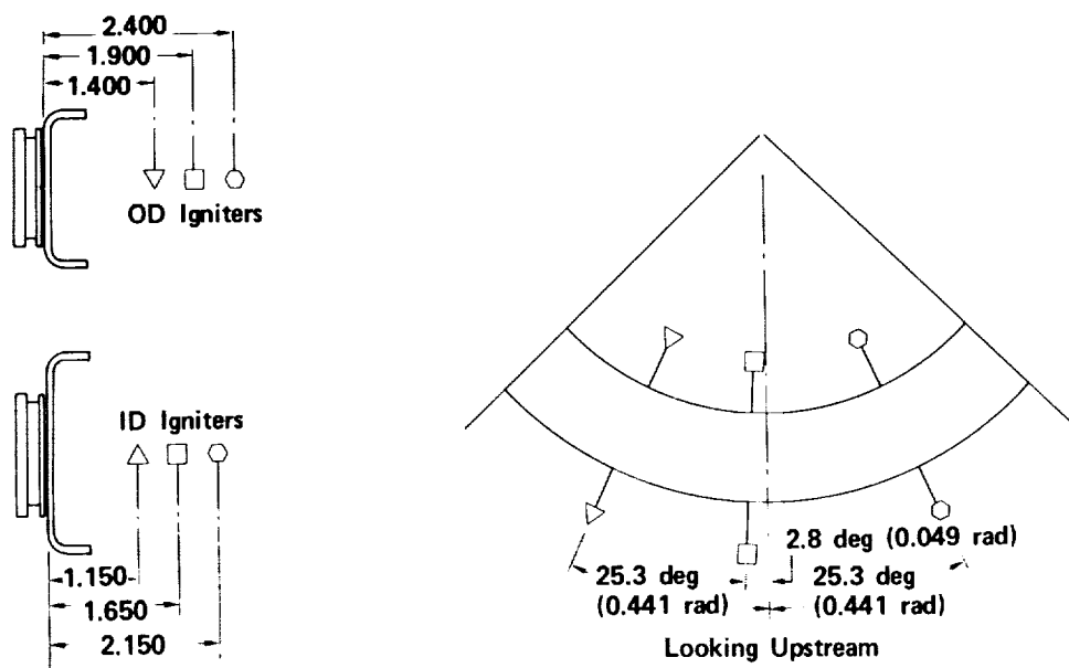
Figure 27. Igniter Positions
