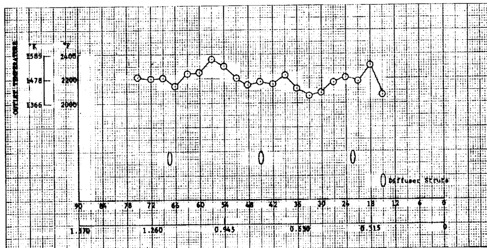
Figure 24b. Outlet Circumferential Temperature Profile, Model 1 Combustor Installed in 14-Degree ECA, Splitter Type Diffuser
