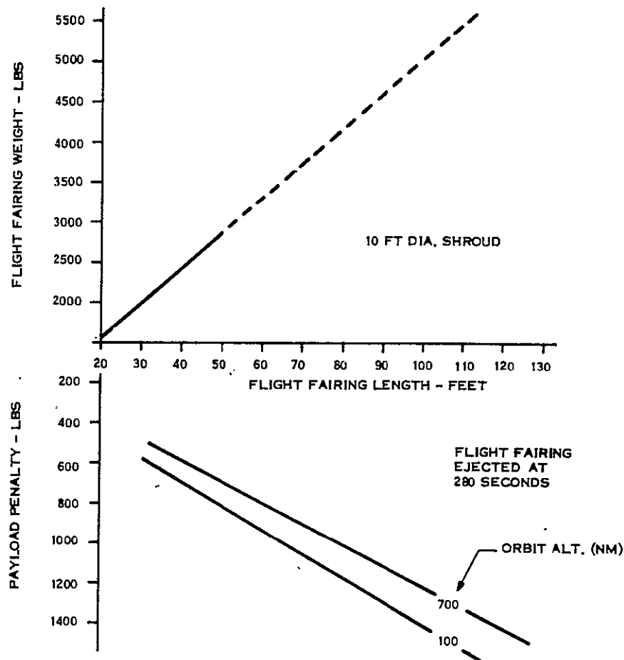
Figure 4-1. Flight Fairing Weight and Payload Penalty (Titan IIC/7)
