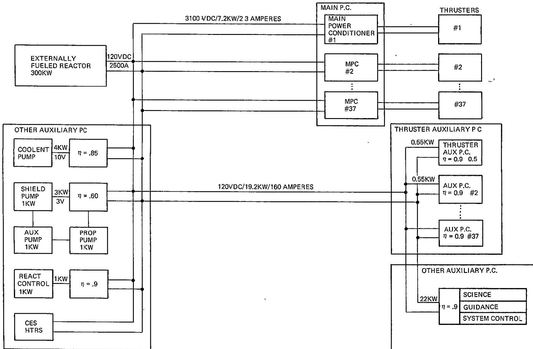
Figure 6-10. Externally Fueled Reactor Electrical Power System
