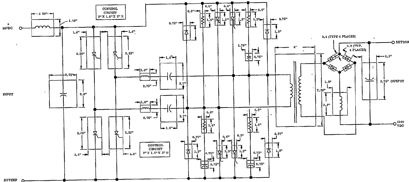
Figure 6-12. Component Geometry, Externally Fueled Reactor Main Power Conditioner
