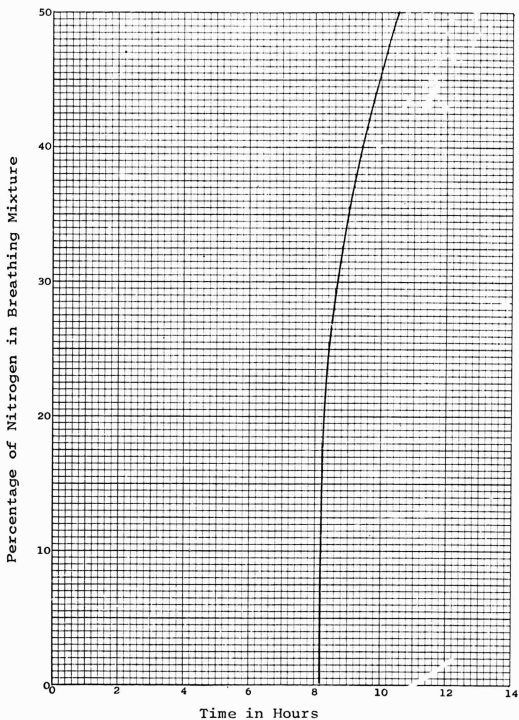
Figure 6. Denitrogenation time considered safe before decompressing from 5.6 psia to 3.5 psia (including 3\frac{1}{4} hours of denitrogenation by breathing oxygen).
