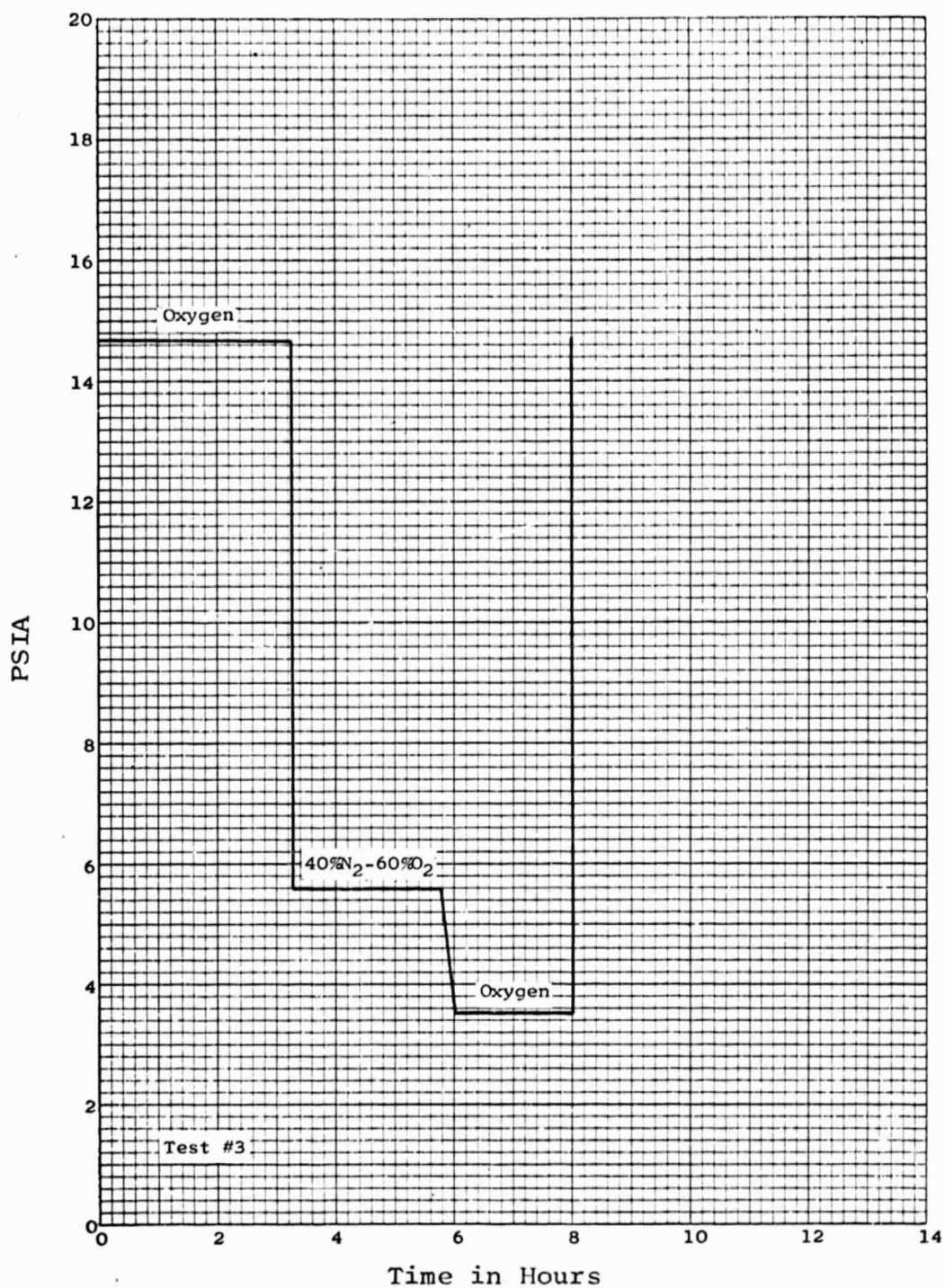
Figure 8. A profile of a pressure exposure which includes a 3\frac{1}{4} hour preoxygenation period at surface pressure.
