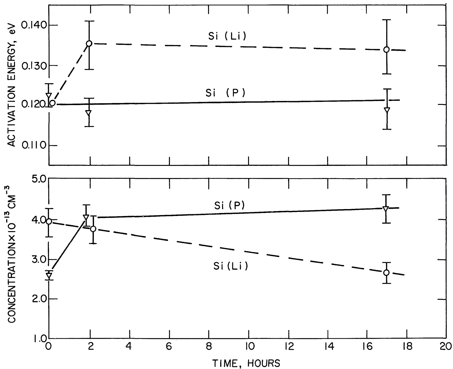
Fig. 8 - Effect of mobile lithium upon a radiation-induced level at E_c - .12 \text{ eV} .
