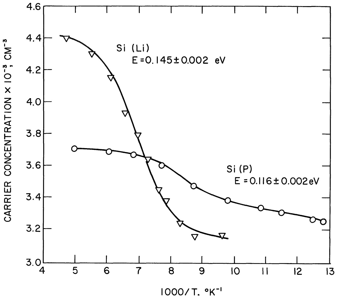
Fig. 5 - Radiation-induced intermediate level structure and least squares best fits for lithium and phosphorus-doped silicon
