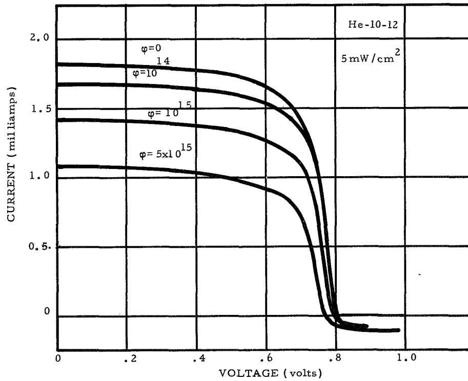
Fig. 15 - Current - voltage characteristics for a representative cell as a function of 1 MeV electron fluence. The cell was irradiated at 125°K and measured at 90°K under solar simulator illumination of (a) 100 mw/cm 2 , and (b) 5 mw/cm 2 .
