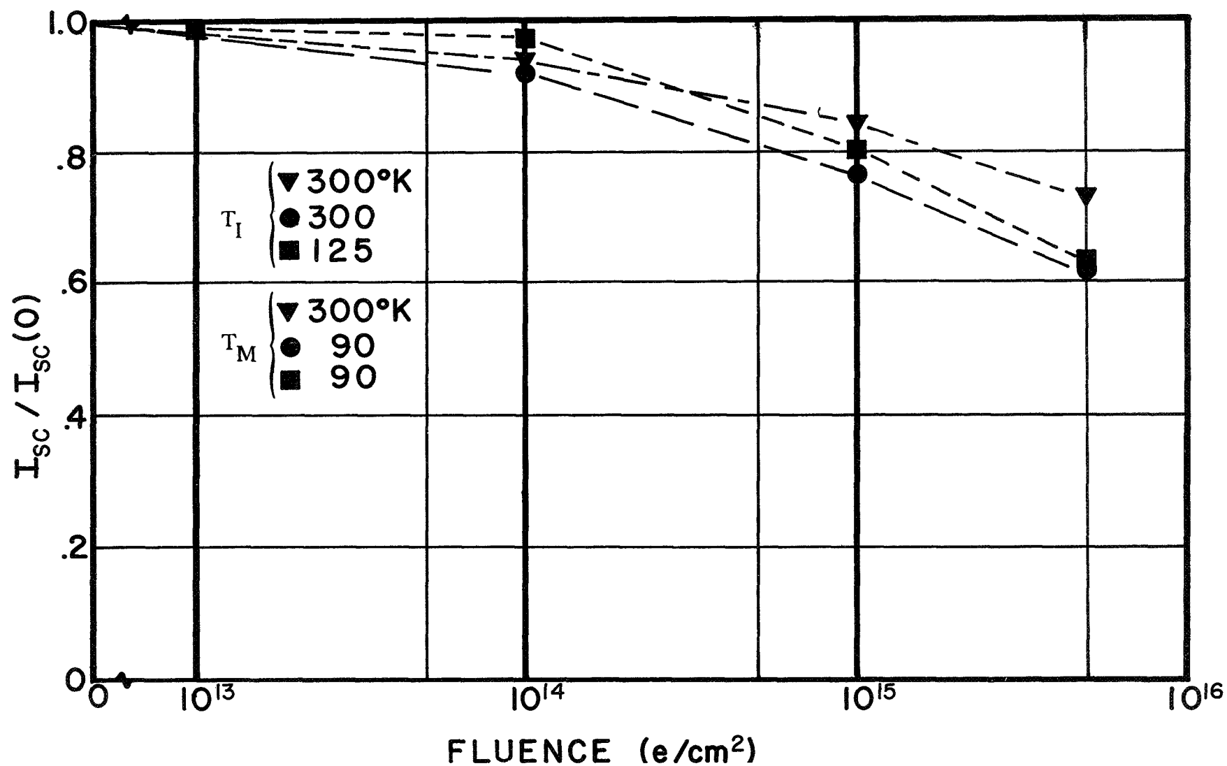
Fig. 18 - Normalized short-circuit current as a function of 1 MeV electron fluence for various irradiation and measurement temperatures.
