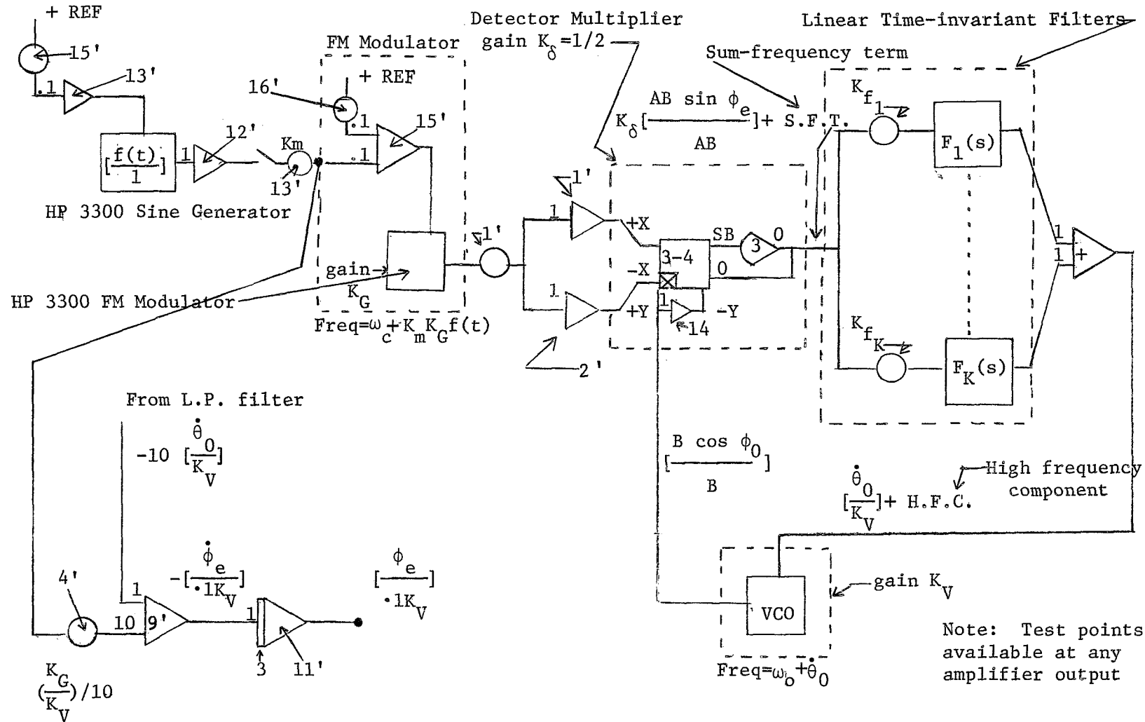
Figure 10a. M-PLL Carrier Model Analog Computer Configuration
