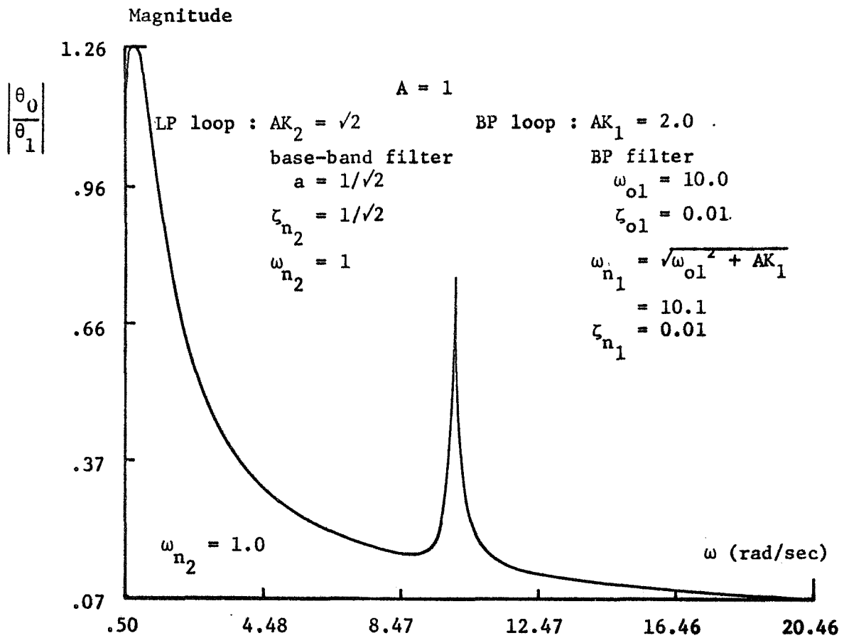
Figure 16a. L-BP M-PLL Phase Magnitude Response for the Linear Approximation
