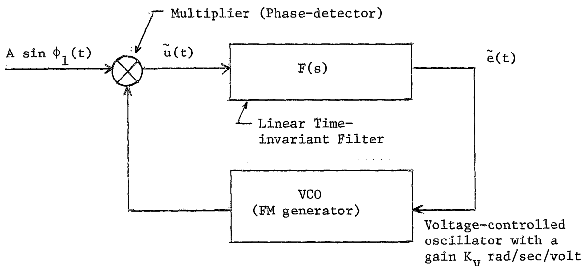
Figure 3. System Diagram for a PLL
