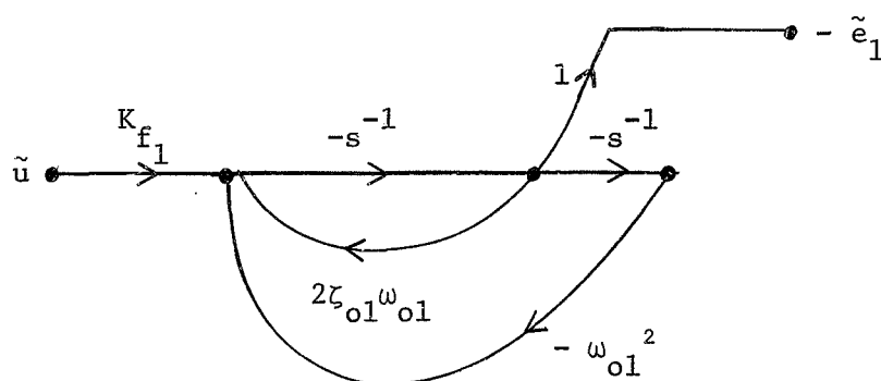
Figure 13 . Signal Flow Graph for K_{f1}s/(s^2 + 2\zeta_{o1}\omega_{o1}s + \omega_{o1}^2)
