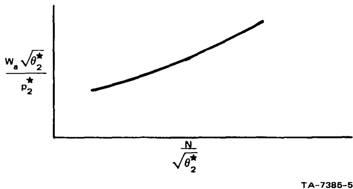
FIGURE 7 AIRFLOW AS A FUNCTION OF ROTOR SPEED
