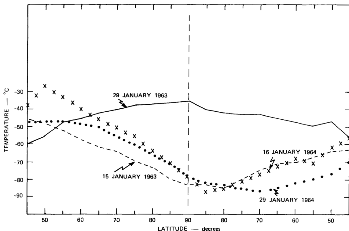
FIGURE 22 COMPARISON OF TEMPERATURE DIFFERENCES AT 30 mbs DURING SELECTED DAYS IN JANUARY, 1963 AND 1964, FOR 5^\circ INCREMENTS NORTH OF LATITUDE 45^\circ\text{N} ALONG THE 0^\circ - 180^\circ MERIDIAN THROUGH THE NORTH POLE
