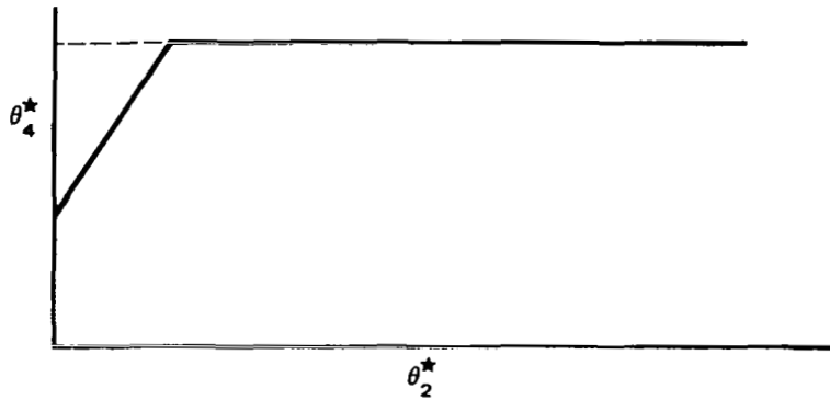
FIGURE 9 TYPICAL TOTAL TEMPERATURE INCREASE DUE TO COMPRESSOR AND COMBUSTOR
