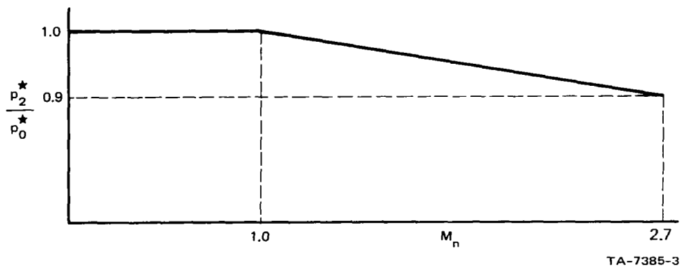
FIGURE 5 RAM RECOVERY
