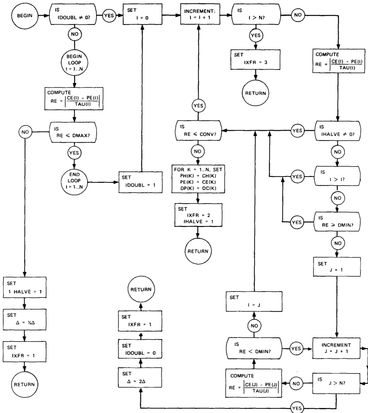
FIGURE 31 FLOW CHART FOR SUBROUTINE CHKCONV, N, DELTA, DMIN, DMAX, CONV
