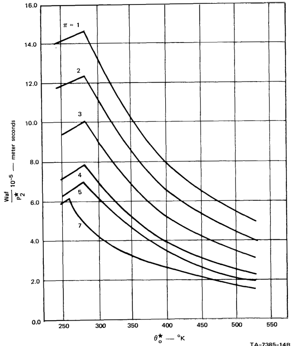
FIGURE 16 FUEL FLOW AS A FUNCTION OF \theta_o^*
