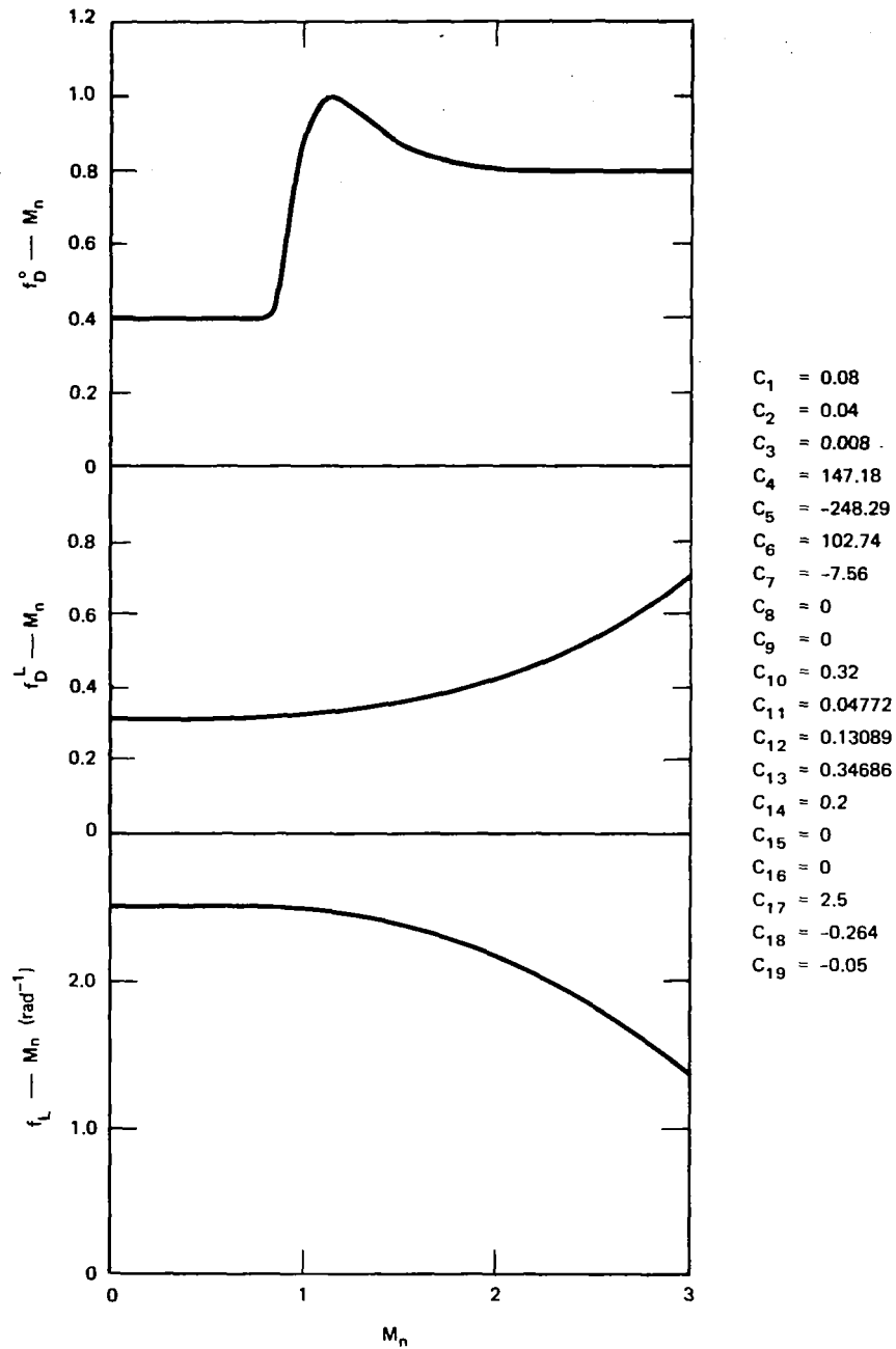
FIGURE 28 TYPICAL AERODYNAMICS
