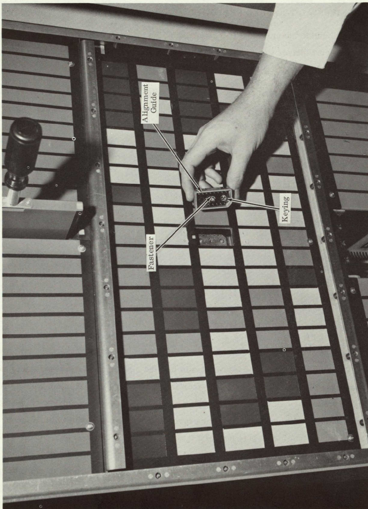
Figure 8-10. Module #10 Installation
